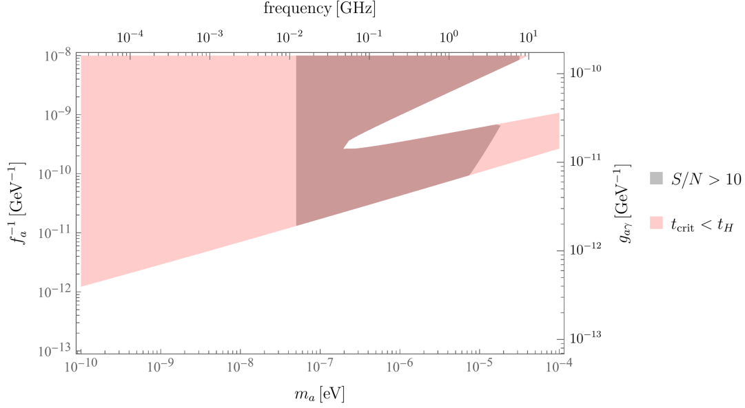
FIG. 2. Axion parameters that lead to axinovae in the current universe using the self-similar growth in Ref. [27]. The pink region represents the axion parameter space that leads to axion star collapse and the gray region corresponds to radio emissions with S/N > 10 . Note that the result is very similar to that in Fig. 1 even though we have used a different formula for axion star growth.
