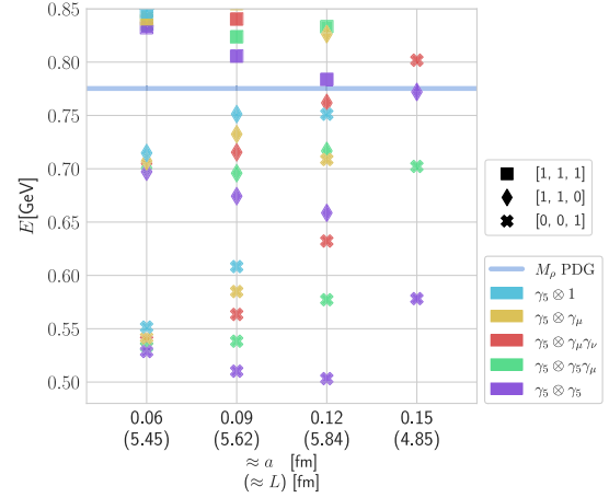
FIG. 1. Continuum, noninteracting energy spectrum for \pi_\xi \pi_\xi \rightarrow \rho case on four physical-mass HISQ ensembles for the relevant tastes, \xi . The ensembles' parameters are given in Ref. [21]. The tastes of the single pions in the two-pion state are indicated by the color. The back-to-back momentum is indicated by the symbol shape. Also given is the \rho^0 Particle Data Group mass (blue band) [50] which is used as the cutoff energy to select the operator basis.
