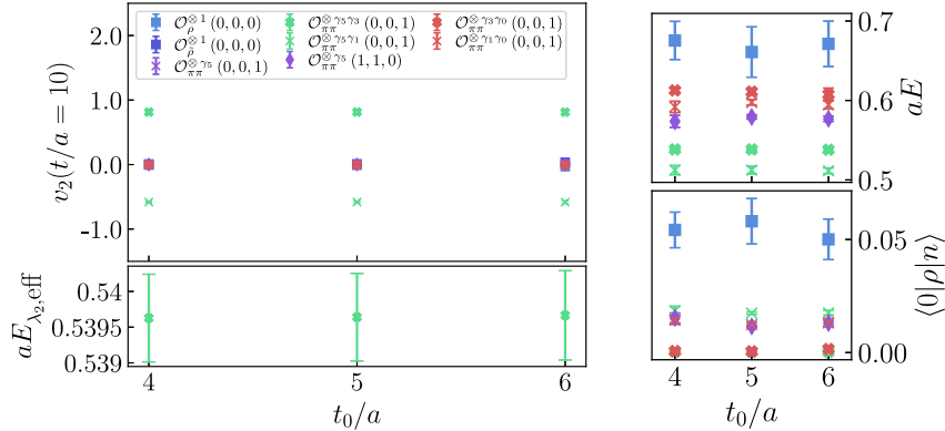
FIG. 7. Left: normalized eigenvector for the n = 2 state as function of t_0 (top). The eigenvector is selected at t'/a = 10 . The corresponding energy (bottom) is obtained by applying the effective mass formula, Eq. (3.30), to the eigenvalue and performing a correlated average over the data points t/a > 10 . Right: full GEVP spectrum comparison, energies (top) and amplitudes (bottom) for the same three choices of t_0 . See legend of Fig. 6 for state labels. The ground-state energy is omitted to improve the visibility of the rest of the spectrum, as the gap to the first excited state is large (see Fig. 6).
