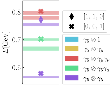
FIG. 5. Comparison of the free continuum spectrum of Fig. 1 (symbols) with the interacting spectrum of Fig. 4 (bands).
