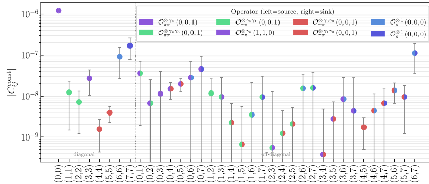
FIG. 15. All constants obtained from the MEM fit, Eq. (G1). On the left side of the figure we show the diagonal constants including the \rho two-point functions. On the right side we show the off-diagonal constants.
