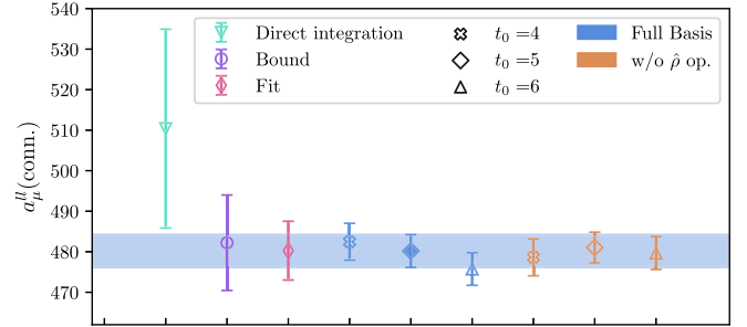
FIG. 11. Results for a_{\mu}^{II}(\text{conn}) from the reconstruction strategy described in this work, using the 9600 configuration vector-current dataset. We show results for the variations discussed in Sec. IV A 1, choosing different values of t_0 and also dropping the \rho^0 operator before performing the GEVP. Our final choice of a_{\mu}^{II}(\text{conn}) is given by the full operator basis at t_0/a = 5 , indicated by the blue band and filled symbol. Also included are comparisons to a_{\mu}^{II}(\text{conn}) from the different noise-reduction strategies discussed in Sec. II, a_{\mu}(\text{fit}) and a_{\mu}(\text{bound}) , as well as a_{\mu}(\text{direct}) , the result obtained by direct integration of the data with no noise-reduction applied.
