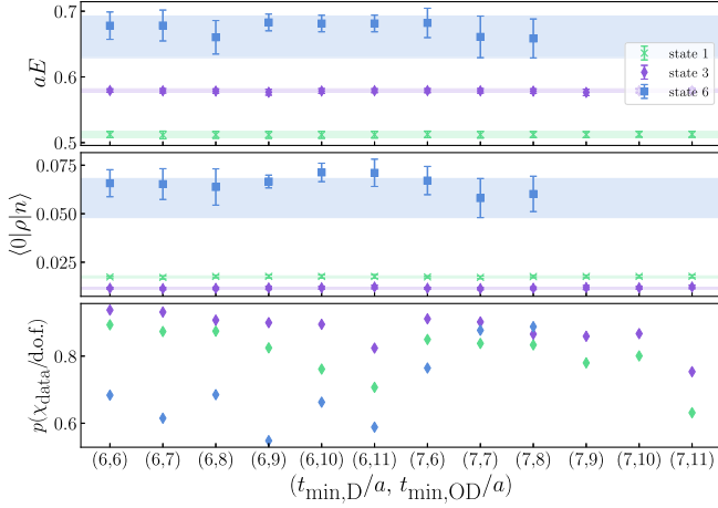
FIG. 8. Stability of fit results with respect to t_{\min,D}/a and t_{\min,OD}/a for the n = [1, 3, 6] states. All fits contain 2 + 1 exponentials and t_{\max,D}/a and t_{\max,OD}/a are fixed to 18 and 20 which corresponds to the maximum available time slice for t_{\max,D}/a . Bands represent the fits from the preferred values listed in Table V. Top: ground-state energy. Middle: overlap amplitude. Bottom: quality of fit as measured by the p value, excluding the prior contribution.
