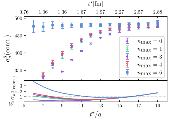
FIG. 10. Top: results for a_{\mu}^{II}(\text{conn}) as t^* , the point at which the correlator is replaced by the reconstruction, is varied. Bottom: relative error in the determinations of a_{\mu}^{II}(\text{conn}) from the top figure.
