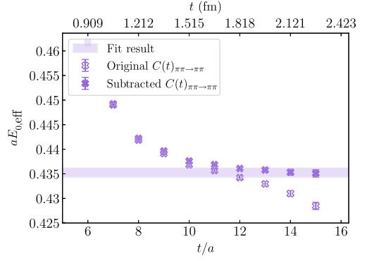
FIG. 2. Effective mass of the correlation function C(t)_{\pi\pi\rightarrow\pi\pi} : \langle \mathcal{O}_{\pi\pi}^{\otimes\gamma_s}(\vec{0}, t) \mathcal{O}_{\pi\pi}^{\otimes\gamma_s}(\vec{0}, 0) \rangle uncorrected (empty) and corrected (filled) purple crosses for the wraparound contribution using the method described in this section. Also shown is the result of a fit to corrected correlation function.
