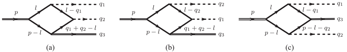
FIG. 3. Kinematics used for calculating four-point integrals.
