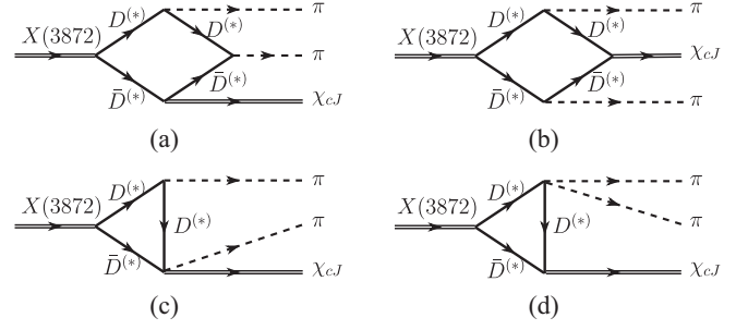
FIG. 1. Box [(a), (b)] and triangle [(c), (d)] diagrams contributing to the dipionic transitions from X(3872) to \chi_{cJ} .
