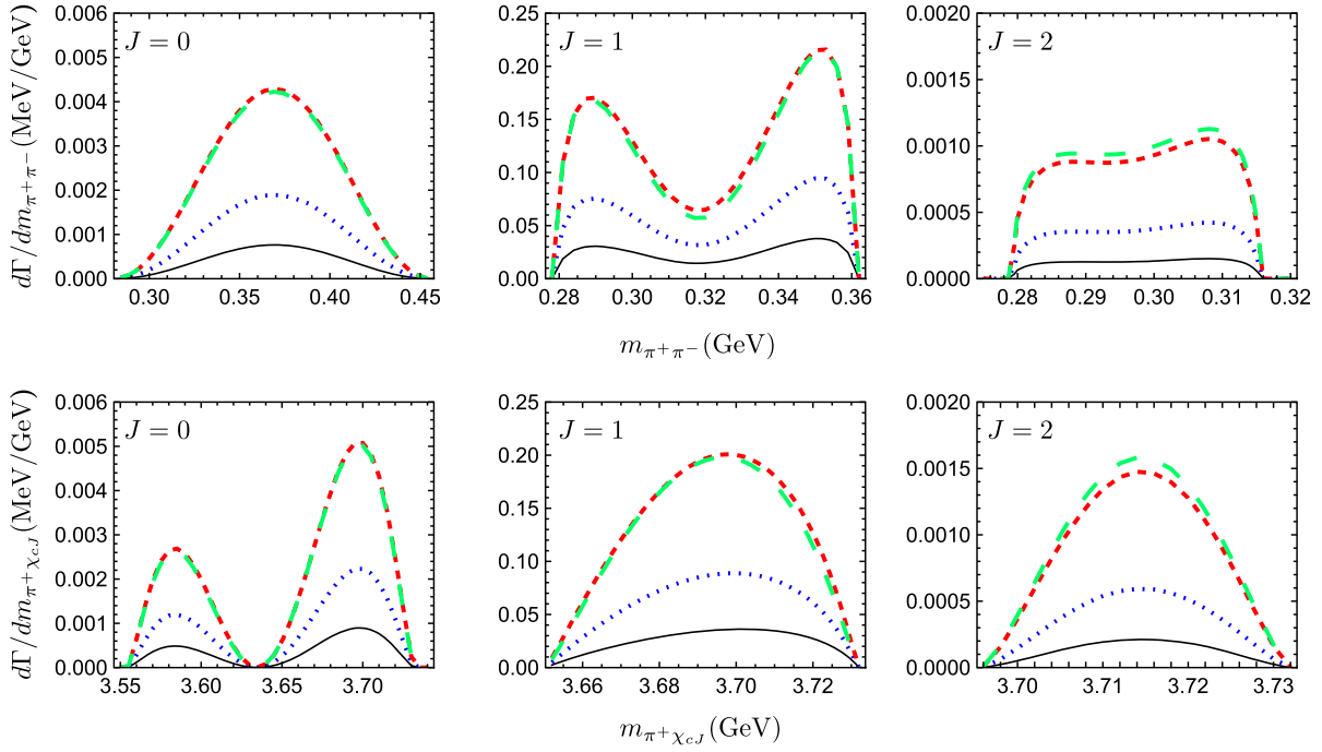
FIG. 2. Invariant mass distributions of \pi^+\pi^- and \pi^+\chi_{cJ} for the decays of X(3872) \rightarrow \pi^+\pi^-\chi_{cJ} ( J = 0, 1, 2 ). The black, blue, red, and green lines correspond to \theta = 0, \pi/12, \pi/4 , and \pi/2 , respectively.
