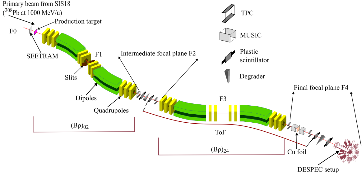
FIG. 1. Schematic layout of the FRS showing its focal planes F0–F4. The production target was located at F0; F1 and F3 were under vacuum; F2 was dispersive and F4 achromatic. Single particle detectors were placed in air gaps at F2 and F4, and the DESPEC setup was situated at F4. (B\rho)_{02} and (B\rho)_{24} are the magnetic rigidity of the separator in each section.
