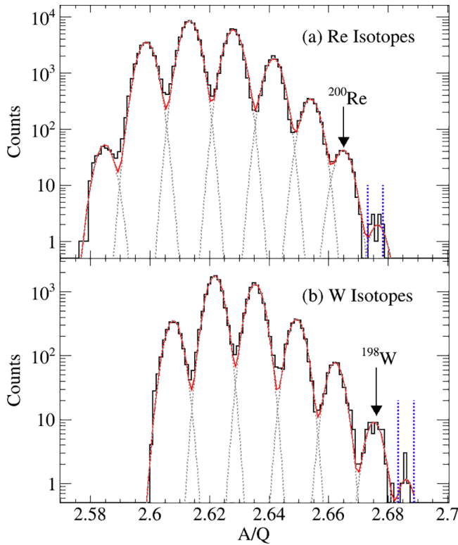
FIG. 4. A/Q spectra for (a) rhenium isotopes and (b) tungsten isotopes produced in the ^{202}\text{Os} setting. One isotope is labeled with an arrow for reference. The A/Q spectra were fitted with a sum of Gaussian distributions. In addition to the fit, the number of counts of the two peaks with smallest statistics was obtained by counting within the region indicated by blue dashed lines; for details see text.
