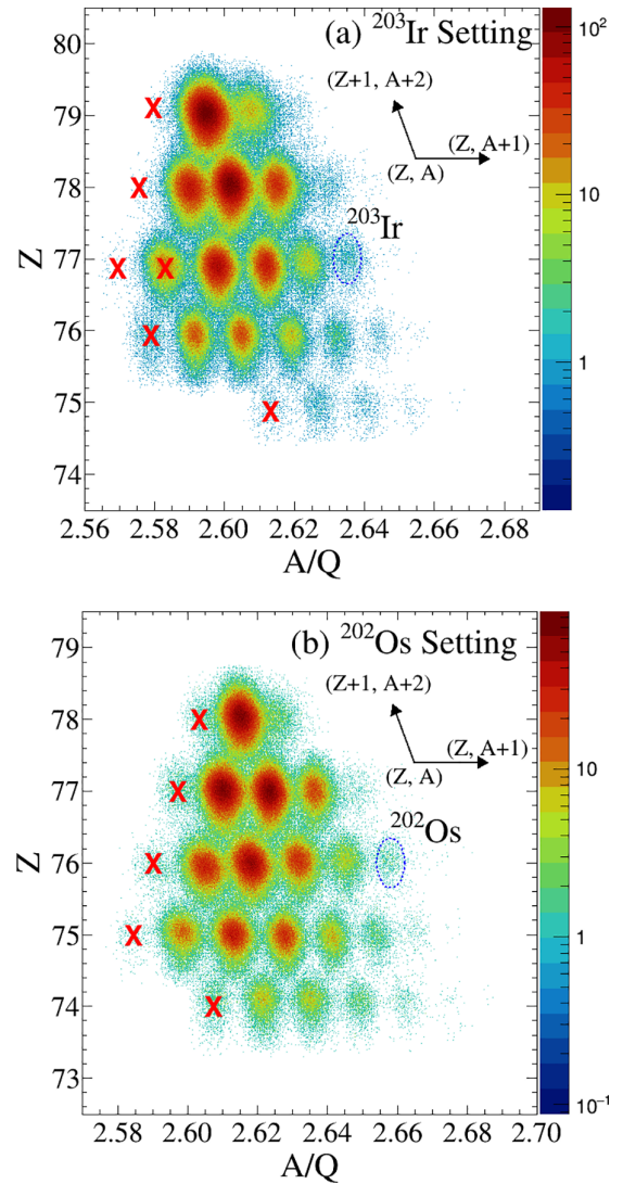
FIG. 3. Particle identification (PID) plot of the ions which were fully ionised in both stages of the separator, i.e., for which Q = Z . The plot shows the atomic number Z versus the A/Q ratio for (a) the ^{203}\text{Ir} setting and (b) the ^{202}\text{Os} setting. For clarity, the centered isotope is highlighted and labeled with its mass number. The arrows show the relations of atomic and mass numbers of the nuclides. The red crosses indicate those nuclides, for which ion-optical transmission was determined to be less than 10% and their production cross sections were not evaluated from this setting; for details see Sec. II B 3.
