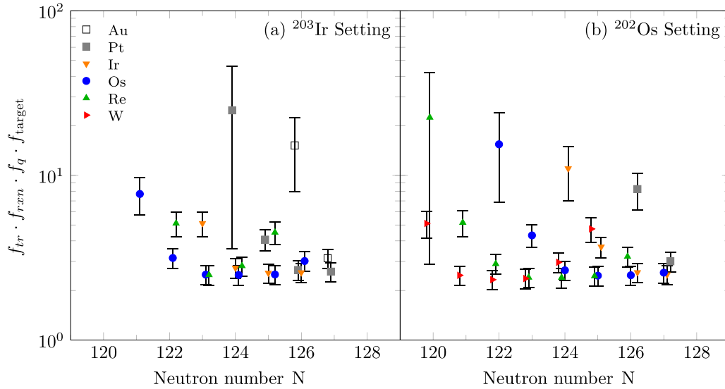
FIG. 5. Combined correction factor ( f_{tr} \cdot f_q \cdot f_{rxn} \cdot f_{target} ) as a function of neutron number for (a) ^{203}\text{Ir} setting and (b) ^{202}\text{Os} setting, note the log scale. The time-dependent factors f_{DAQ} and f_{det} are not shown here. See Secs. II B 2–II B 6 for details.
