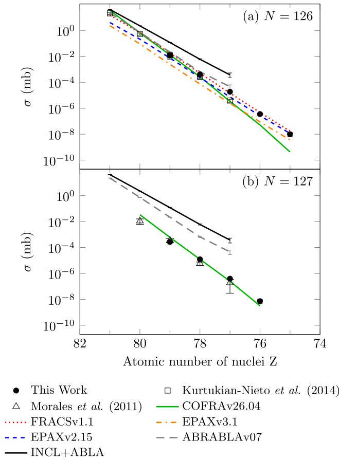
FIG. 7. (a) Production cross sections for the N = 126 isotones via proton removals, measured in the reaction 1000 \text{ MeV/u } ^{208}\text{Pb} + ^9\text{Be} (filled black circles). The data are compared with literature Kurtukian-Nieto et al. [35] obtained for the same collision system and energy (open black square). The lines show predictions of various models: COFRAv26.04 calculation (solid green line) [22,38], FRACsv1.1 parametrization (red dotted line) [41], EPAXv3.1 parametrization (orange dash-dotted line) [34], EPAXv2.15 parametrization (blue dashed line) [36], ABRABLA07 (gray long dashed line) [37], and INCL + ABLA (black double dot dashed line) [39,40]. (b) Production cross sections of N = 127 isotones in charge-exchange reactions: 1000 \text{ MeV/u } ^{208}\text{Pb} + ^9\text{Be} (filled black circles; this work), 1000 \text{ MeV/u } ^{208}\text{Pb} + ^9\text{Be} (open black triangle) from Morales et al. [31]. Line styles correspond to the same models as in panel (a). If the error bars of the experimental data are not visible, they are smaller than the marker size.
