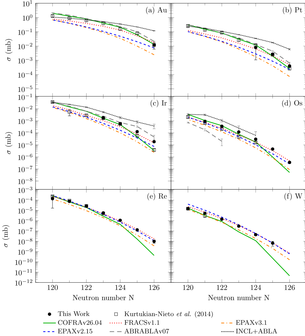
FIG. 6. Measured production cross sections of fragment residues from element Z = 79 to Z = 74 produced in the reaction 1000 \text{ MeV/u } ^{208}\text{Pb} + ^9\text{Be} (filled black circles). Data from Kurtukian-Nieto et al. [35] obtained for the same reaction are also shown (open black squares). If the error bars of the experimental data are not visible, they are smaller than the marker size. The lines show predictions of various models: COFRAv26.04 calculation (solid green line) [22,38], FRACsv1.1 parametrization (red dotted line) [41], EPAXv3.1 parametrization (orange dashdotted line) [34], EPAXv2.15 parametrization (blue dashed line) [36], ABRABLA07 (gray long dashed line) [37], and INCL + ABLA (black double dot dashed line) [39,40].
