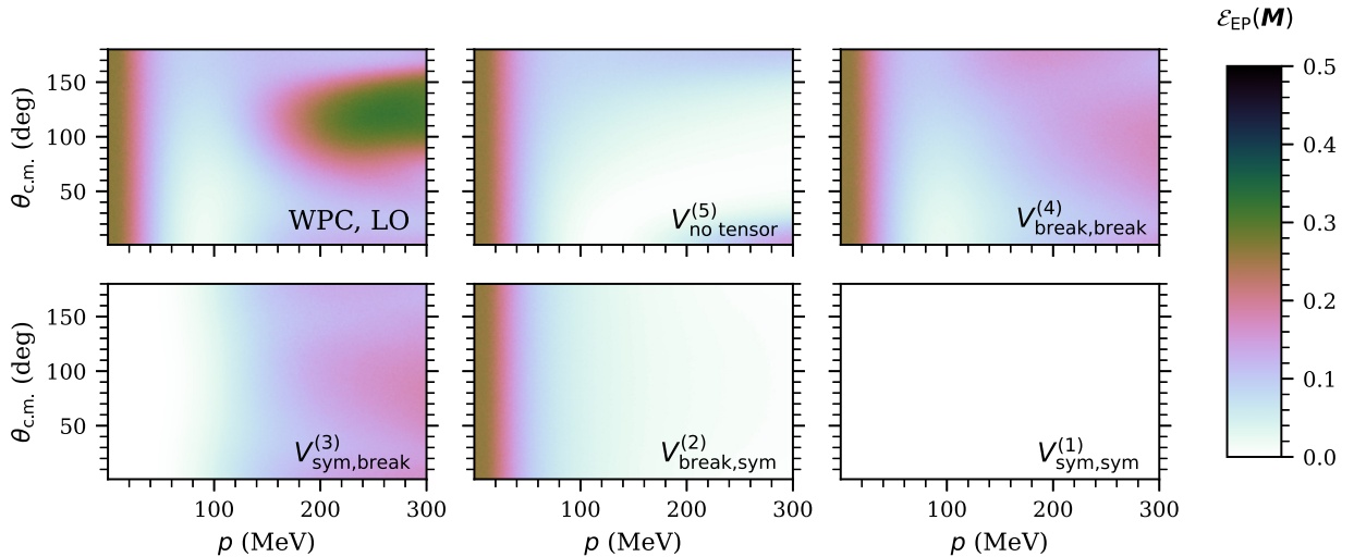
FIG. 2. Entanglement power of the M matrix \mathcal{E}_{\text{EP}}(M) for the np system using the LO WPC and the modified LO WPC potentials listed in Table I. Each LEC is tuned to a single S -wave phase shift, see Sec. II C, in all potentials (even the LO WPC potential). \mathcal{E}_{\text{EP}}(M) is evaluated for scattering angles \theta_{\text{c.m.}} \in [1^\circ, 180^\circ] and relative momenta p \in [0.01, 300] \text{ MeV} .
