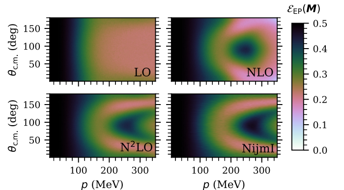
FIG. 4. Entanglement power of the M matrix \mathcal{E}_{\text{EP}}(\mathbf{M}) for the nn system using the WPC potential at different chiral orders. The lower right panel is the pp result using the NijmI potential [60] without the electromagnetic contribution. Due to charge symmetry, the nuclear pp and nn M matrices should be very similar. The LECs in the WPC potentials are from Ref. [62]. \mathcal{E}_{\text{EP}}(\mathbf{M}) is evaluated on the same angle-energy grid as in Fig. 3.
