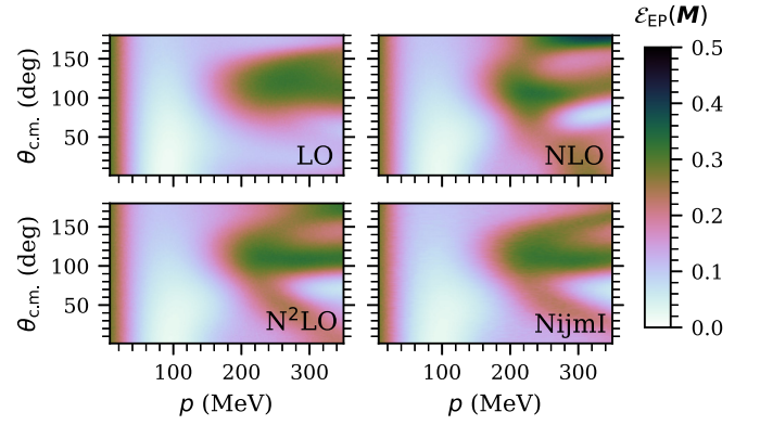
FIG. 3. Entanglement power of the M matrix \mathcal{E}_{\text{EP}}(\mathbf{M}) for the np system using the WPC potential at different chiral orders and using the phenomenological NijmI potential [60]. The LECs in the WPC potentials are from Ref. [62]. \mathcal{E}_{\text{EP}}(\mathbf{M}) is evaluated for scattering angles \theta_{\text{c.m.}} \in [1^\circ, 180^\circ] and relative momenta p \in [7, 350] MeV.
