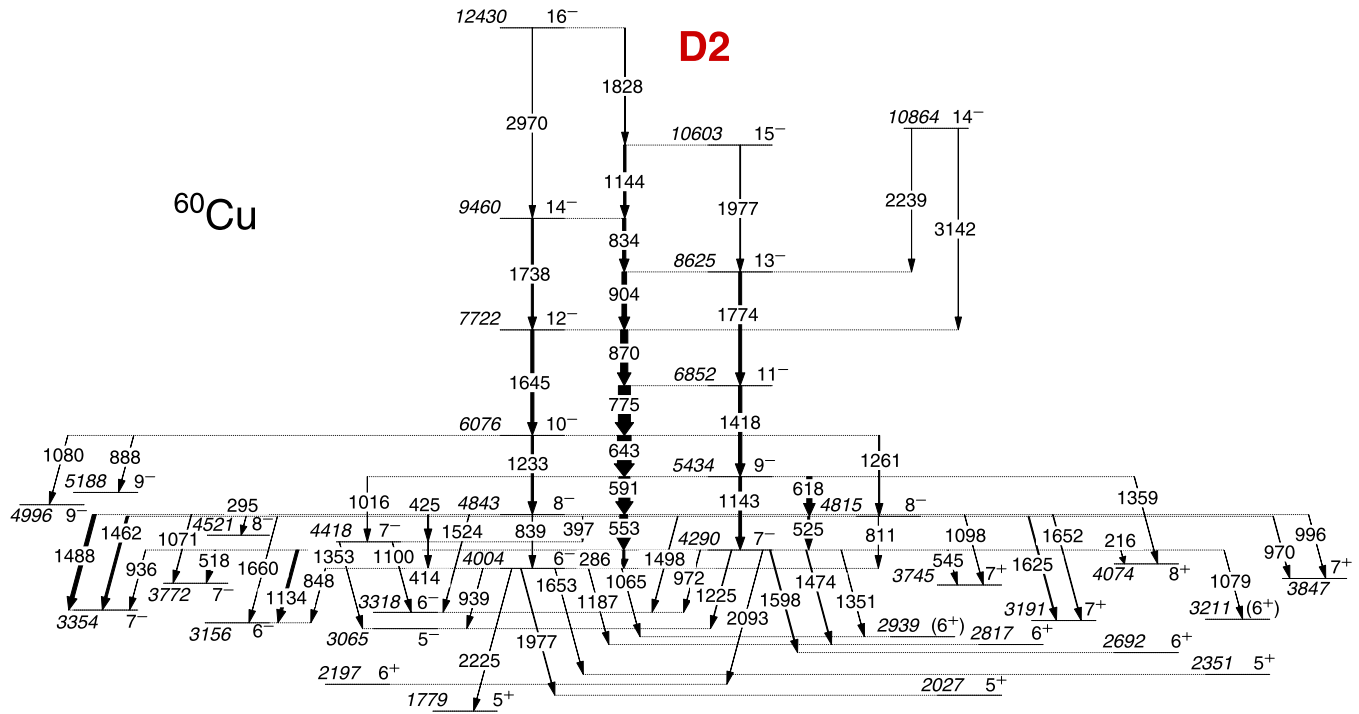
FIG. 4. Part of the level scheme of ^{60}\text{Cu} from the present study focusing on the dipole structure D2 (brick red) and its decay paths into the lower-lying structures (cf. Fig. 2). Energy labels are in keV. The widths of the arrows correspond to the relative intensities of the \gamma rays.
