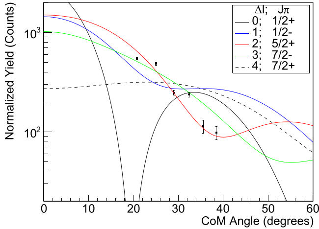
FIG. 10. Measured differential cross section for the 5822-keV energy level compared to different \ell -transfer predictions. The best fitting predictions are \ell = 2 and 3 .
