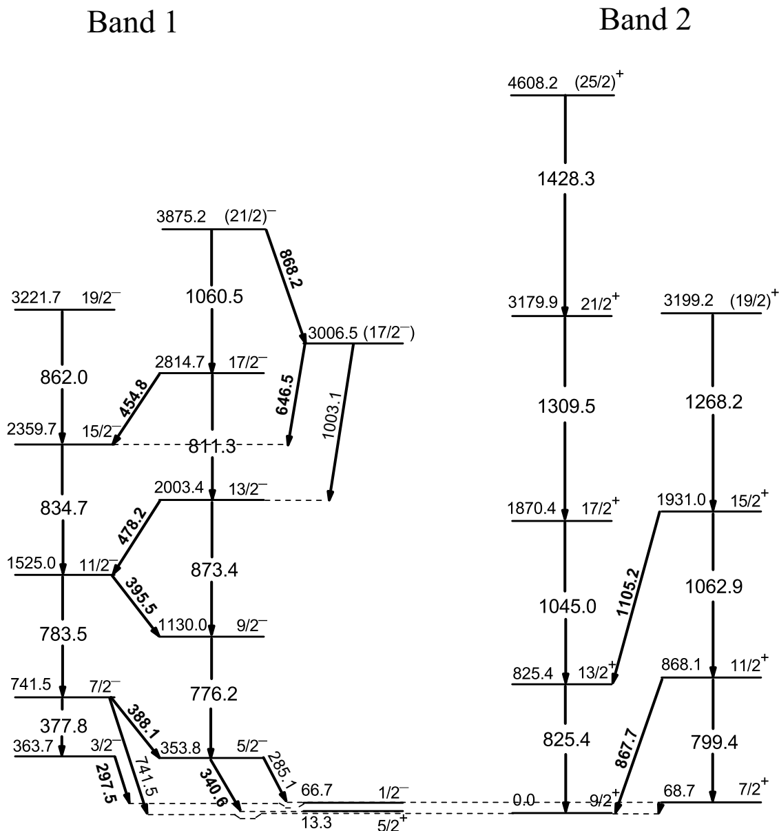
FIG. 1. Partial level scheme of ^{73}\text{Ge} . Energies are in keV. The energies that are updated in this Erratum are marked in bold.
