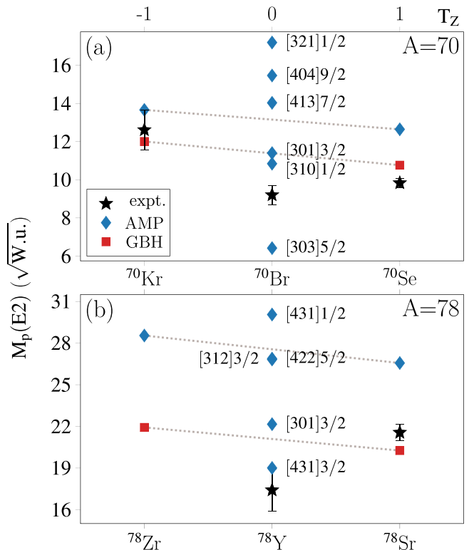
FIG. 6. The values of M_p(E2) computed with HFB + AMP using the UNEDF1 EDF for (a) A = 70 and (b) A = 78 isotriplets, compared with experimental data [6]. Different values for the T_z = 0 nuclei correspond to various 2-qp states near the Fermi level.
