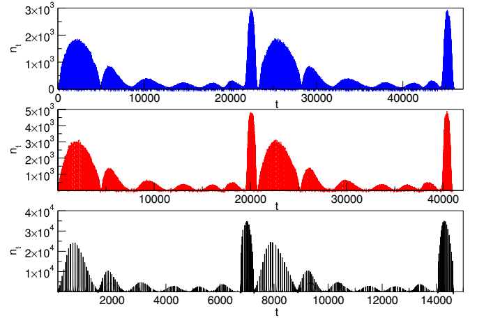
FIG. 2. The Barkhausen noise signal n_t vs time t recorded during the whole hysteresis loop for varied disorder f = 0.04, 0.3 , and 0.5 (bottom to top panel), exhibiting seven peaks along each branch, but with different scales and durations. From left to right, seven peaks correspond to the reversal of the system's segments comprising of spins with k = 0, 1, 2, \dots, 6 reversed nearest neighbor spins, leading to the magnetization steps along the ascending branch at the external field H_t^{ca} indicated in the Table I. Similarly, the following seven peaks are observed at these fields in the reversed order along the descending branch.
