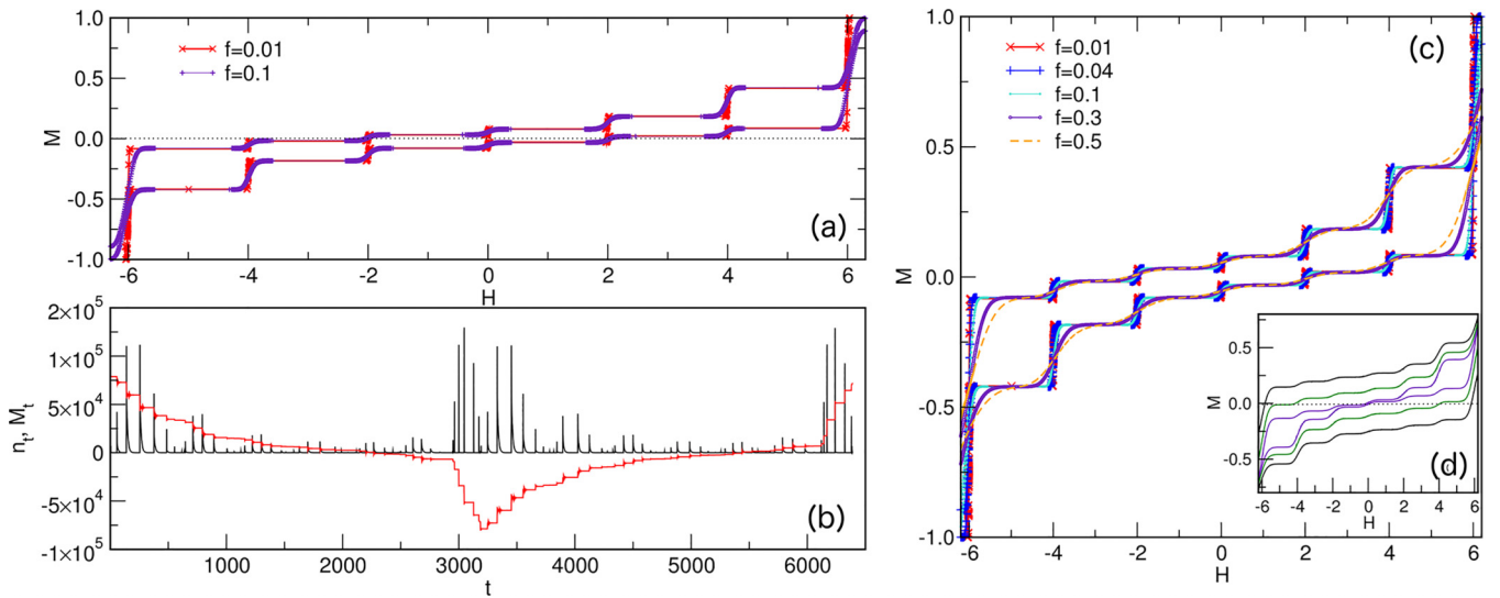
FIG. 1. (a) The hysteresis loop M vs H for the antiferromagnetic system with a weak random-field disorder f = 0.01 , showing the magnetization plateaus and the changing transition regions between them for slightly increased disorder f = 0.1 . (b) The appearance of magnetization bursts n_t for very low disorder f = 0.01 , and the magnetization evolution along the descending and ascending hysteresis branches M_t (normalized to fit the scale). (c) The hysteresis loops for different disorder f , indicated in the legend, and fixed probability p = 0.95 . The inset (d) shows how the hysteresis loop for fixed disorder f = 0.3 changes when p is varied from 0.995 (inner line), to 0.9 (middle line) and 0.8 (outer line).
