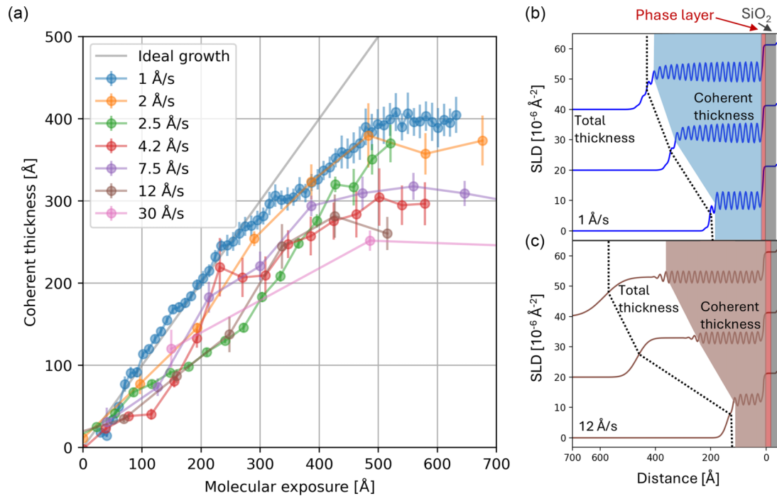
FIG. 4. Thickness of the coherently ordered fraction of the thin film as a function of the molecular exposure for all experiments. (a) Shows that the final coherently ordered film thickness is decreasing with higher growth rates. Moreover, the slope and therefore coherent growth speed is decreasing as well. (b) Three SLD profiles corresponding to slow growth rate of 1 Å/s with coherently ordered layer (colored area) and total thickness of the thin layer (dotted line). (c) SLD profiles for the fast growth rate of 12 Å/s reveal the amorphous layer (250 Å, dotted) on top of the coherently ordered layer (270 Å, colored) at the end of the growth (SLD offset for visualization).
