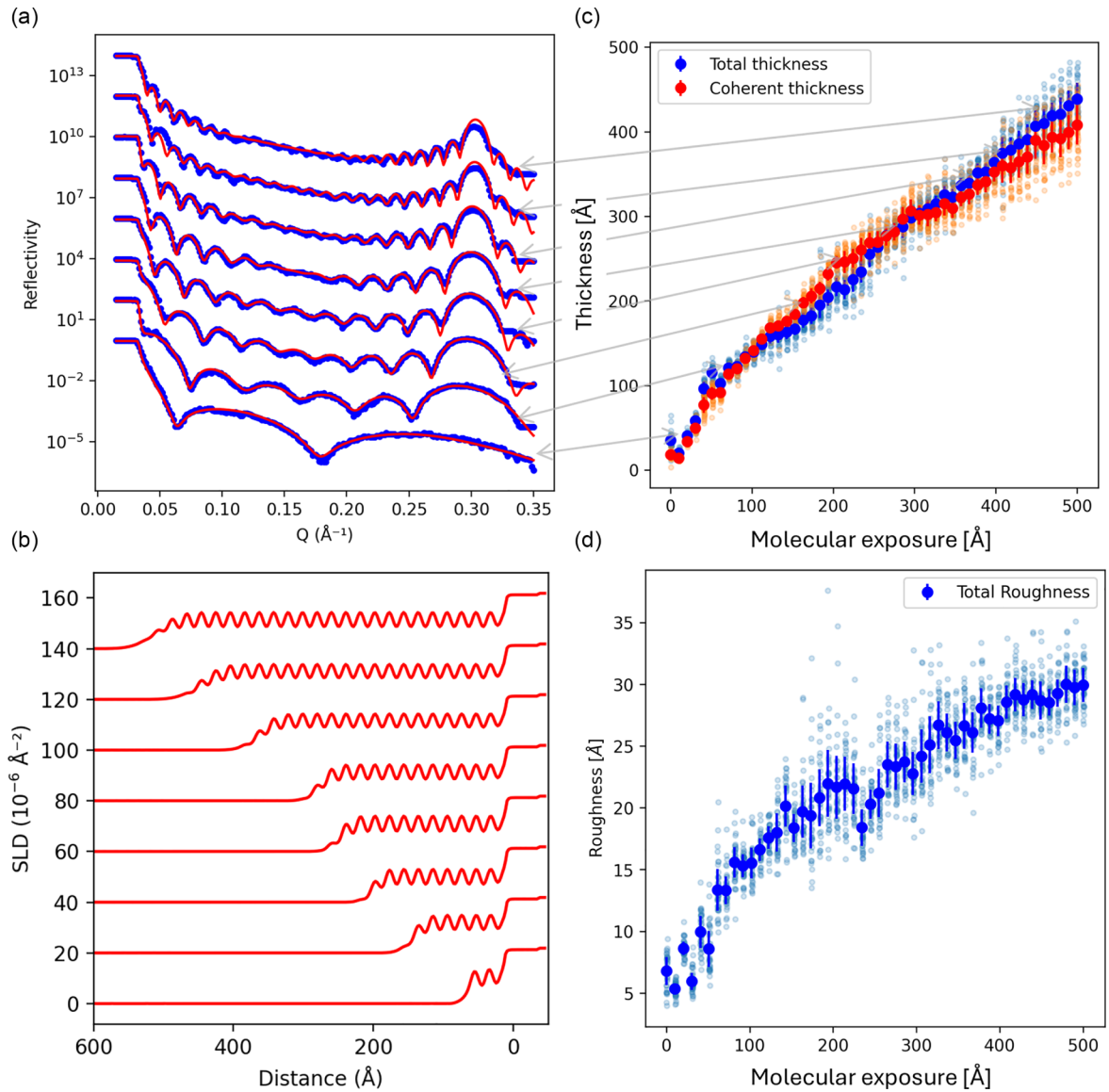
FIG. 2. Growth of the thin PTCDI-C 8 layer under the growth rate of 1 Å/second. (a) Neural network prediction polished with refnx fit of sample curves recorded within 12 ms each during the growth. (b) Corresponding SLD profile of the sample curves indicating the formation of the layers. (c) The evolution of the absolute (blue) and coherent (orange) thickness, mean value, and MAE variation is shown in the plot. (d) Absolute roughness as a function of the molecular exposure where mean value and MAE variation are shown.
