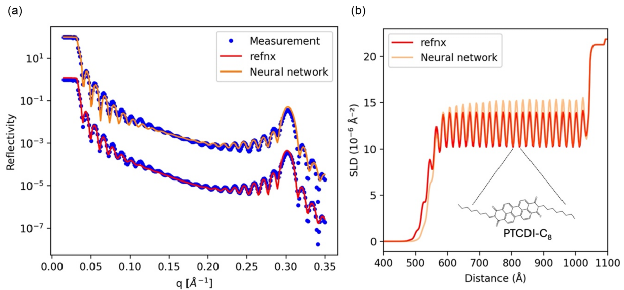
FIG. 1. A comparison of the refnx fit and NN prediction on the standard 400-second long XRR measurement of a thin PTCDI- C_8 film using the same multilayer structure model. (a) refnx fit of the measurement (red) and the NN prediction (orange). (b) Corresponding SLD profiles of the sample for the refnx fit (red) and the NN prediction (orange). The inset shows the chemical structure of PTCDI- C_8 with dashed lines indicating the size of the molecular core and the interdigitating side chains in the SLD profile.
