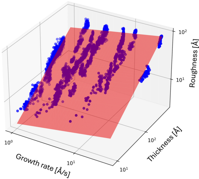
FIG. 3. Roughening of a thin layer as a function of the thickness and growth rate. The red plane is a fit using the scaling relation of Eq. (2). The fit uses NN roughness predictions of all XRR curves within our study.
