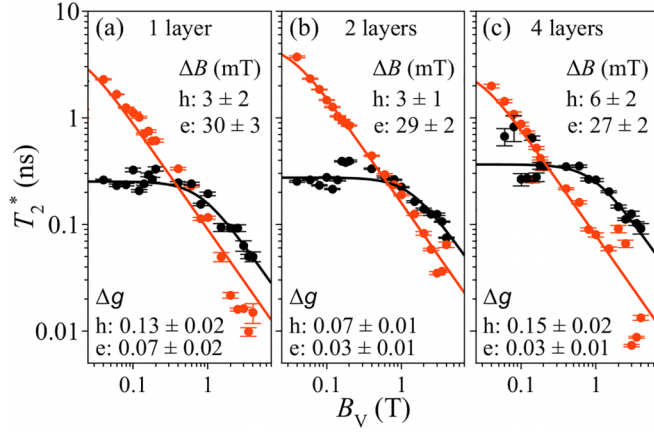
FIG. 3. Spin dephasing time ( T_2^* ) measurements as a function of transverse magnetic field ( B_V ) for InAs/InAlGaAs QD samples with different numbers of layers. The data are presented on log-log scales for samples containing one, two, and four QD layers [panels (a), (b), and (c), respectively]. Red circles represent hole spin dephasing times, and black circles represent electron spin dephasing times. The solid lines show fits to the experimental data using a model that accounts for g -factor spread and magnetic field fluctuations. The fitting parameters, including magnetic field spreads ( \Delta B_h , \Delta B_e ) and g -factor spreads ( \Delta g_h , \Delta g_e ), are displayed for each sample. The measurement configuration is the same as in Fig. 1.
