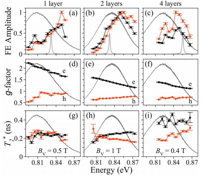
FIG. 2. Energy-dependent parameter characterization for QD samples with different numbers of layers (one, two, and four layers). Panels (a), (b), and (c) display the normalized Faraday ellipticity amplitudes A_i from Eq. (9), red points represent holes, and black ones electrons. Gray lines additionally show the PL and the laser pulse profile for later experiments. Panels (d), (e), and (f) show the extracted Lande g -factors. Panels (g), (h), and (i) show the spin dephasing times T_{2,i}^* measured at magnetic field values shown in the panels. Pump powers for the one-layer sample were 15 mW, and for two- and four-layer samples, 20 mW. All measurements were performed at 6 K and a probe power of 2 mW.
