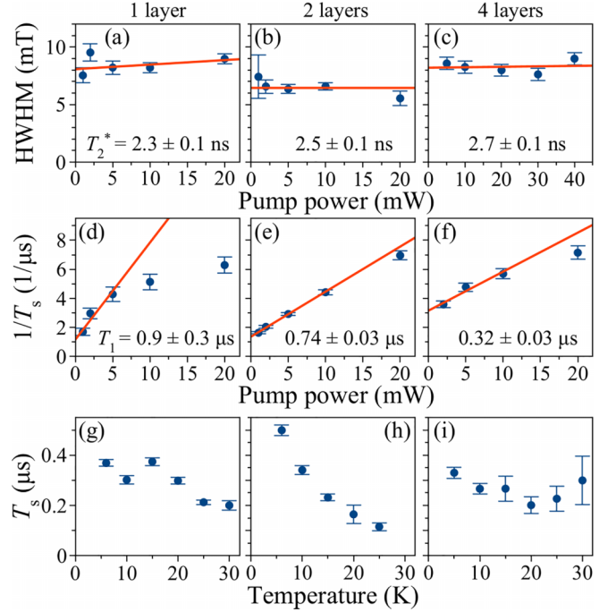
FIG. 6. Spin dynamics measurements for QD samples with different numbers of layers (one, two, and four layers). Panels (a), (b), and (c) display the half-width at half-maximum (HWHM) of Hanle curves as a function of pump power, from which spin dephasing times T_2^* are extracted through linear extrapolation to zero pump power. Panels (d), (e), and (f) show the inverse spin lifetime ( 1/T_s ) vs pump power measured under a longitudinal magnetic field of 0.1 T, with the intrinsic longitudinal spin relaxation times T_1 determined by extrapolating the linear fits to zero pump power. Red lines are linear fits for extrapolation to zero. Panels (g), (h), and (i) show the spin lifetime in Faraday geometry dependency on the sample temperature, measured using the spin inertia method. All the samples are subjected to a magnetic field of 0.1 T. Pump power for the different panels is (g) 5 mW, (h) 2 mW, and (i) 2 mW. Measurements in panels (a)–(f) were performed at 6 K and a probe power of 2 mW.
