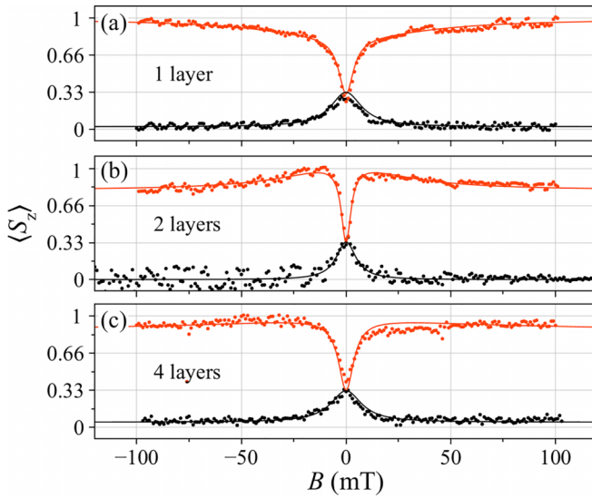
FIG. 4. Polarization recovery curves (red) and Hanle effect measurements (black) for (a) single-layer sample, (b) two-layer sample, and (c) four-layer sample. The measurements show the total spin polarization \langle S_z \rangle as a function of magnetic field strength. The fits for PRCs are done with Eq. (5). The pump power is 20 mW and probe power is 2 mW for both PRCs and Hanle, for single- and two-layer samples, and the pump power for the four-layer sample is 10 mW. All measurements are performed at 6 K.
