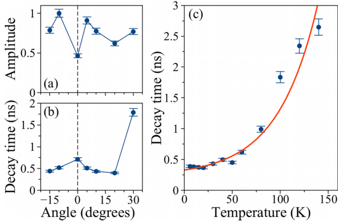
FIG. 5. Characterization of the additional exponential decay component observed in a four-layer QD sample. (a) Normalized amplitude of the exponential component as a function of magnetic field angle measured away from the Voigt geometry. (b) Decay time of the exponential component as a function of magnetic field angle. (c) Temperature dependence of the exponential component decay time. All measurements are performed at a temperature of 6 K [except for (c)], a transverse magnetic field strength of 0.4 T, a pump power of 10 mW, and a probe power of 2 mW.
