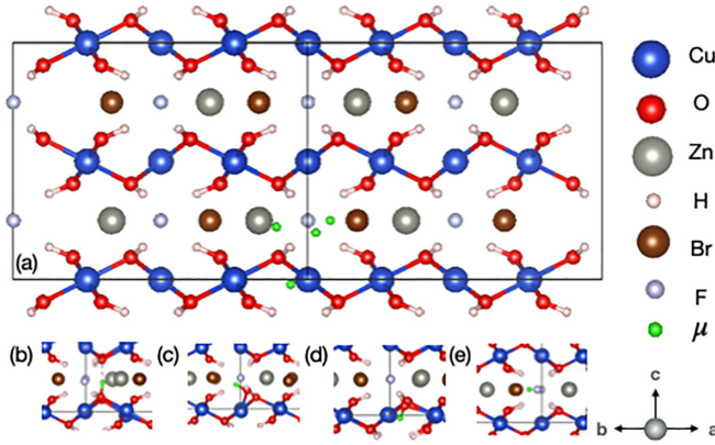
FIG. 1. (a) Candidate muon stopping sites in Zn-barlowite identified using classical DFT + \mu (green) in the undistorted 2 \times 2 \times 1 supercell. (b)–(d) Close-up views of the \mu -OH sites, showing local distortions induced by the muon. (e) F- \mu -Br stopping site with its associated local distortion.
