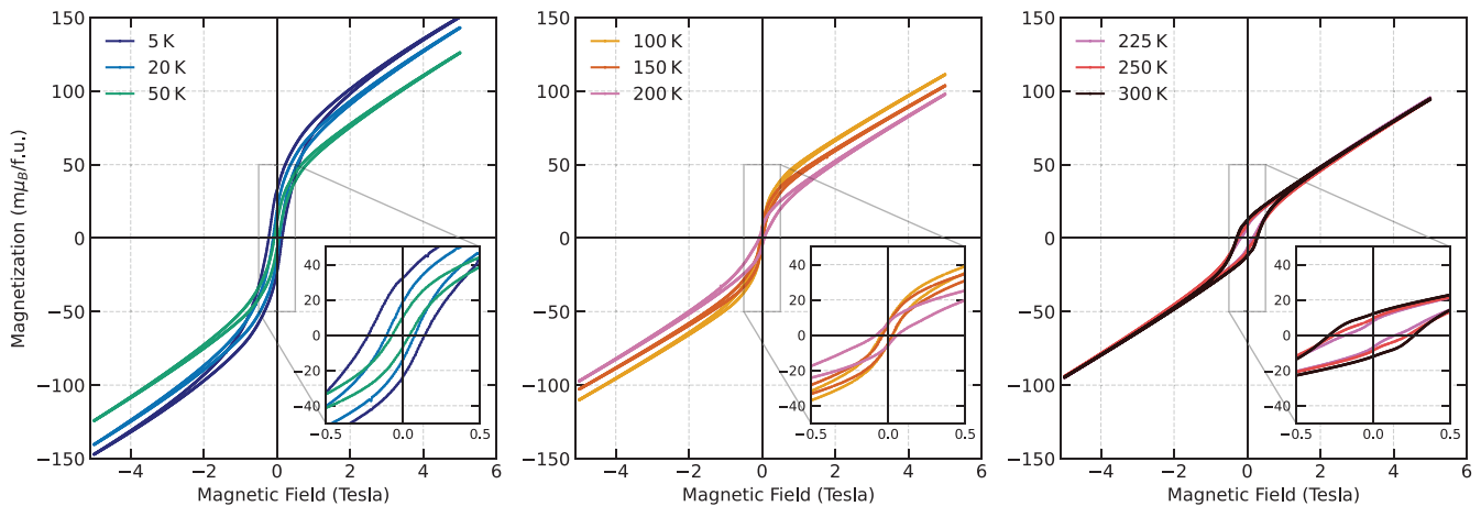
FIG. 7. Extended isothermal bulk magnetization. Magnetization of \text{Mn}_3\text{Sn} as a function of applied external magnetic field, measured across a wide range of temperatures. The data are grouped into three panels by temperature range for clarity. The insets provide a magnified view of the low-field region to more clearly illustrate the temperature evolution of the hysteresis loops.
