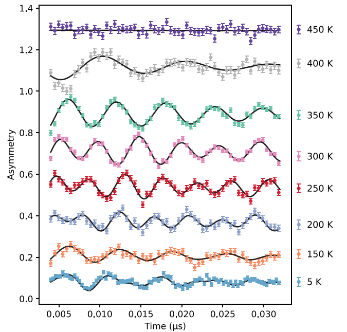
FIG. 4. Temperature evolution of ZF- \mu^+ SR spectra. Zero-field (ZF) muon spin relaxation ( \mu^+ SR) asymmetry of Mn 3 Sn measured at various temperatures from 5 to 450 K. Solid black lines show fits to the experimental data using Eq. (2). Successive spectra are vertically offset by a constant value for clarity of presentation.
