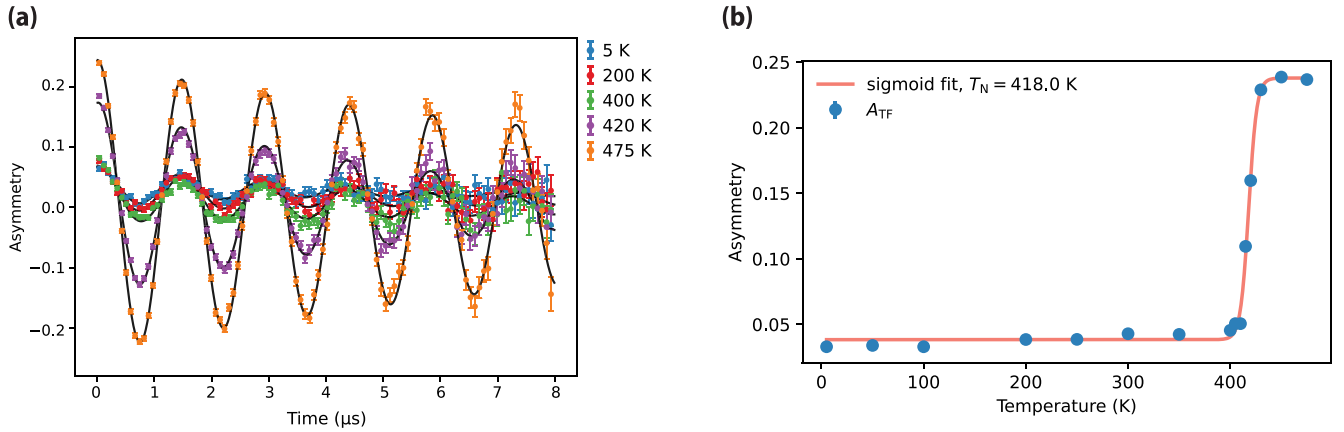
FIG. 3. Néel temperature from TF- \mu^+ SR. (a) Muon spin relaxation ( \mu^+ SR) spectra of Mn 3 Sn measured in an applied transverse field (TF) of B = 50 G at various temperatures. Solid black lines show fits to the experimental data using Eq. (1). (b) Evolution of the fitted TF asymmetry coefficient, A_{TF} , as a function of temperature. The sharp magnetic transition is fitted with a sigmoid function (red curve), extracting a Néel temperature of T_N = 418 K.
