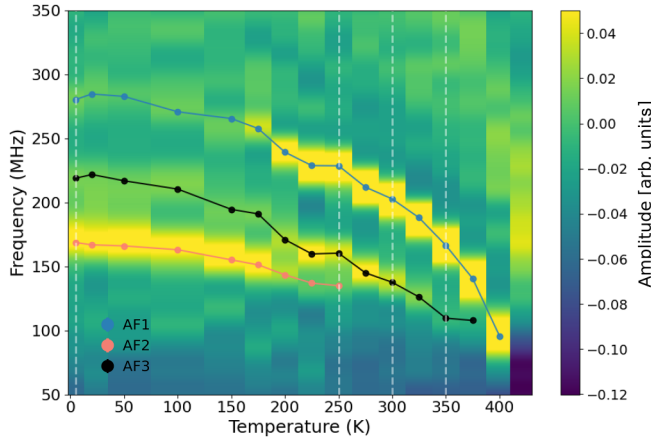
FIG. 6. Fourier transform heat map of the ZF- \mu^+ SR signal. Two-dimensional (2D) heat map showing the real part of the Fourier transform (FT) of the asymmetry signal over the first 0.05 \mu s as a function of temperature. Vertical dashed lines indicate temperatures where high-statistics measurements were performed. Overlaid points denote the fitted zero-field (ZF) precession frequencies (AF1, AF2, and AF3) extracted using Eq. (2), matching the parameters presented in Fig. 5(a).
