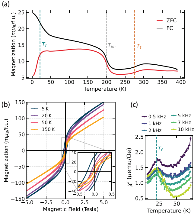
FIG. 2. Bulk magnetic characterization. (a) Temperature dependence of the magnetization using zero-field-cooled (ZFC) and field-cooled (FC) protocols with an applied magnetic field of B = 0.1 T, marking key transition temperatures ( T_f , T_{im} , and T_t ). (b) M(H) curves showing magnetization as a function of applied magnetic field between -5 and 5 T at 5 , 20 , 50 , and 150 K. The inset provides a magnified view of the low-field region to highlight the temperature evolution of the hysteresis. (c) Real part of the ACMS, \chi' , as a function of temperature across various frequencies, showing a peak near T_f .
