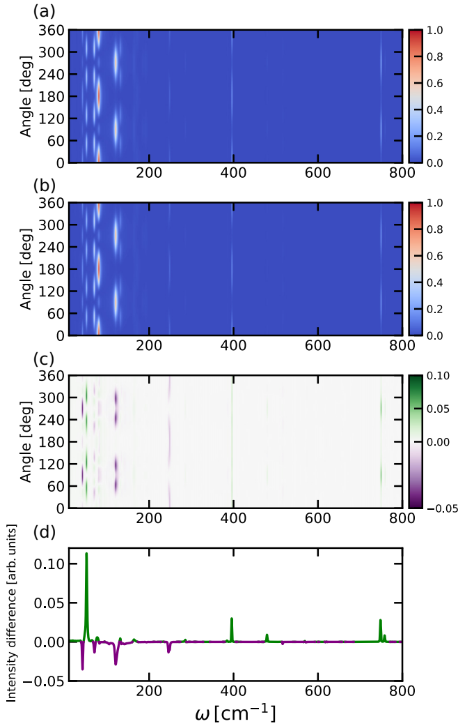
FIG. 1. (a) PO-Raman spectrum of anthracene at 100K obtained with the “full-ML” framework ( 4 \times 4 \times 4 supercell). (b) PO-Raman spectrum of anthracene at 100K obtained with the RGDOS-ML framework ( 4 \times 4 \times 4 supercell). Intensities are normalized to the highest peak amplitude in both cases. (c) Difference between the PO-Raman spectra obtained with the two frameworks. Negative values correspond to features that are more intense in full-ML than in RGDOS-ML and vice versa. (d) Difference between the unpolarized Raman spectra obtained with the two frameworks.
