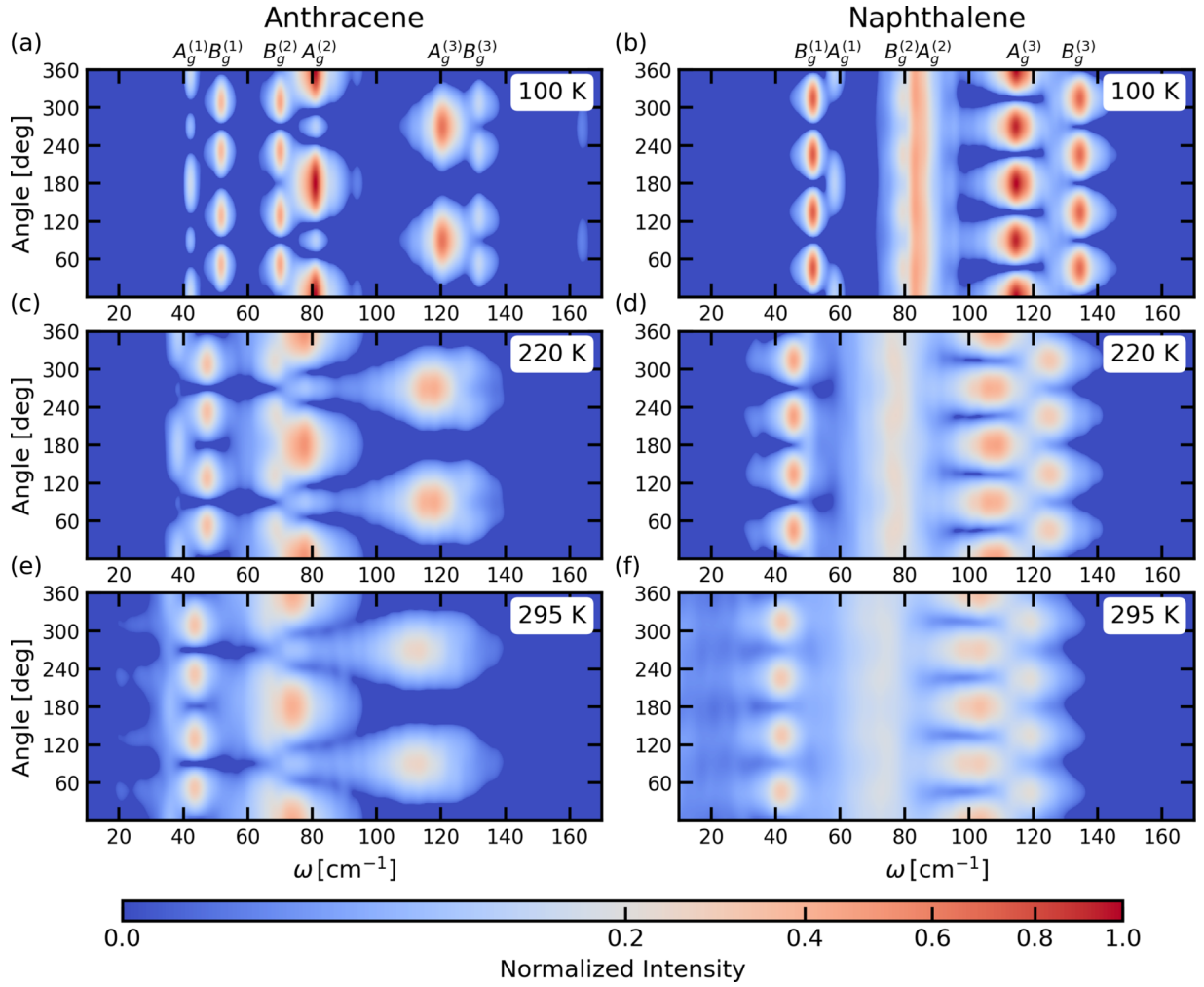
FIG. 3. Temperature dependence of the parallel configuration PO-Raman spectra of anthracene (a), (c), (e) and naphthalene (c), (d), (f) in the intermolecular motion range of 10 to 170 \text{cm}^{-1} , obtained with the RGDOS-ML method. The intensity is normalized to the maximum intensity of the 100K spectrum.
