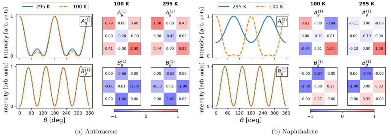
FIG. 2. Harmonic polarization dependence of the Raman intensity of modes A_g^{(1)} and B_g^{(1)} in anthracene (a) and naphthalene (b), obtained with the harmonic approximation of Eq. (7) in the parallel configuration. On the right, the corresponding Raman tensors for every mode computed with finite differences from DFPT polarizabilities along normal mode displacements of the MACE-MLIP at the 100K and 295K lattice vectors. Tensor components are normalized to their highest value for each mode. In the parallel configuration, only A_g modes can show a change in the polarization pattern with temperature (lattice expansion) within the quasiharmonic approximation. This effect is particularly pronounced in the case of naphthalene, where structural changes impact the A_g^{(1)} mode. The full set of harmonic polarization patterns and a more detailed analysis can be found in Sec. S4 of the SM [26].
