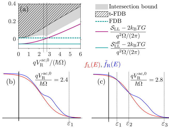
FIG. 8. Excess noise and bounds for a harmonically driven two-terminal conductor with constant transmission probability [all parameters in (a) as in Fig. 4(c) in the main text]. (b), (c) Distribution function for the hot contact (red) and the modified distribution from the cold contact due to driving (blue) at the parameter values indicated by vertical dashed lines in (a), namely, at qV_R^{ac,0} = 2.4\hbar\Omega in (b) and at qV_R^{ac,0} = 2.8\hbar\Omega in (c).
