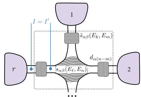
FIG. 1. Sketch of the multiterminal setup with contacts \alpha = 1, \dots, r . Time-dependent driving is applied in the leads and in the central region (patterned). Measurements of the time-averaged current and of the zero-frequency noise, when performed before or after the driven lead region (blue spots), yield the same result.
