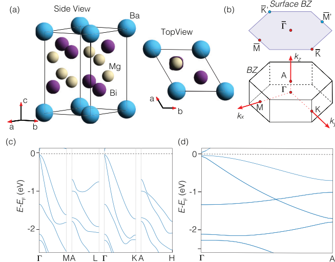
FIG. 1. (a) Side and top views of the structure and unit cell of BaMg 2 Bi 2 crystal, showing the typical CaAl 2 Si 2 structure. (b) Resulting Brillouin zone with high-symmetry directions indicated. The surface Brillouin zone is also indicated. (c) Bulk electronic structure along the in-plane high-symmetry directions. (d) Same as (c) but along the out of plane direction.
