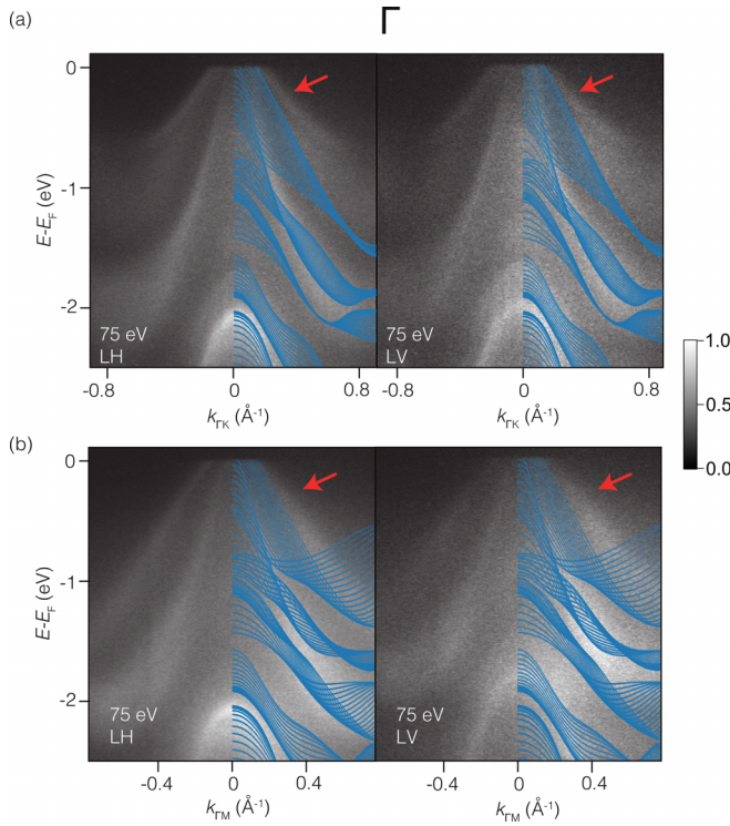
FIG. 3. (a) ARPES ( E , k ) dispersions of \text{BaMg}_2\text{Bi}_2 along the \Gamma - K and (b) \Gamma - M directions for both light polarizations indicated in the figure. The projected bulk continuum from DFT calculations (in blue) has been overlaid to the experimental spectra.
