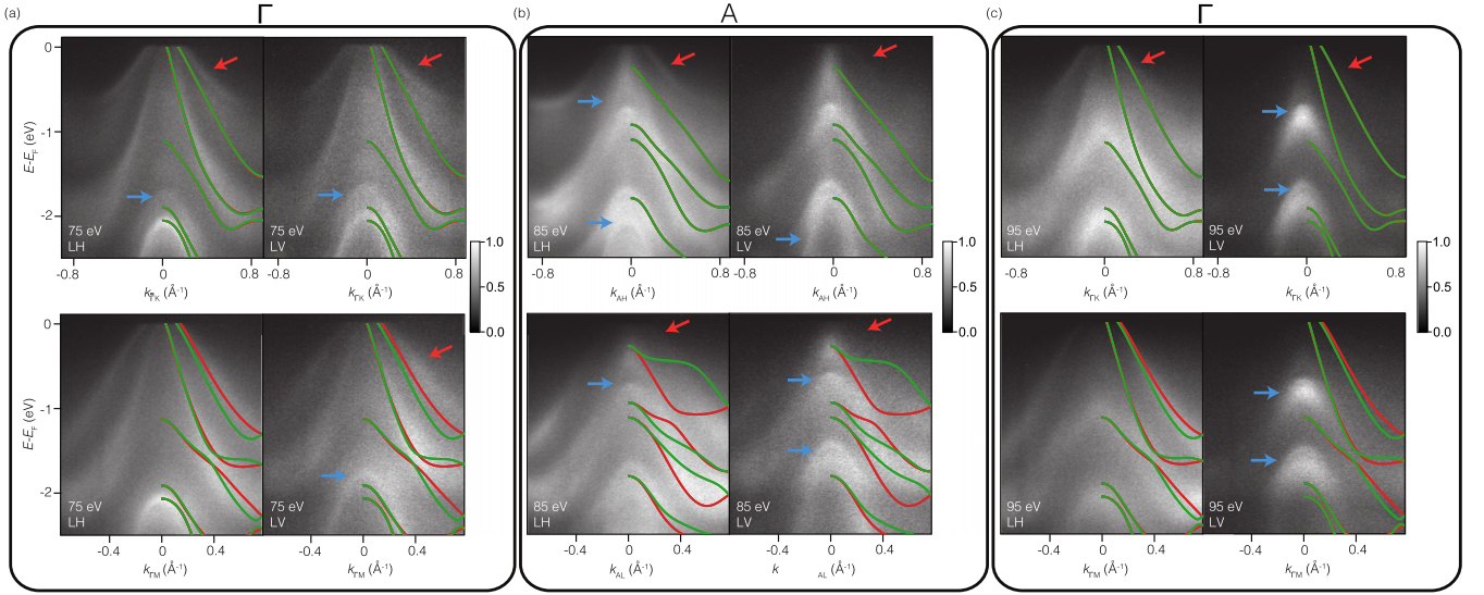
FIG. 2. (a) ARPES ( E , k ) dispersions of BaMg 2 Bi 2 along the \Gamma - K (top) and \Gamma - M (bottom) directions for both LH and LV polarizations. Spectra were acquired with 75 eV photons, corresponding to a bulk \Gamma point. (b) Same dispersions acquired with 85 eV photons, corresponding to the A point. (c) Spectra obtained with 95 eV photons, corresponding to the next bulk \Gamma point. Red and blue arrows highlight additional features not previously reported.
