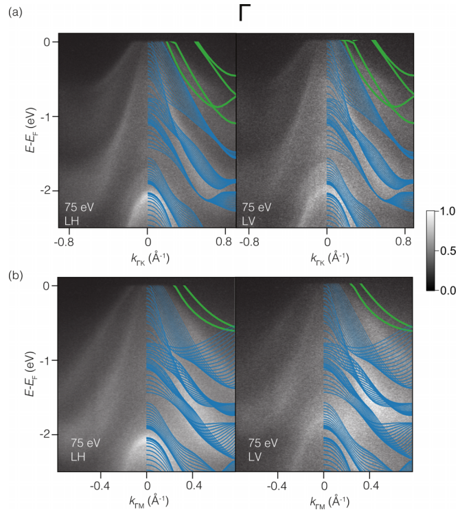
FIG. 4. (a) ARPES ( E , k ) dispersions of \text{BaMg}_2\text{Bi}_2 along the \Gamma - K and (b) \Gamma - M (bottom) directions for both light polarizations indicated in the figure. The projected bulk continuum from DFT calculations (in blue) has been overlaid to the experimental spectra. The green color indicates the surface states, calculated as described in the text.
