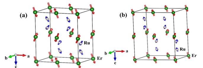
FIG. 13. IR7 and IR3 magnetic structures of BErRuO (a) below T_N and (b) above T_N , respectively. Ru moments are enlarged for better visibility.
