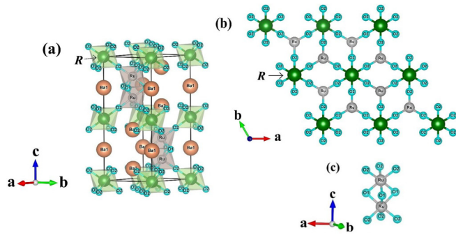
FIG. 1. (a) Hexagonal crystal structure of \text{Ba}_3\text{RRu}_2\text{O}_9 ( \text{BRRuO} ) compounds. Here Ba1 and Ba2 occupy 2b ( 0, 0, 1/4 ) and 4f ( 1/3, 2/3, z ) Wyckoff positions, respectively, R at 2a ( 0, 0, 0 ), Ru at 4f ( 1/3, 2/3, z ), O1 at 6h ( x, 2x, 1/4 ), and O2 at 12k ( x, 2x, z ). (b,c) Different views of crystal structure showing R(\text{Ru})\text{-O2-Ru}(R) and \text{Ru-O1-Ru} superexchange pathways in these compounds. Ba and O1 atoms in (b) are omitted for clarity.
