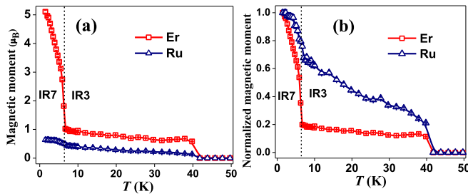
FIG. 12. Thermal variation of total (a) Er and Ru magnetic moments, and (b) normalized Er and Ru magnetic moments. The magnetic moments below and above T_N (represented by vertical dotted line) correspond to the IR7 and IR3 models, respectively.
