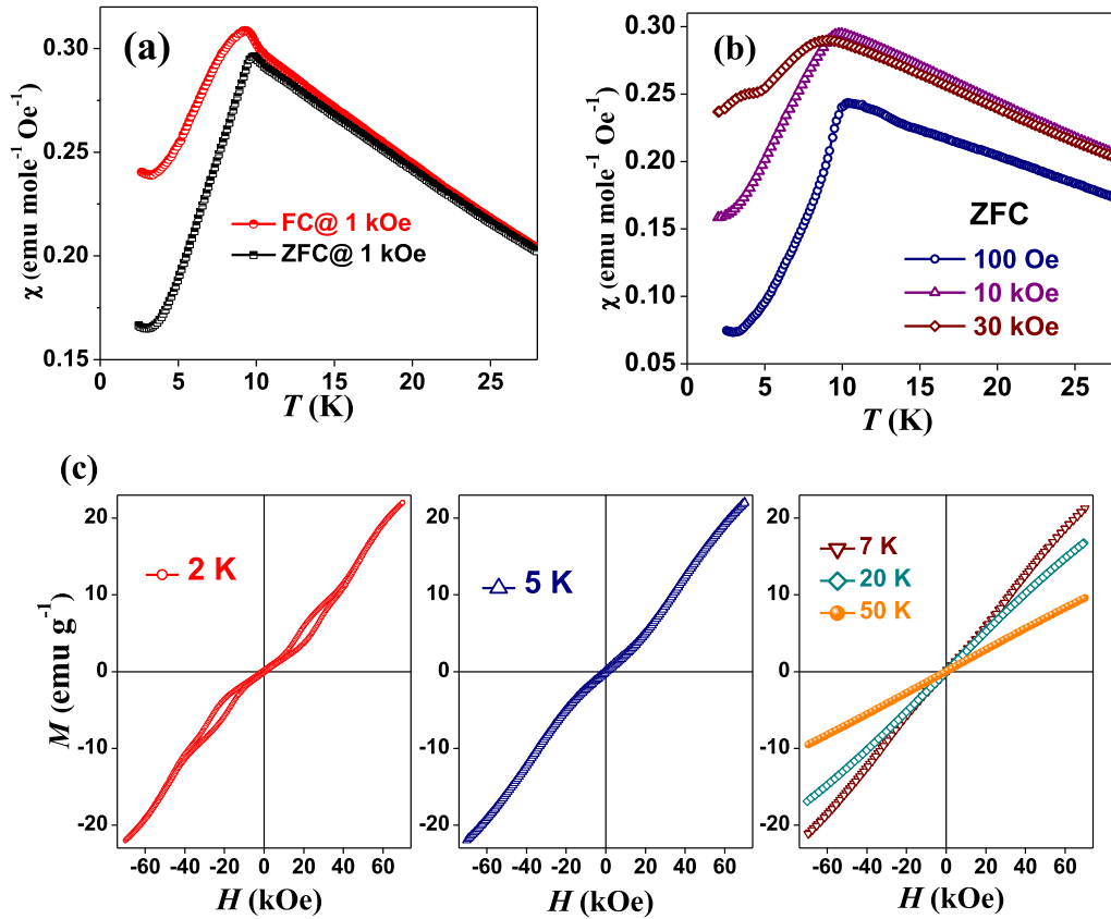
FIG. 2. (a) Temperature dependence of dc susceptibility, \chi ( = M/H ), under H = 1 kOe in ZFC and FC modes for the BTbRuO compound. (b) ZFC \chi vs T curves under different magnetic fields. (c) M - H hysteresis loops at selected temperatures.
