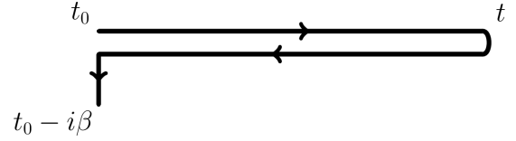
FIG. 1. Kadanoff-Baym-Keldysh time contour. It starts at time t_0 , when the system is in equilibrium and the two branches correspond to forward and backward evolution determined by the evolution operators (which first advance in time \hat{U} and then go backwards in time \hat{U}^\dagger ) for the time-dependent operators.
