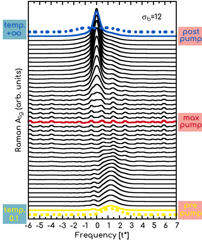
FIG. 2. Waterfall plot for the Raman scattering cross section for in case of a bad metal phase in equilibrium with Coulomb interaction U = 1 . Dotted lines correspond to the equilibrium results at temperatures T = 0.1 (yellow) and T \rightarrow \infty (blue). Different lines correspond to different time delays t_p of the probe pulse with respect to the pump pulse with t_p \in [-20, 20] , starting from times before the pump (yellow line) to the time with the maximum pump (red line) and to the late times after the pump pulse is gone (blue line). Stokes and anti-Stokes peaks are centered around frequencies \omega = U and \omega = -U , respectively. The peak at zero frequency corresponds to the elastic contribution to the scattering cross section. The probe pulse width is given by \sigma_b = 12 .
