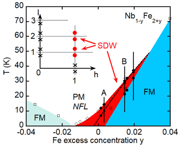
FIG. 1. Phase diagram of \text{Nb}_{1-y}\text{Fe}_{2+y} with results for bulk T_C (squares) and T_N (diamonds) from previous single-crystal (filled symbols) [30] and polycrystal (empty symbols) [31] studies. Vertical solid lines indicate the T range of previous cold neutron diffraction measurements. A and B denote samples also studied with thermal neutron diffraction reported here. Of the two ferromagnetic (FM) phases, the one on the more Fe-rich side is separated from the paramagnetic (PM) state by a /SDW at low temperatures, where NFL behavior is found as well. T_0 , the FM phase boundary buried by the SDW phase (dashed line) is an extrapolation of T_0 values (circles) measured or calculated for the single crystals. The inset shows the relevant reciprocal-space region, which was accessible during previous neutron diffraction experiments. Circles show the presence and crosses the absence of SDW peaks.
