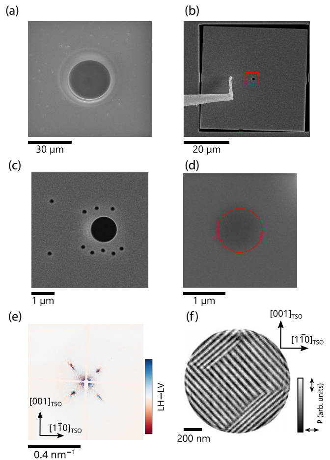
FIG. 4. Holography-assisted CDI of ferroelectric domains in KNN on TSO. (a) X-ray transparent window for the RXS measurements in Fig. 3. (b) Square Au/Cr multilayer FTH mask during transfer to the KNN sample. (c) Enlarged view of the FTH mask with object and reference holes after fastening to the sample surface, corresponding to the red framed area in (b). (d) FTH sample from the KNN side. The transparent circular window for the object is circled. (e) Difference in the diffraction patterns with LH and LV polarization obtained at the maximum ferroelectric RXS at the O K -edge [see Figs. 3(a) and 3(b)]. The superdomain diffraction peaks appear with interference fringes. (f) Reconstructed holographic XLD difference image of the ferroelectric superdomains with 57-nm and 44-nm in-plane stripe periods.
