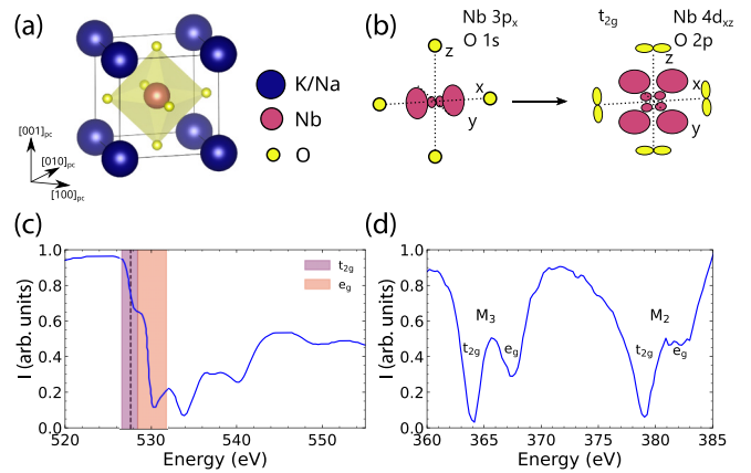
FIG. 1. (a) The pseudocubic (pc) perovskite unit cell of KNN shows the octahedral coordination of Nb 5+ by O 2- . (b) Sketch of the electronic orbitals in the ground (left) and excited hybridized state (right). The anisotropy in the O 2p orbitals causes strong XLD at the O K -edge. (c) X-ray transmission spectrum of 37-nm KNN on TSO at the O K -edge. The peaks assigned to hybridization with 4d t_{2g} and e_g are shaded. The broken vertical line indicates the photon energy of maximum XLD. (d) X-ray transmission spectrum of 37-nm KNN on TSO at the Nb M_{3,2} -edges.
