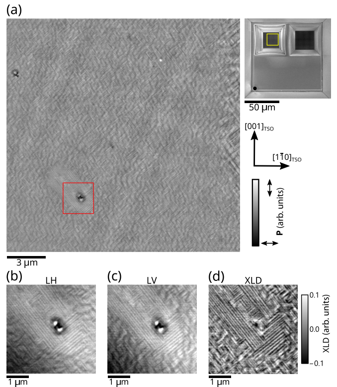
FIG. 2. (a) STXM image of ferroelectric domains in KNN in an 18 \mu\text{m} \times 18 \mu\text{m} area. Horizontally polarized x-rays at the O K -edge tuned to the energy of 2p\text{-}4d t_{2g} hybridization were used. The in-plane components of the ferroelectric polarization \mathbf{P} are in [001]_{\text{TSO}} and [1\bar{1}0]_{\text{TSO}} directions. An SEM image of two x-ray transparent windows in the substrate is shown in the top right with the imaged region framed in yellow. (b)–(d) Higher-resolution images of the framed area in (a) with LH/LV polarized x-rays and the corresponding XLD image, emphasizing the ferroelectric domains and suppressing topography contrast.
