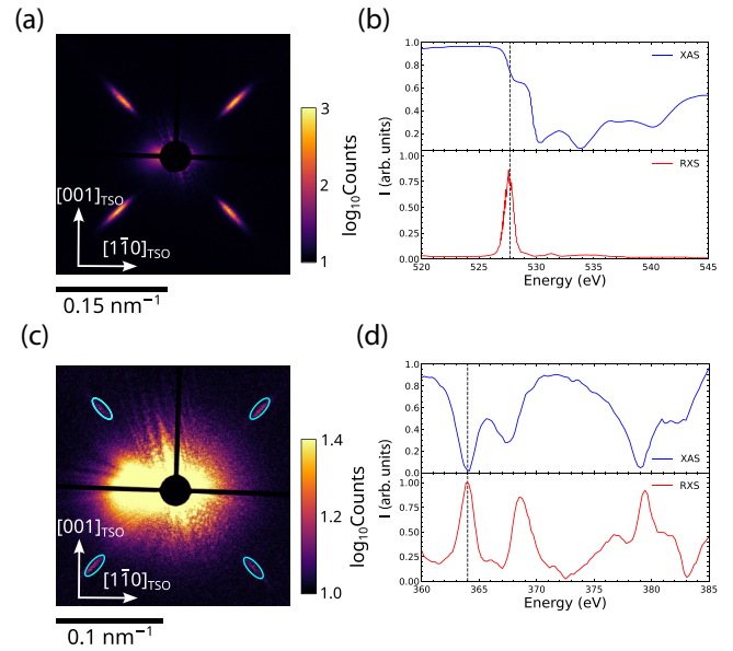
FIG. 3. Resonant x-ray scattering from ferroelectric domains in 37-nm KNN on (110) TSO. (a) RXS at the O K -edge (527.7 eV) shows the presence of diffraction peaks corresponding to the ferroelectric superdomains with ferroelectric stripes of 50-nm mean period in two directions. (b) The normalized x-ray transmission (XAS) and RXS signal from the diffraction peaks are shown. The maximum intensity of diffraction from the superdomains is at the t_{2g} hybridization of the O 2p and Nb 4d states. (c) RXS signal at the Nb M_{3,2} -edges (364 eV) also shows the ferroelectric domains with lower intensity. (d) Intensity of the RXS signal is detectable at the crystal-field split transitions of the Nb M_{3,2} -edges.
