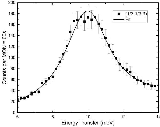
FIG. 2. A constant- Q scan at the K point on the HB3 thermal triple-axis spectrometer. A background scan was also performed using the same configuration, but driving the analyzer flat. This removes coherent scattering from the analyzer, but preserves the incoherent signal that is a source of spurious scattering. The background-subtracted data are shown, where the solid line is a fit to the Hamiltonian with zero DM term, and convoluted with the instrumental resolution.
