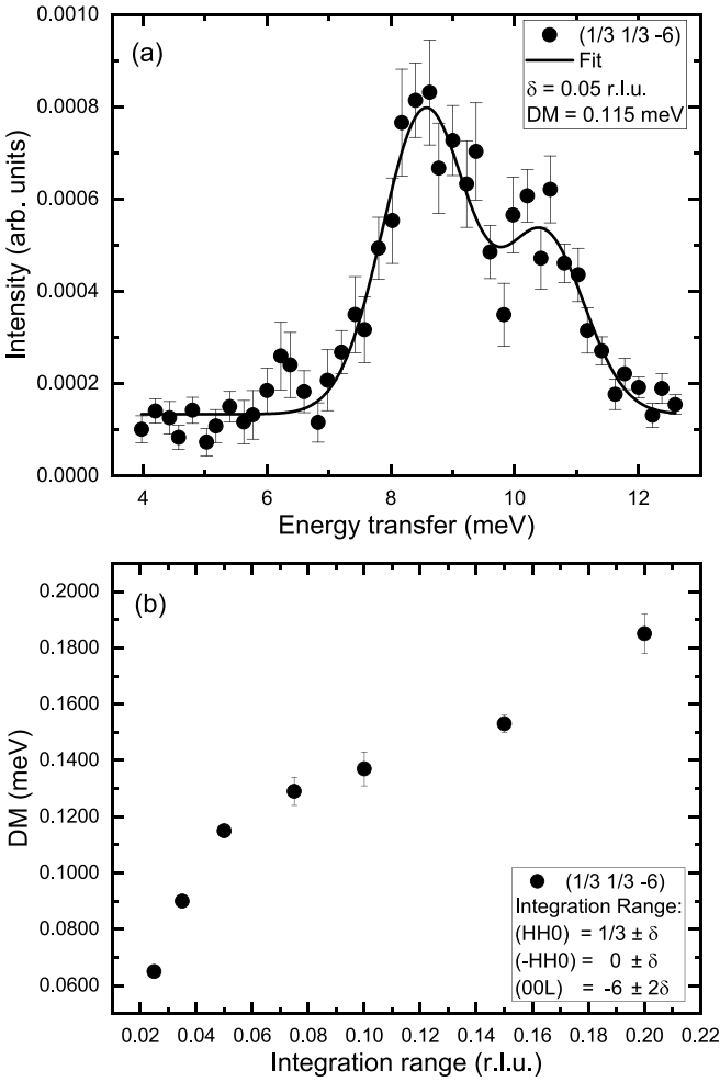
FIG. 1. (a) A line cut through the K point by integrating (\frac{1}{3} \pm 0.05 \frac{1}{3} \pm 0.05 - 6 \pm 0.1) and \Delta E = 0.25 meV using the data collected on ARCS. The data were then fit to the Hamiltonian described in the text, including the DM term. The fit value for the DM term was 0.115(3) meV, in good agreement with Ref. [8]. (b) When the procedure done in the top panel was repeated for integrating different Q volumes around the K point, the fit value of the DM term was found to monotonically decrease with the integration range. The fits did not converge for volumes with \delta < 0.025 r.l.u.
