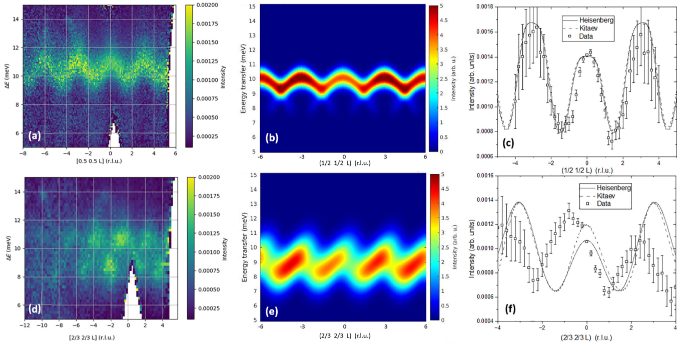
FIG. 3. (a) Spin waves measured along the (\frac{1}{2} \frac{1}{2} L) direction, where there is no contribution from a DM term. This data were used to constrain the fits to the out-of-plane exchange constants. (b) Spin-wave simulations of the (\frac{1}{2} \frac{1}{2} L) dispersion with the Kitaev interaction described in the text. (c) The data along (\frac{1}{2} \frac{1}{2} L) at the top of the band ( \Delta E = 10.5 meV) overlaid with simulations using a purely Heisenberg Hamiltonian and no DM interaction (solid line), and the same Hamiltonian, but with the nearest-neighbor in-plane interaction being a Kitaev interaction (dashed line). Both agree well with the data, as this reciprocal space direction is not sensitive to changes in these parameters. (d) Spin waves measured along the (\frac{2}{3} \frac{2}{3} L) direction, where the dispersion is seen to be anisotropic relative to L=0 . (e) The simulations along the panel (a) direction including the Kitaev interaction. This distorts the spin-wave spectrum and produces an anisotropy along the L direction. (f) The data overlaid with the Heisenberg and Kitaev exchange simulations along the top of the band ( \Delta E = 10 meV). This shows that the anisotropy produced by the Kitaev term does not change the band minima/maxima, fundamentally different from the spin-wave anisotropy observed in the data.
