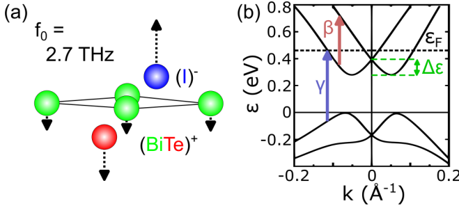
FIG. 1. (a) Atomic displacement and central frequency of an A_1 phonon mode in BiTeI [20]. (b) Rashba-split band structure of BiTeI (adapted from [26]; \Delta\epsilon = 100 meV). The transition \beta (red dashed line at 0.37 eV) represents the highest-energy intraband transition. The transition \gamma (blue dashed line at 0.52 eV) is the lowest-energy interband transition corresponding to the electronic excitation from the valence band to a free state above the Fermi energy \epsilon_F (dashed black line).
