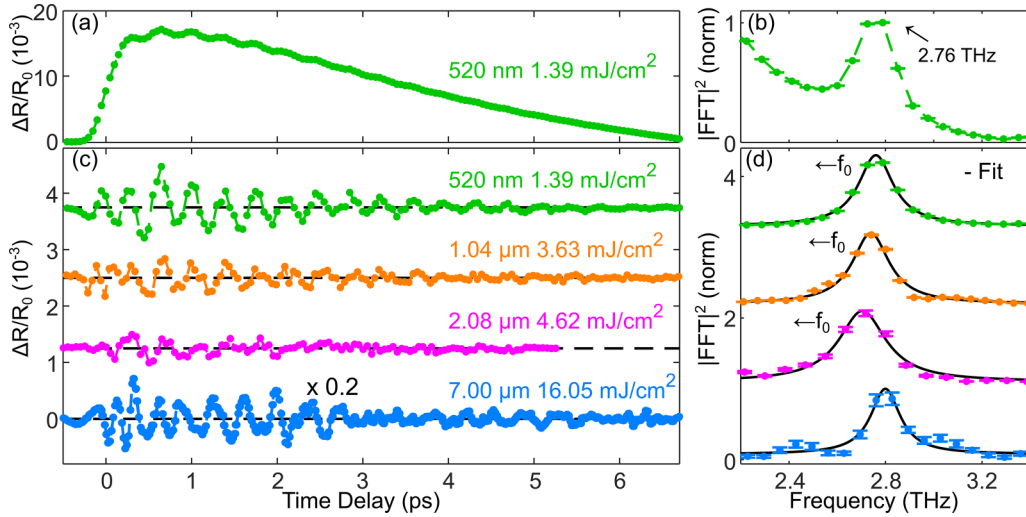
FIG. 2. (a) Dynamics of the normalized reflectivity of BiTeI induced by 520-nm laser pulses. The fluence was set to 1.39 mJ/cm 2 . (b) Power spectrum of the time trace shown in panel (a), obtained via Fourier transform. (c) Oscillatory component of the transient reflectivity for pump wavelengths spanning the visible, near-infrared, and mid-infrared spectral ranges after subtraction of the incoherent background. For the 2.08- \mu m data (purple), the shorter coherence time (4.2 ps) allows us to limit the maximum scanned delay time to 5.3 ps, which improves the statistics while keeping the measurement time constant over the entire dataset shown in this figure. Note that for the 7.00- \mu m data (blue), the time trace was scaled with a factor of 0.2 for presentation purposes. (d) Power spectra of the time traces shown in panel (c). Each dataset is normalized on its peak value at the respective central frequency f_0 . The solid black lines represent a fit with a Lorentzian function (details in [21]). For interband excitation (520 nm to 2.08 \mu m) f_0 redshifts with increasing fluence (see explanation in the main text).
