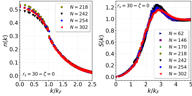
FIG. 2. Momentum density n(k) and static structure factor S(k) of paramagnetic two-dimensional uniform electron liquids using SJB WFs with density parameter r_s = 30 at different system sizes N obtained by VMC at zero twist. k_F is the Fermi wave vector.
