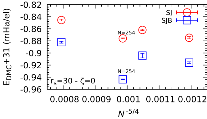
FIG. 4. TA DMC energies for paramagnetic ( \zeta = 0 ) 2D UELs with density parameter r_s = 30 obtained using SJ and SJB WFs. The differences between the SJB and SJ energies for N = 218, 242, 254 , and 302 are -0.041(2), -0.042(4), -0.068(1) , and -0.037(2) mHa/el., respectively.
