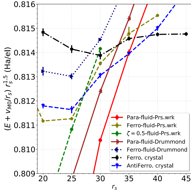
FIG. 6. DMC energy extrapolated to infinite system size as a function of r_s for 2D UELs with spin polarizations \zeta = 0, 0.5 , and 1 . Our results (“Prs-wrk”) are compared with those of Drummond and Needs [36], which include paramagnetic ( \zeta = 0 ) and ferromagnetic fluids ( \zeta = 1 ) and ferromagnetic and antiferromagnetic hexagonal Wigner crystals. The Madelung energy of a hexagonal lattice, -v_{M0}/r_s , where v_{M0} = -0.50751467391482663 is the Madelung constant at r_s = 1 , has been subtracted from all the DMC energies.
