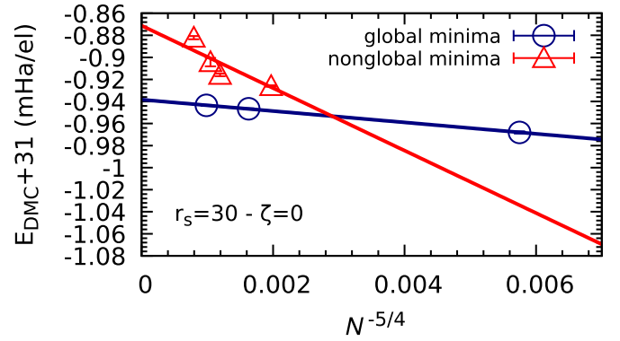
FIG. 5. Extrapolation of TA DMC fluid energies to the thermodynamic limit of infinite system size for paramagnetic ( \zeta = 0 ) 2D UELs with density parameter r_s = 30 . The red data points are assumed to be trapped in nonglobal minima during optimization and do not correspond to the fluid ground state.
