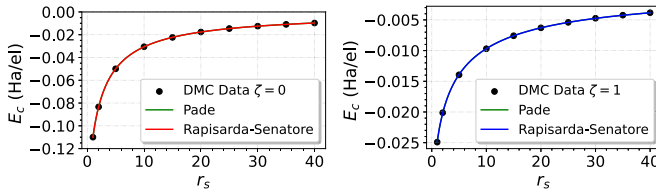
FIG. 7. DMC correlation energy of 2D uniform electron liquid with \zeta = 0 (left panel) and spin polarization \zeta = 1 (right panel) fitted by Padé and Rapisarda and Senatore [21] functions. The fitting parameters are listed in Table IX. Both fitted functions provide similar asymptotic behavior.
