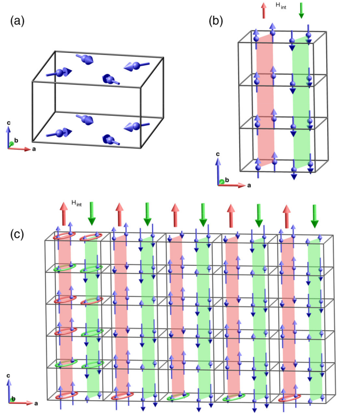
FIG. 2. (a) In-plane (all-in-all-out) Fourier component, m_{xy}^{k1} . (b) Out-of-plane Fourier component, m_z^{k1} , defining the alternating nominally up direction of the internal staggered field, H_{int} . (c) An an-harmonic spin density wave consisting of three Fourier components, m_z^{k1} , m_z^{k2} , and m_z^{k3} . The figure was created using Mag2Pol [33].
