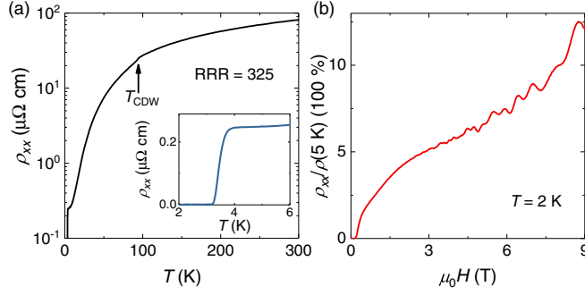
FIG. 1. (a) Temperature dependence of the resistivity of a typical sample with the RRR as high as 325. The kink at 94 K corresponds to the CDW transition. The inset shows the low-temperature resistivity with a sharp superconducting transition at 3.5 K. (b) Resistivity at 2 K divided by the normal-state resistivity \rho(5\text{ K}) as a function of magnetic field. The high RRR and magnetoresistance, sharp superconducting transition, and intense quantum oscillations suggest the high quality of the samples.
