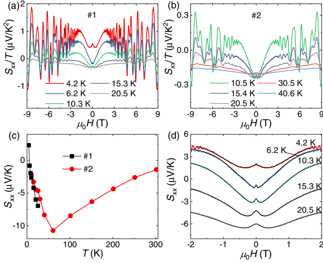
FIG. 3. (a), (b) Magnetic field dependence of the Seebeck signals for samples #1 and #2, respectively. (c) Temperature dependence of the Seebeck coefficient at zero field for both samples. (d) Seebeck signal of sample #1 with the fitting lines of the two-band expression (2).
