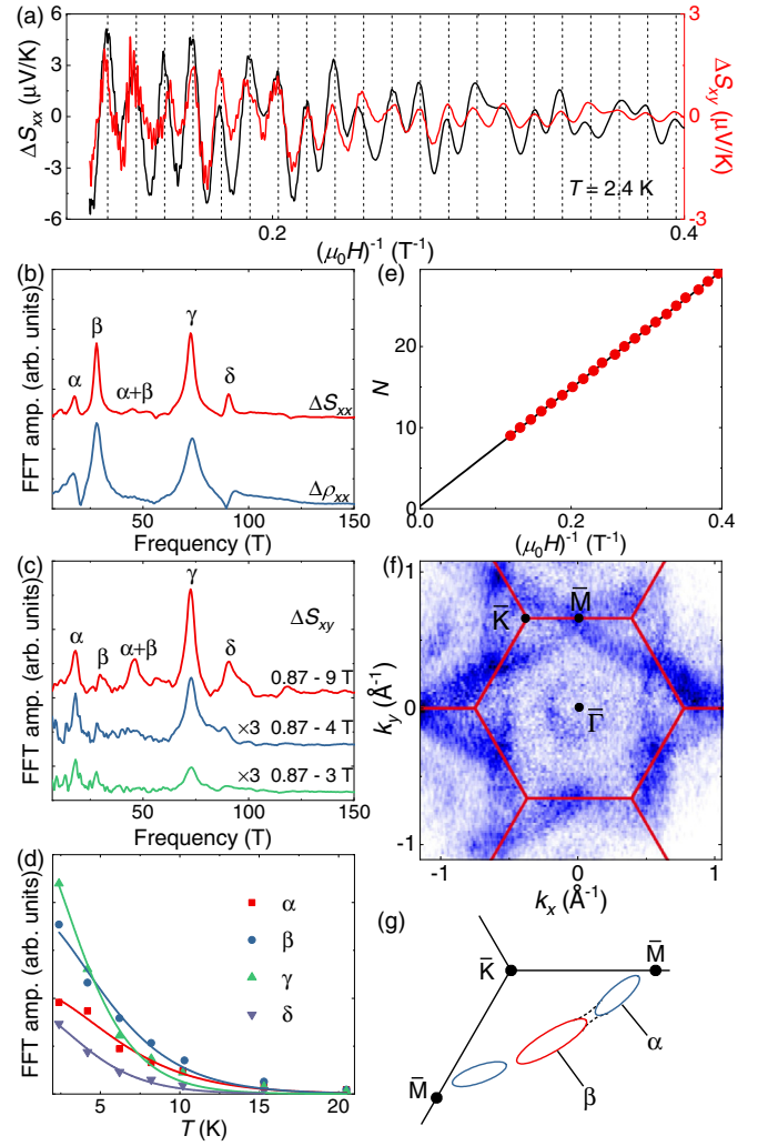
FIG. 4. (a) Oscillation parts of both S_{xx} and S_{xy} at 2.4 K. A primary frequency of F_\gamma = 72 T can be identified and the peaks are marked by dashed lines. (b) FFT spectrum of the Seebeck and SdH oscillations with the peaks are labeled. The highest peak \gamma corresponds to the primary frequency shown in (a). (c) FFT spectrum of the Nernst oscillations obtained from different magnetic ranges. A fifth peak with frequency close to F_\alpha + F_\beta appears but is absent below 3 T. (d) Amplitudes of the four main peaks as a function of the temperature, with the solid lines representing the LK fitting. The effective masses obtained from \Delta S_{xx} and \Delta S_{xy} have very close values. (e) Index plot obtained from the primary oscillation of \Delta S_{xx} shown in (a). (f) FS mapping measured by the ARPES at 33 K with the Brillouin zone and high-symmetry points superposed. (g) Possible sketch of FSs \alpha and \beta , with a breakdown path marked by the dashed lines.
