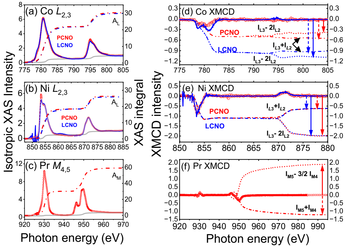
FIG. 8. (a)–(c) Isotropic XAS spectra ( \frac{1}{2}(\mu^+ + \mu^-) ) and the XAS integral ( \int(\mu^+ + \mu^-)dE ) of Co, Ni, and Pr for LCN0 and PCNO. The grey line represents the background. (d)–(f) The resulting XMCD and the corresponding integration for the sum-rule analysis. The solid and dashed arrows represent the direction of the spin and orbital moments.
