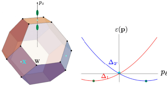
FIG. 1. (Left) Brillouin zone of the face-centered-cubic lattice. The X point (cyan) lies at the center of a square face, with four equivalent W points indicated by black dots around each X point. The two Si valleys (green ellipsoids) are located at \pm k_1 from the X point along the longitudinal ( z ) direction. (Right) Energy dispersion of the \Delta_1 (red) and \Delta_{2'} (blue) bands near the X point in Si, shown as a function of longitudinal momentum p_\ell = p_z . These bands, which form the Si valleys, emerge from the two-dimensional representation of the space group at the X point when moving away from this high-symmetry location. The energy of the X point is about 80 meV above the degenerate conduction band minimum.
