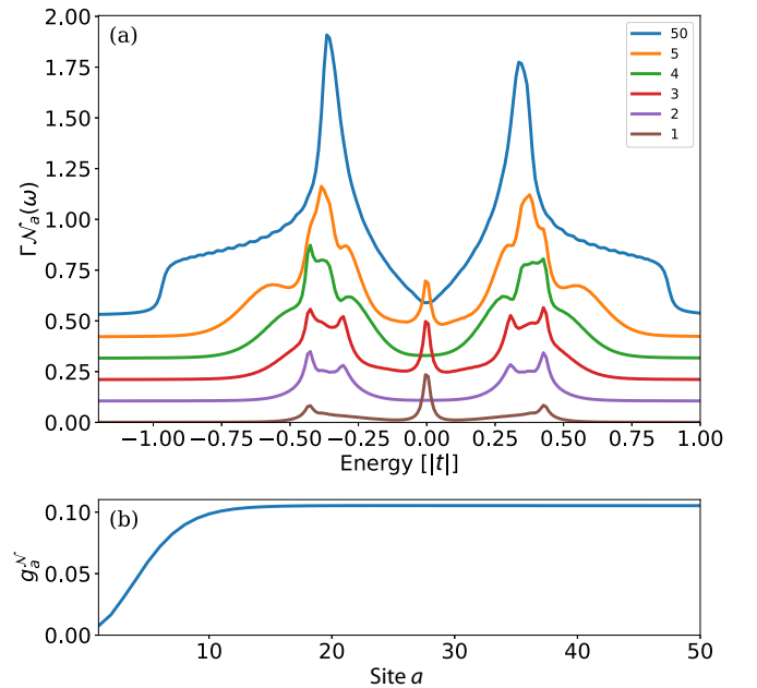
FIG. 7. (a) Cuts of the local density of states \Gamma \mathcal{N}_a(E) in Fig. 6 ( N_x = 100 , \delta = 0.05 ) at sites between 1 and 50. Each consecutive curve is shifted upwards by 0.105 for clarity. (b) The spatial dependence of the Gutzwiller factor g_a^N that enters into the LDOS defined in Eq. (15).
