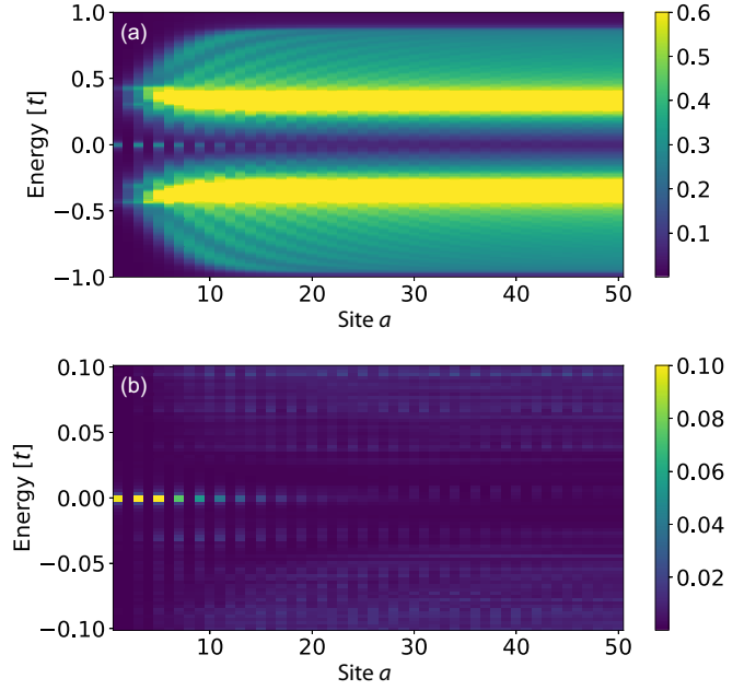
FIG. 6. Local density of states \Gamma \mathcal{N}_a(E) , scaled by the Lorentzian width \Gamma of the delta functions in Eq. (15), for the same slab as in Fig. 5 ( N_x = 100 , \delta = 0.05 ). In (a) we show the full spectrum as function of coordinate a using \Gamma = 0.015 . (b) Focus on the low-energy part of the spectrum, where the zero-energy Andreev bound states are clearly seen with a smaller \Gamma = 0.001 .
