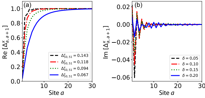
FIG. 8. The real (a) and imaginary (b) parts of the pairing amplitude \Delta_{aa+1}^x for varying slab hole doping under the assumption that the bulk values for electron density and hopping mean field are the same throughout the slab. The real and imaginary parts have d -wave and extended s -wave symmetries, respectively. These results agree well with Ref. [45]. The real part of the pairing amplitudes is normalised with respect to the respective bulk value indicated by the legend.
