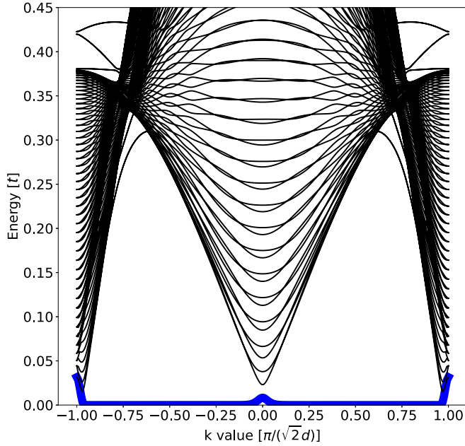
FIG. 5. The spectrum of eigenvalues E_{lk} for a N_x = 100 wide slab at average hole doping \delta = 0.05 . The spectrum contains 100 bands at positive energies within the first Brillouin zone k \in (-\pi d/\sqrt{2}, \pi d/\sqrt{2}] . Note that the spectrum is cut at an energy 0.450. The thick blue line is the lowest positive eigenvalue and contains the zero-energy Andreev bound states.
