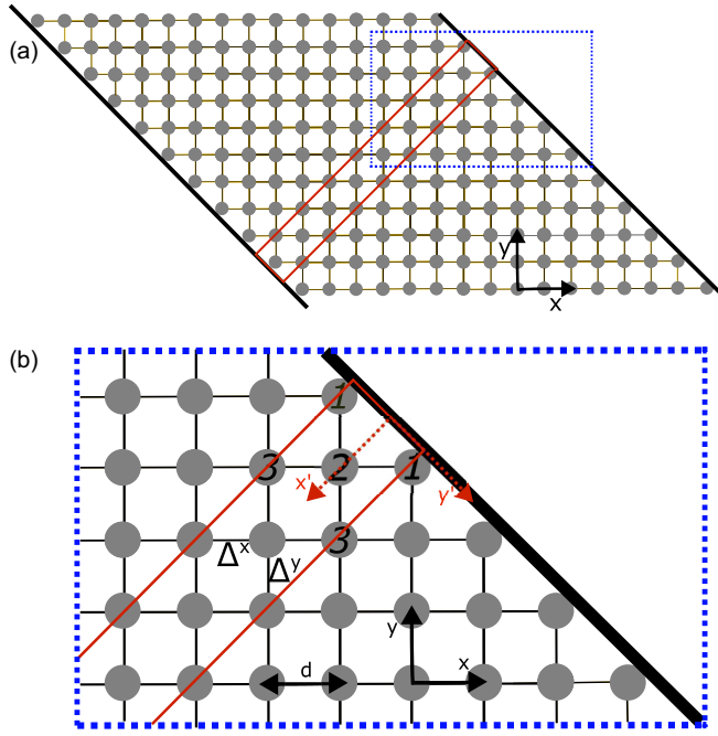
FIG. 1. (a) Square lattice with lattice constant d cut into a slab with [110] edges. There is translational invariance along the edge tangent. The red lines mark the unit cell, the gray disks sites, and the x - and y -axes are the crystal axes. Lines between sites represent the links in either x - or y -direction. (b) The area enclosed by dotted blue lines in (a), including the right [110] edge with edge tangent y' and edge normal x' . The sites are a = 1, 2, 3 etc. dependent on distance from the edge measured along x' . Note that between sites a and a + 1 there will be one link in the y -direction and one in the x -direction. The pairing amplitudes \Delta_{a,a+1}^x and \Delta_{a,a+1}^y , laying on links, are computed independently in order to allow for d -wave and extended s -wave symmetries.
