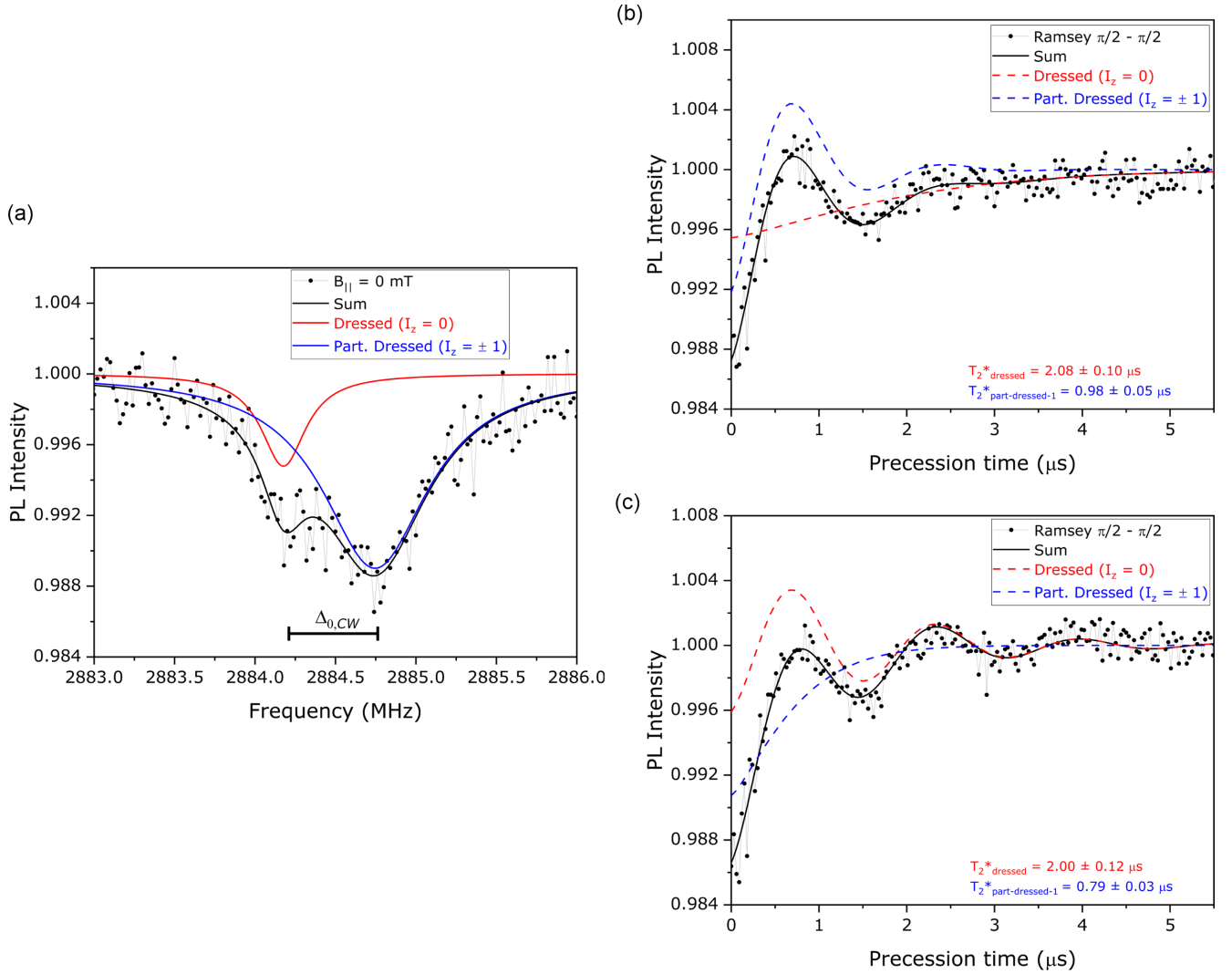
FIG. 2. Experimental results for B_{||} = 0 , corresponding to point A of Fig. 1(a) upper branch: (a) optically detected magnetic resonance spectra. Two resonances are present. The blue solid line fits the one related to the two degenerate partially dressed states ( I_z = \pm 1 ), following a Lorentzian distribution. The red solid line fits the one related to the dressed state ( I_z = 0 ). The black curve corresponds to the sum of the two Lorentzians. (b) Free induction decay relaxation for a microwave of frequency \nu_{MW} = \nu_{A,dres} on resonance with the dressed state I_z = 0 . The decay is fitted as the contribution of a pure stretched exponential, red dashed curve, relative to the dressed state I_z = 0 , and an oscillating stretched exponential, blue dashed curve, related to the partially dressed states with I_z = \pm 1 . (c) Free induction decay relaxation for a microwave of frequency \nu_{MW} = \nu_{A,p-dres1} on resonance with the degenerate partially dressed states I_z = \pm 1 . The decay is fitted as the contribution of a pure stretched exponential, blue dashed curve, related to the partially dressed states with I_z = \pm 1 , and an oscillating stretched exponential, red dashed curve, related to the dressed state with I_z = 0 . In all curves, the value of the stretched exponential is fixed to p = 1.28 , derived from the fit of the decaying of strong-axial-field states (see Supplemental Material [44]).
