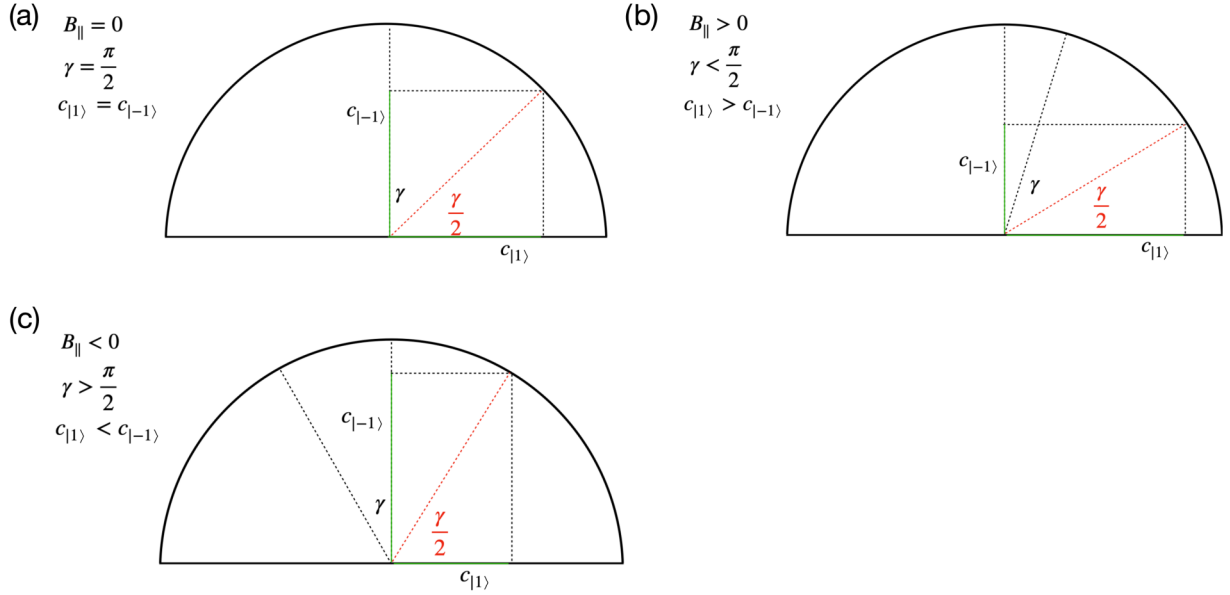
FIG. 4. Different balance of coefficients of high field for (a) B_{||} = 0 , (b) B_{||} > 0 , (c) B_{||} < 0 . For B_{||} = 0 the coefficients are equal, and the superposition is balanced, corresponding to dressed states. For B_{||} > 0 the superposition is unbalanced toward |S_z = +1\rangle and for B_{||} < 0 the superposition is unbalanced toward |S_z = -1\rangle .
