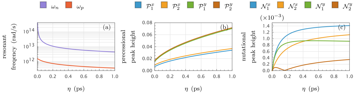
FIG. 3. (a) Resonant frequencies as a function of \eta . Curves are computed from Eq. (16). A logarithmic scale is used on the frequency axis, and low-frequency regions are omitted for clarity. (b) and (c) show the dependence of peak heights on \eta for precession and nutation, respectively. Curves are computed from Eqs. (19) and (18). The parameters used are the same as in Fig. 2.
