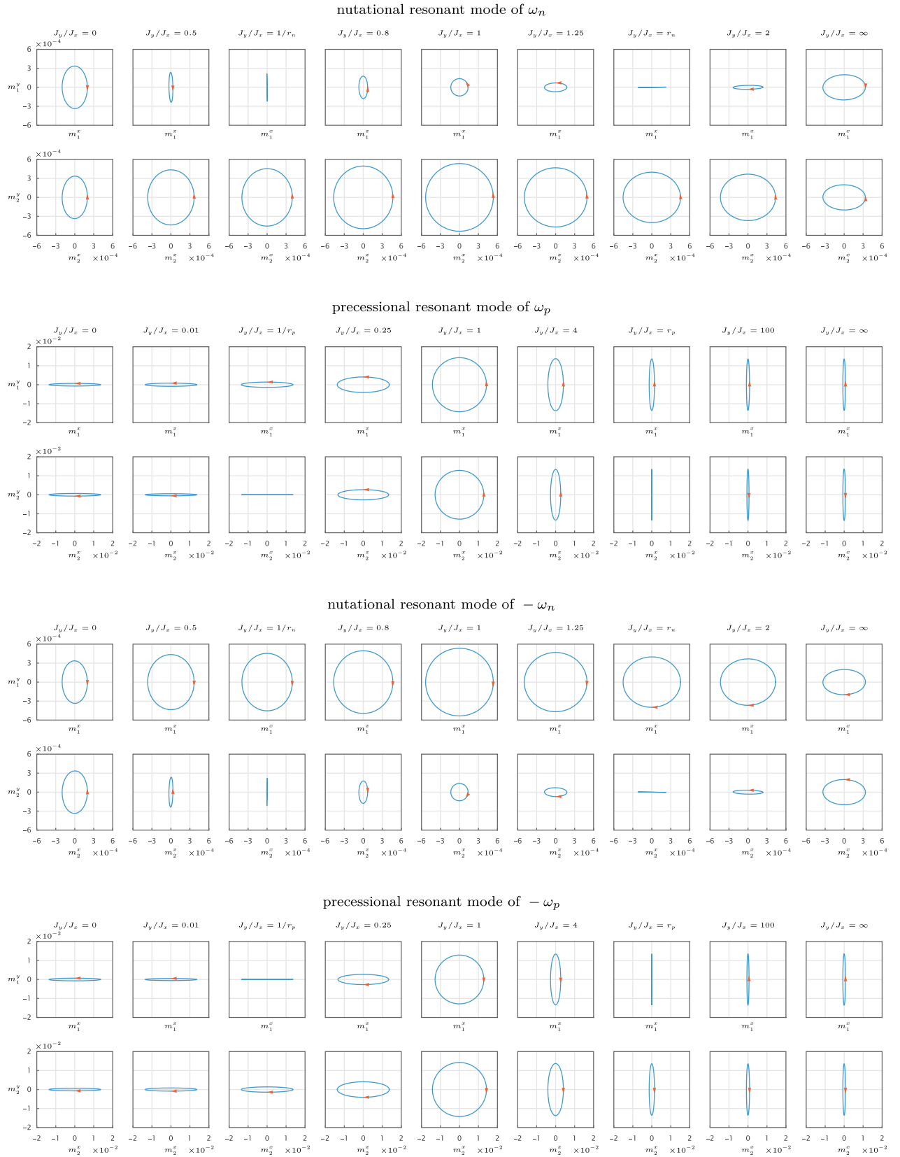
FIG. 5. Polarization and handedness of resonant modes for four branches ( \pm\omega_p , \pm\omega_n ) at various values of J_y/J_x . The inertial relaxation time is set to \eta = 100 fs, yielding r_n = 1.6855 and r_p = 19.4488 from Eq. (23). In each panel, the horizontal and vertical axes correspond to m_x and m_y components, respectively. Curves represent the magnetization orbits, and arrows indicate the sense of rotation. In the panels in columns 1–5, J_x = 1 GA/m 2 , and J_y is calculated by the ratio J_y/J_x . In the panels in columns 6–9, J_y = 1 GA/m 2 , and J_x is calculated by the ratio.
