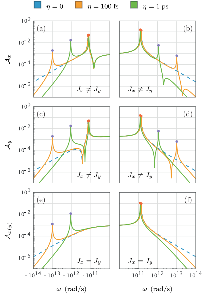
FIG. 7. FM resonant spectra for various values of \eta . (a)–(d) Under elliptically polarized SOTs ( J_x \neq J_y ), both precessional and nutational FM resonances are excited on the positive- and negative-frequency ranges. (e) and (f) For circular polarization ( J_x = J_y ), the nutational mode is observed at negative frequencies, whereas the precessional mode appears at positive frequencies. Noninertial spectra at \eta = 0 are shown with dashed curves. The precessional resonance is shifted by finite spin inertia ( \eta > 0 ), and additional nutational resonances are induced (solid curves). Peaks labeled with red (purple) points correspond to precessional (nutational) resonances. To enhance visibility, both axes are shown on a logarithmic scale, and low-frequency regions are omitted. All spectra are calculated from Eq. (B8) using the following parameters: \omega_K = 0.14 THz, \alpha = 0.01 , \beta = 0.02 , \rho \approx 0.13 Hz/(A/m 2 ); in (a)–(d), J_x = 1 GA/m 2 , J_y = 2 GA/m 2 ; in (e) and (f), J_x = J_y = 1 GA/m 2 . For comparison with AFMs, the values of \omega_K and \rho are chosen to match those in Fig. 2.
