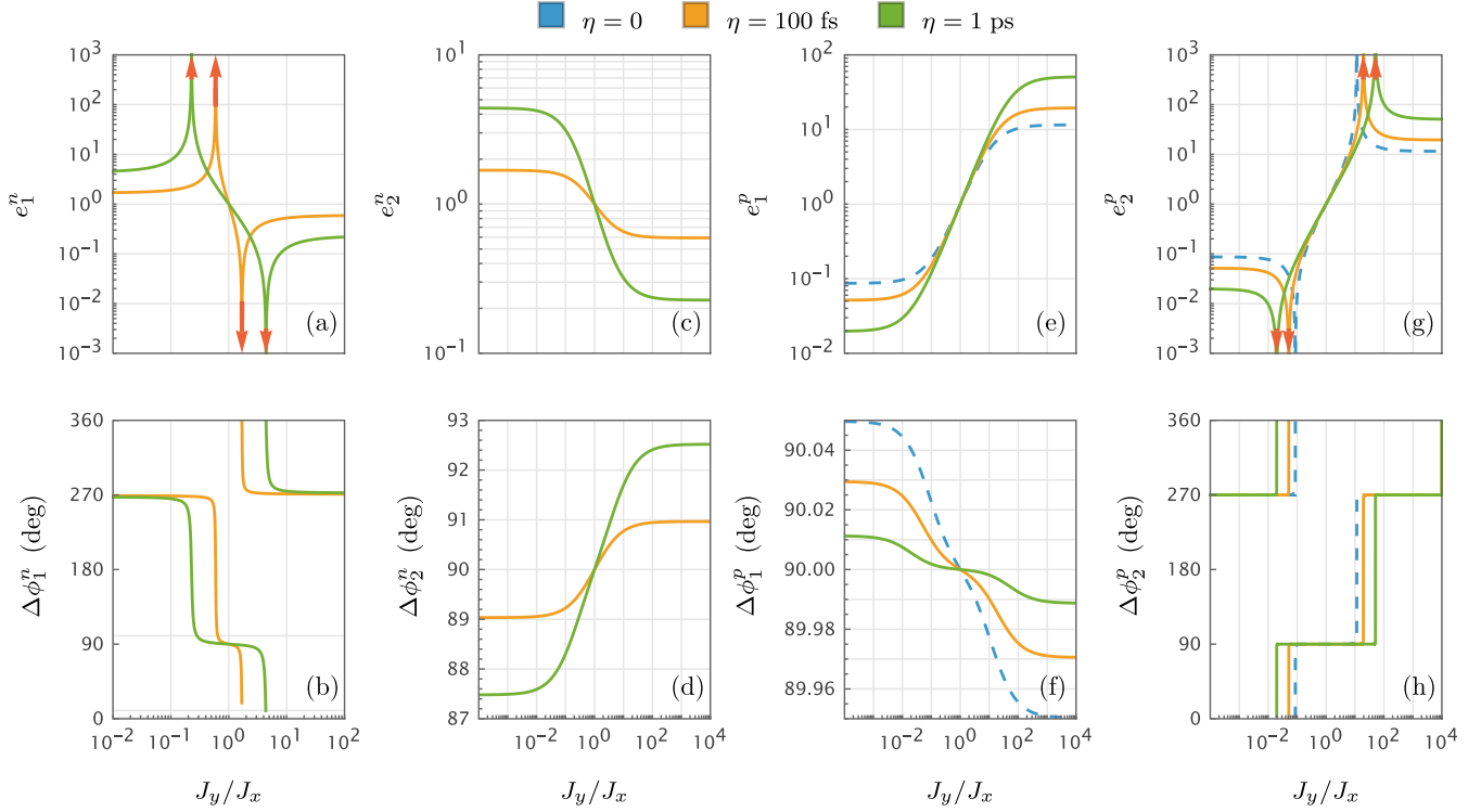
FIG. 4. Ellipticity (upper row) and intercomponent phase difference (lower row) as functions of the current ratio J_y/J_x at positive frequencies for several values of \eta . Panels (a)–(d) present the nutational modes of sublattices 1 and 2, while (e)–(h) display the corresponding precessional modes. The curves are calculated with Eqs. (21), (22), and (24). Parameters are identical to those in Fig. 2.
