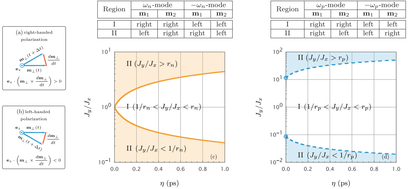
FIG. 6. (a) and (b) Definition of handedness. Phase diagrams illustrating the polarization of \mathbf{m}_{1,2} as functions of J_y/J_x and \eta for (c) nutational and (d) precessional resonances. In (c), the upper (lower) boundary is given by J_y/J_x = r_n ( J_y/J_x = 1/r_n ); in (d), by J_y/J_x = r_p ( J_y/J_x = 1/r_p ). The upper and lower circles in (d) mark J_y/J_x = \sqrt{(2\omega_E + \omega_K)/\omega_K} and \sqrt{\omega_K/(2\omega_E + \omega_K)} , respectively. The tables above (c) and (d) contain the handedness in different regions for nutational and precessional resonant modes, respectively.
