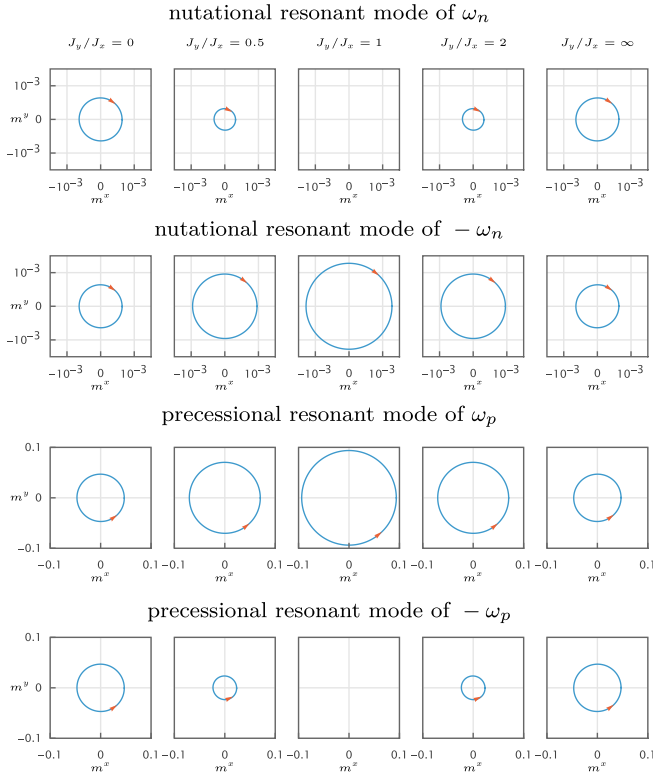
FIG. 8. Polarization and handedness of resonant modes for various ratios J_y/J_x . The inertial relaxation time is set to \eta = 100 fs. In each panel, the horizontal and vertical axes represent the m_x and m_y components, respectively. The curves depict the trajectories of the magnetization vector, and the arrows indicate the sense of rotation. In the panels in columns 1–3, J_x = 1 GA/m 2 , and J_y is calculated by the ratio J_y/J_x . In the panels in columns 4–5, J_y = 1 GA/m 2 , and J_x is calculated by the ratio.
