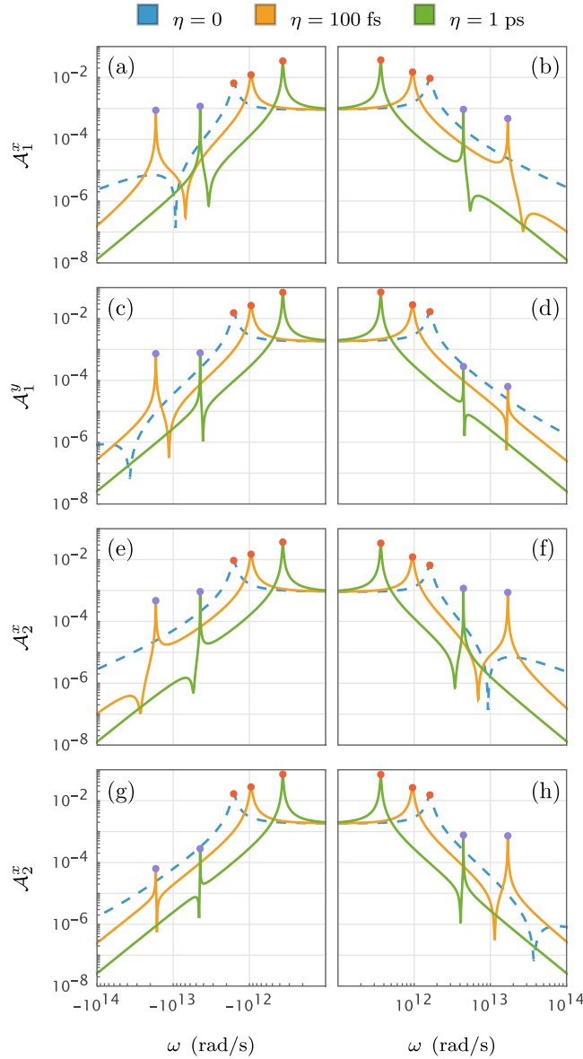
FIG. 2. AFM spectra without spin inertia exhibit the single precessional resonance (dashed lines, \eta = 0 ). Finite spin inertia \eta > 0 shifts the precessional AFM resonance and induces the additional nutational resonances (solid lines). Peaks labeled with red (purple) points correspond to precessional (nutational) resonances. Both axes are shown on a logarithmic scale; low-frequency parts are omitted for clarity. Curves are evaluated from Eq. (10) using \omega_E = 9.25 THz, \omega_K = 0.14 THz, \alpha = 0.01 , \beta = 0.02 , J_x = 1 GA/m 2 , J_y = 2 GA/m 2 , and \rho \approx 0.13 Hz/(A/m 2 ). The values of \omega_E , \omega_K , and \rho are derived from the magnetic parameters of MnF 2 [52] for a film thickness d = 3 nm and SOT efficiency \xi = 0.32 .
