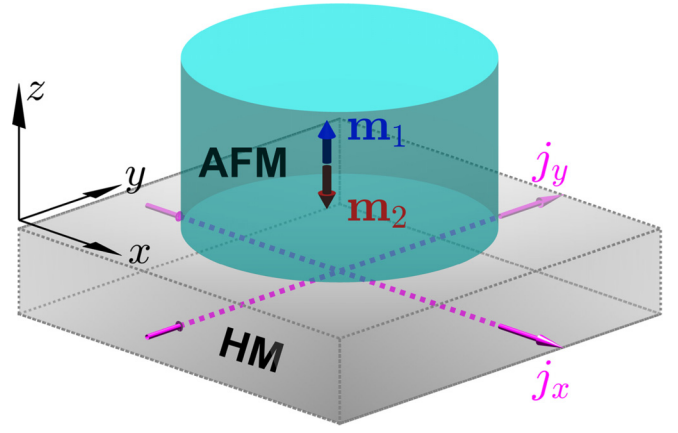
FIG. 1. Schematic diagram of model.
