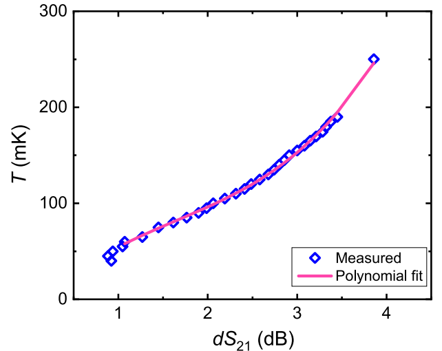
FIG. 8. S_{21} \rightarrow T_{\text{gr}} calibration plot. The calibration curve is the best polynomial fit T_{\text{gr}}(S_{21}) = a(dS_{21})^3 + b(dS_{21})^2 + c(dS_{21}) + d , where dS_{21} = S_{21} - 15.6 \text{ dB} , a = 0.00715 , b = -0.03543 , c = 0.09803 , and d = -0.01529 . The polynomial fit was performed over temperatures in the range from 60 to 200 mK to exclude the region where the sample temperature saturates.
