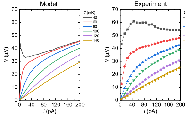
FIG. 15. Calculated (left) and measured (right; symbols correspond to experimental data, and lines are guides for the eye) V - I curves at different fridge temperatures T .
