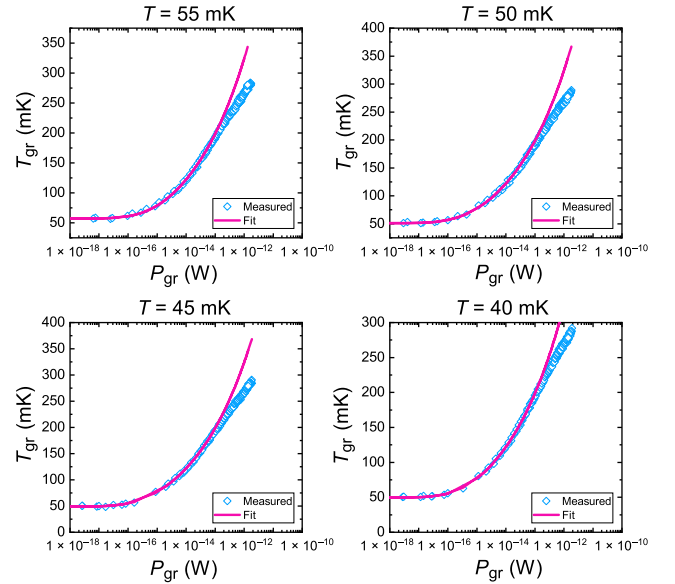
FIG. 12. Experimental data for T_{\text{gr}} vs P_{\text{gr}} (diamonds) for fridge temperatures T = 55, 50, 45 , and 40 mK. Solid lines are fits to T_{\text{gr}} = ((P_{\text{gr}}/A) + T_0^5)^{1/5} with the same A = 3.5 \times 10^{-10} W for all plots. The saturation temperatures T_0 = \lim_{P_{\text{gr}} \rightarrow 0} T_{\text{gr}} extracted from the fits are 57, 51, 49, and 49.5 mK.
