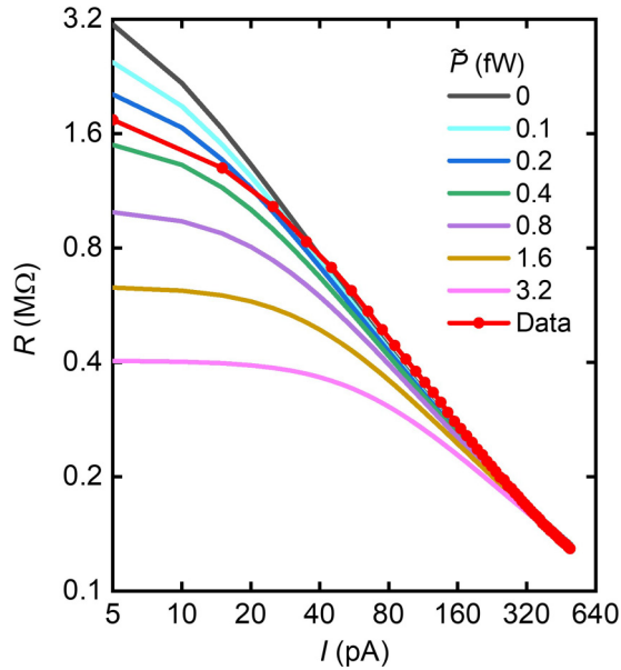
FIG. 16. Effect of the background heating power \tilde{P} on the shape of graphene resistance R(I) = V/I vs bias current curves. A set of theoretical curves and experimental data (red circles correspond to experimental data, and the red curve is a guide for the eye) at the fridge temperature of 60 mK.
