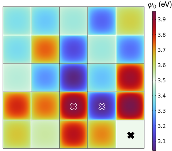
FIG. 5. Surface generated with 10 \times 10 \mu\text{m}^2 work function patch squares. These work functions were randomized to have \bar{\phi}_0 = 3.5 \text{ eV} with a \pm 0.5 \text{ eV} variation. The patches marked with X show the locations of the potential energy barriers along a straight line perpendicular to the surface shown in Fig. 6. The potential energies are smoothed near square edges to avoid ES field singularities in the simulations.
