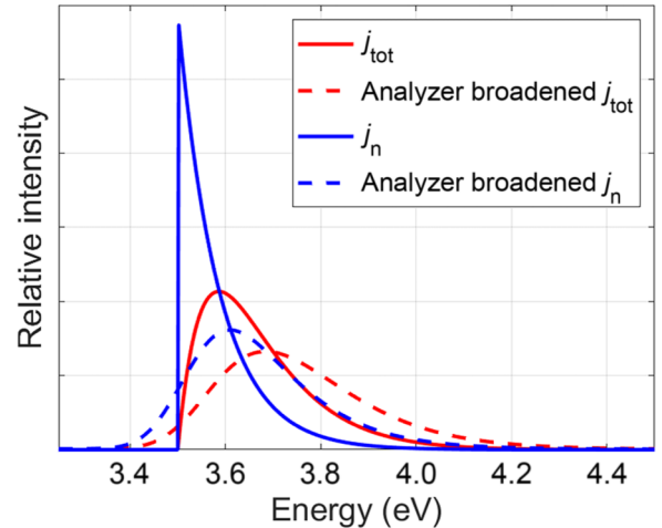
FIG. 3. Comparison of a typical NED and TED from j_n and j_{\text{tot}} , respectively, in Eq. (1) shown by the solid curves. The dashed curves show an emulated analyzer broadening effect at a pass energy of 5 eV on both j_n and j_{\text{tot}} , demonstrating how different a real measurement may appear compared with Eq. (1).
