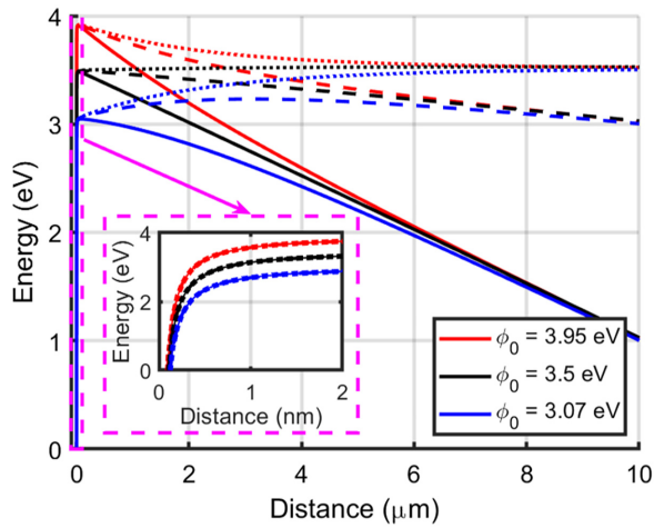
FIG. 6. Potential energy barriers for select points on the generated surface in Fig. 5. The barriers are observed at the exact center of a 3.95 eV (red X ), 3.5 eV (black X ), and 3.07 eV (blue X ) patch. The dotted, dashed, and solid lines represent external ES fields of 0.1, 50, and 250 kV/m, respectively. The inset shows an enlarged distance region of 0 to 2 nm from the emitter surface. This region is relevant to electron tunneling in field emitters. Here, the potential energy barrier does not bend downward for any of the external ES fields, indicating that these barriers are far too wide for electron tunneling.
