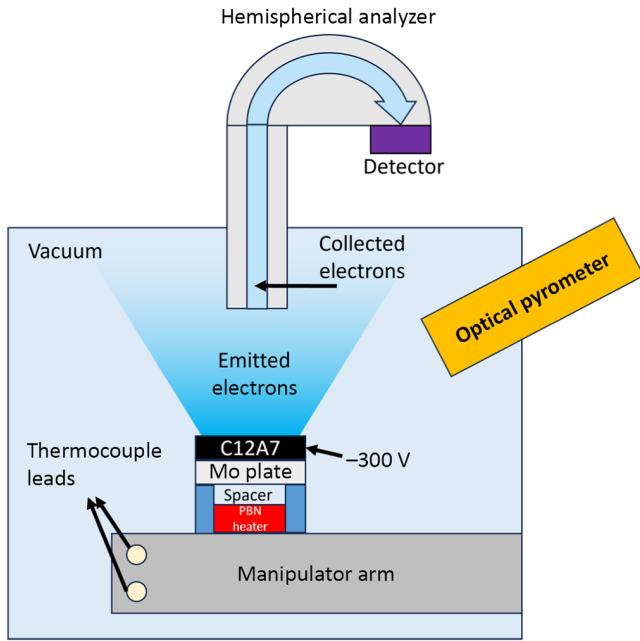
FIG. 1. Experimental setup for measuring the thermal electron emission energy distributions.
