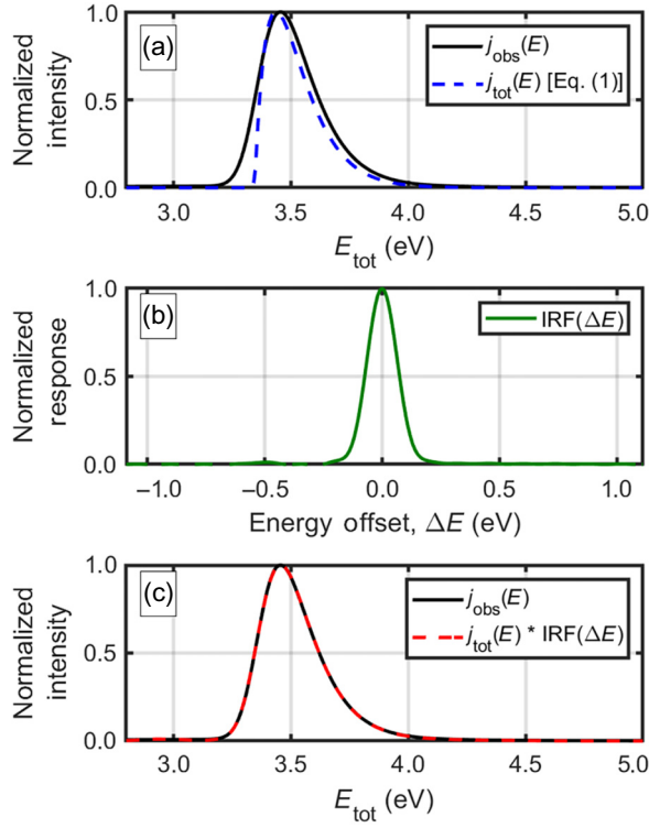
FIG. 7. (a) Normalized intensity versus E_{\text{tot}} for the measured j_{\text{obs}}(E) distribution and theoretical j_{\text{tot}}(E) distribution from Eq. (1). To generate the j_{\text{tot}}(E) distribution, the measured temperature and work function of 1062 K and 3.35 eV were used, respectively. Due to the instrumental resolution constraints, the measured curve was not quite reproduced. (b) Representation of the instrumental resolution function \text{IRF}(\Delta E) . (c) Normalized intensity versus E_{\text{tot}} for the measured j_{\text{obs}}(E) distribution and the convolution of the j_{\text{tot}}(E) * \text{IRF}(\Delta E) distributions. After considering the instrument resolution here, the measured curve was nearly perfectly recreated. All the spectra are normalized to their peak intensity.
