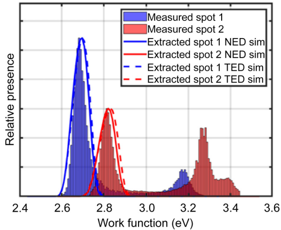
FIG. 14. Comparison of the measured and extracted work function distributions. An MC algorithm predicted ThEEDs from the measured work function distribution, then a steepest-descent algorithm extracted a predicted work function distribution from the ThEEDs. The solid and dashed lines represent the MC algorithm determining normal and total energy ThEEDs, respectively. Excellent work function distribution agreement exists regardless of normal or total energy MC simulations.
