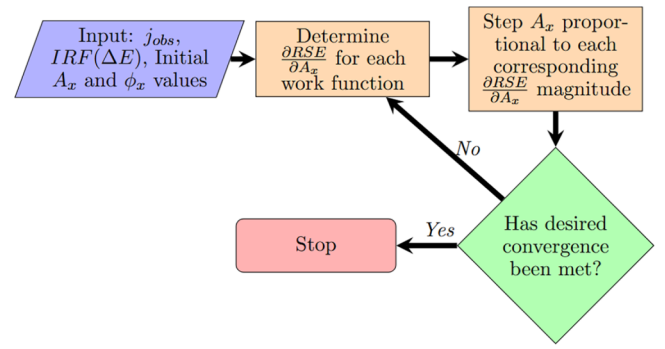
FIG. 4. Flowchart for determining the work function distribution via the steepest-descent algorithm.
