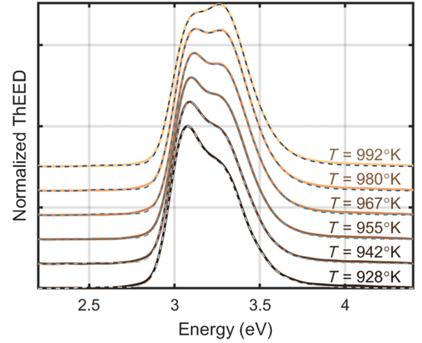
FIG. 8. Measured normalized and offset ThEED curves of \text{C12A7:e}^- at various temperatures, as shown by the solid lines. Dashed lines represent the fits generated with j_{\text{sum}}(E) * S(E) . A unique j_{\text{sum}}(E) was generated for each curve. All the spectra are normalized to their peak intensity.
