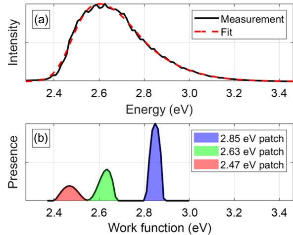
FIG. 16. (a) ThEED measurement and fit from the steepest-descent algorithm. (b) Extracted work functions from the ThEED measured at the location marked in Fig. 15(b). The three peaks are each shaded and the two lower work function patches, which dominate the emission, are in excellent agreement with the measured distinct work function patch values.
