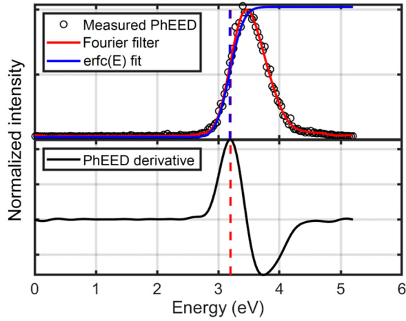
FIG. 2. (top) Measured PhEED, frequency-filtered PhEED, and complementary error function fit. Vertical dashed lines represent the extracted work functions using the derivative and complementary error function methods, with red and blue lines, respectively. (bottom) Numerical PhEED energy derivative after applying a frequency filter. The maximum of this curve (represented by a vertical red line) represents the inflection point of the PhEED and, therefore, the work function. All the curves are normalized to their peak intensity.
