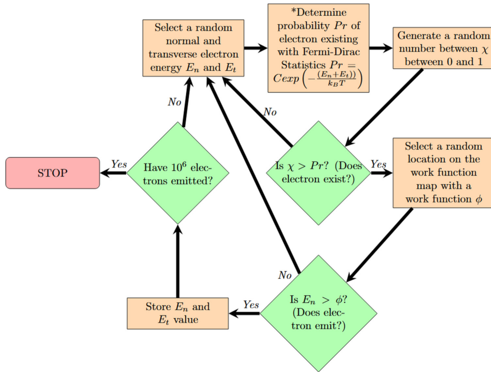
FIG. 12. Flowchart for the Monte Carlo algorithm to determine the ThEED. *The parameter C is a normalization constant C = \exp(\varphi_{\min}/k_B T) , where \varphi_{\min} is the minimum work function on the surface. Normalizing the Fermi-Dirac statistics and setting the minimum possible generated value of E_n to \varphi_{\min} greatly enhance the simulation speed.
