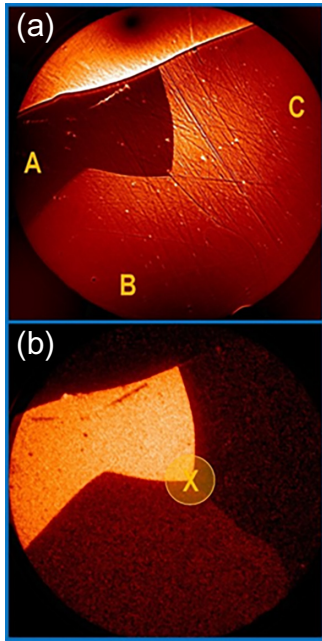
FIG. 15. (a) LEEM image of the Mayenite surface showing three distinct patches (i.e., A, B, and C) of a unique work function. (b) ThEEM image of the same location, where a low work function patch dominates electron emission. Locations marked on (b) represent the region where a ThEED was measured, capturing emission from all three patches simultaneously; the temperature is 784 K, the field-of-view is 88 \mu\text{m} , and the external extracting ES field is 5250 kV/m. Rendering histograms are linear in (a) and logarithmic in (b).
