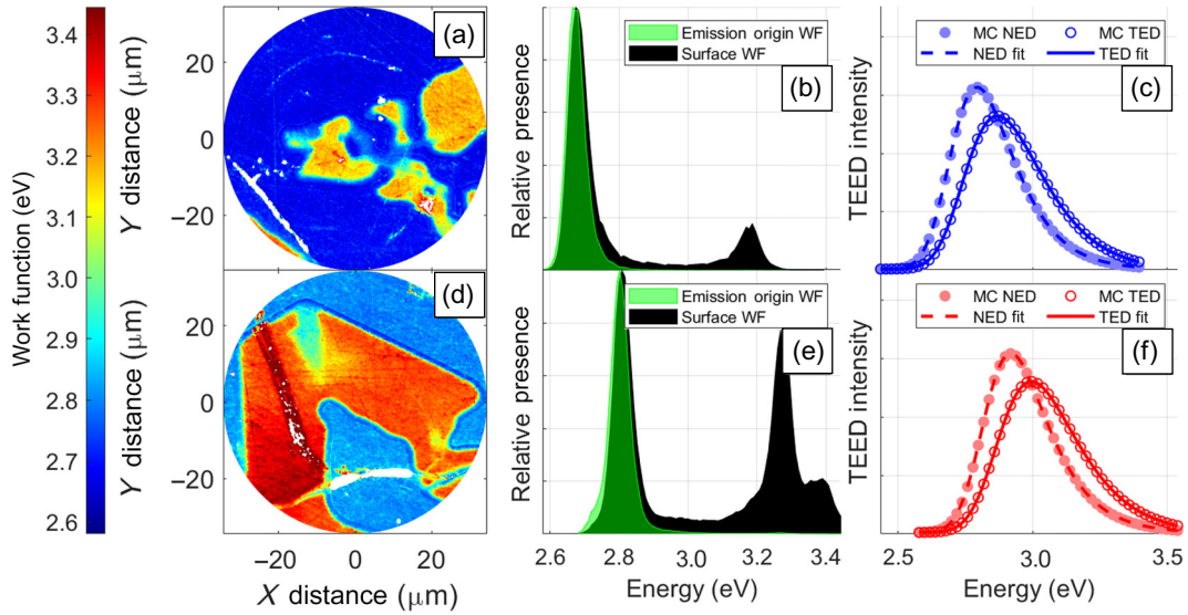
FIG. 13. (a),(d) Measured work function maps determined using PEEM at two arbitrary locations on the sample surface. (b),(e) Work function histograms of the corresponding work function map, shown in black. Histogram of the work function origin of the emitted electrons in the MC simulation, shown in green. (c),(f) ThEEDs simulated with the MC simulation and then fit with the work function extraction method. All ThEEDs are broadened using the \text{IRF}(\Delta E) distribution, as shown in Fig. 7, prior to extracting work functions.
