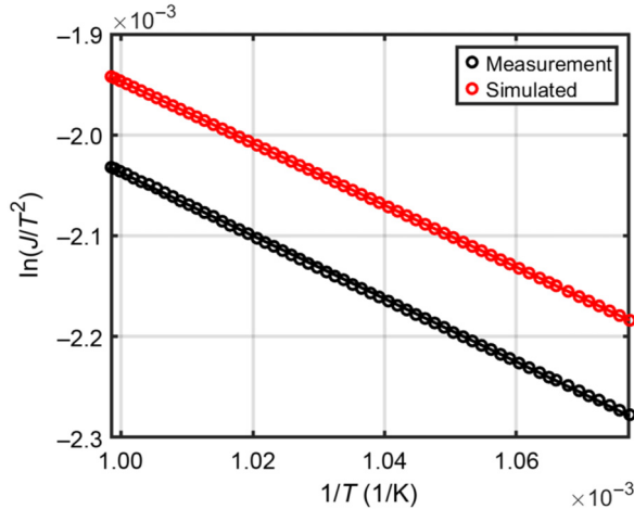
FIG. 11. Richardson–Laue–Dushman plot to extract the work function from the experimental and simulated data via a linear fit. The work functions of 3.12 eV and 3.08 eV are extracted for the measured and simulated data, respectively, with a coefficient of determination r^2 > 0.999 .
