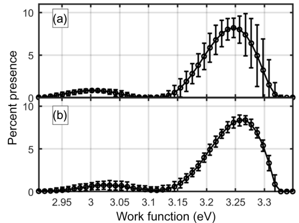
FIG. 10. Mean relative work function presence extracted from the ThEEDs using the steepest-descent algorithm, as outlined in Fig. 4. The error bars represent a 95% confidence interval. (a) Average extracted work values across all the temperatures. (b) Average extracted work values at T = 1002 \text{ K} using randomized initial values of A_x over 100 iterations.
