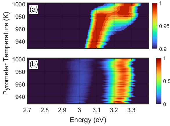
FIG. 9. (a) Measured normalized ThEED curve intensities at various temperatures. (b) Normalized A_x distribution (the relative surface presence of each work function) for each temperature. For both contours, the data across each temperature row is normalized with respect to its maximum value.
