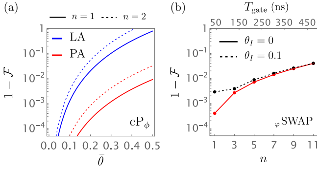
FIG. 3. Two-qubit gates. (a) Infiltrity 1 - \mathcal{F} of the cP_\phi gate for the planar arrangement (PA) and linear arrangement (LA) of dots [see Figs. 1(a) and 1(b)] against \bar{\theta} . We consider a pulse duration of t = n\tau_I/\alpha_H with n = 1 (solid lines) and n = 2 (dashed lines). Specifically, for PA (LA) with pulse amplitude J_I/h = 20 MHz, the gate time is T_{\text{gate}} = \tau_I/\alpha_H \approx 37 ns ( T_{\text{gate}} \approx 150 ns). (b) Infiltrity of the \varphi SWAP gate against n for \theta_I = 0 (red) and \theta_I = 0.1 \approx 6^\circ (black). We simulate the full time evolution of the six spins in PA using \bar{J}/h = 1 GHz, \bar{\theta} = 0.5 , and J_I/h = 20 MHz.
