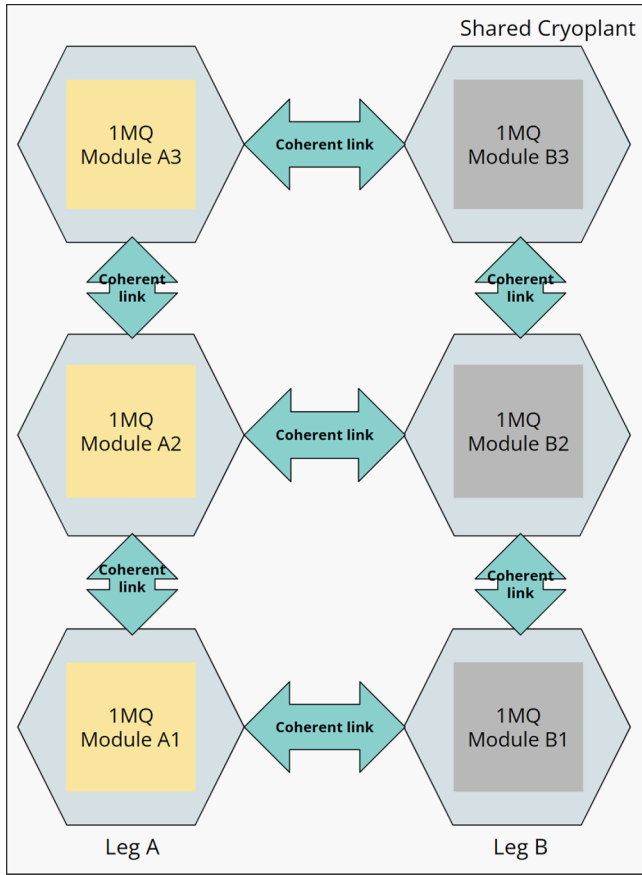
FIG. 3. The high-level macroarchitecture consists of two sets of 10^6 -physical-qubit (1MQ) modules arranged like the legs of a ladder. Following the example in Fig. 2, each leg contains three modules, each following the layout of Fig. 1(bottom). Portions of the algorithm are divided and executed solely within modules on the same leg, where intramodule interactions with high connectivity and short gate times dominate. All modules communicate via width- d “coherent interconnects” (or links) at a lower rate and with reduced connectivity, used only for graph preparation (vertical interconnects) and state handover (horizontal interconnects).
