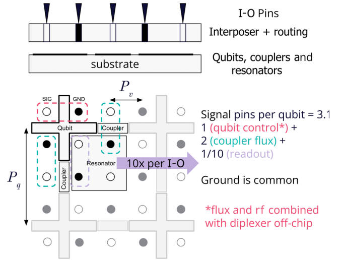
FIG. 4. A schematic layout for the required components to couple superconducting qubits through tunable couplers in a surface-code layout. In this example, we demonstrate the essential components: qubits, readout resonators, tunable couplers, and I-O pins. Each physical qubit and coupler requires a single control line, their respective ground connections, and an additional rf line for multiplexed readout shared among ten qubits. This limits the physical-qubit pitch to match that of the signal lines. A qubit-to-qubit pitch at three times the signal-line pitch has sufficient I-O pins to accommodate this.
