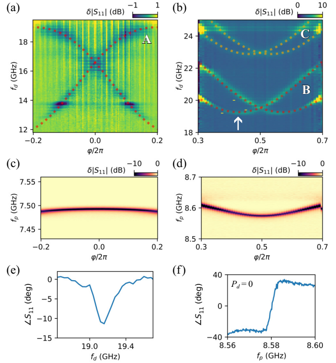
FIG. 5. (a)–(d) Spectroscopy data obtained for (a),(c) device 3 at V_g = 1.498 V and (b),(d) device 2 at V_g = 2.44 V. (a),(b) In two-tone spectra, bundles of SQPTs are observed, with crossings at the degeneracy points. SQPT frequency fits are denoted by the dotted lines and labeled as A, B, and C. The fit parameters are listed in Table II. (c),(d) The corresponding single-tone spectra. (e) Phase of the reflected signal as a function of the drive frequency at a minimum of the lower SQPT [see the white arrow in panel (b)]. (f) The corresponding resonator response when the system is not excited.
