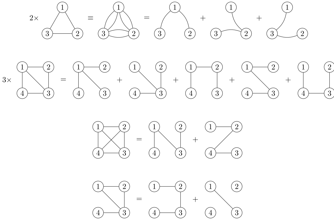
FIG. 4. Spanning-tree packings in different graphs with equal edge weights (bipartite QKD rates) for all edges (note that this assumption is used only for illustrative purposes in the figures, while the general theory is formulated for arbitrary bipartite key rates r_e , see the text). Here it is convenient to think that an edge in a graph represents a bipartite key with a fixed length L . Then multiple QKD sessions (factors in front of the graphs) give multiple edges between the same vertices. One spanning tree corresponds to a conference-key of the length L . Thus, the problem is to find an optimal spanning-tree packing , i.e., a set of edge-disjoint spanning trees such that the ratio of the number of edge-disjoint spanning trees to the number of QKD sessions (per each bipartite link) is maximal. The last term in the last line is not a spanning tree, but a leftover edge. The operations \times and + are understood here in the sense of edge multiplicities in a multigraph. If all bipartite secret key rates are equal to one ( L = 1 ), then the conference-key rates r_{\text{conf}} for these examples (from top to bottom) are 3/2 , 5/3 , 2 , and 1 . We found the spanning-tree packings here using the heuristic described in Appendix A.
