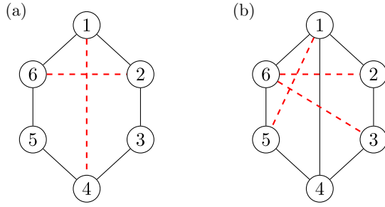
FIG. 7. Network optimization. All edges here correspond to bipartite secret key rate r = 1 . (a) The initial ringlike network of six nodes gives the conference-key rate r_{\text{conf}} = 6/5 . If we are allowed to add one link (edge), then which of the two links marked as red-dashed edges is it better to choose? The optimal choice is to add the link (1, 4). (b) If we are allowed to add one more link, which of the three marked options is optimal? The optimal solution is to add (2, 6) or (3, 6) because the addition of the link (1, 5) leads to a triangle bottleneck structure, see the text.
