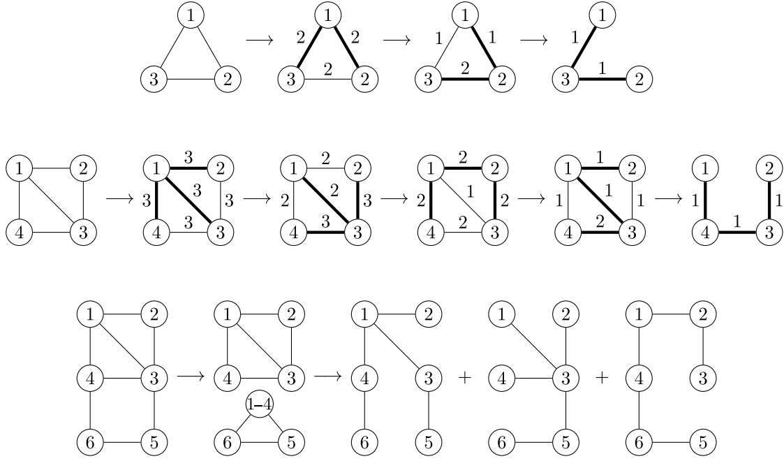
FIG. 8. Illustration of the Basic algorithm (first two lines) and the General algorithm (the last line) of finding an optimal spanning-tree packing. All edge weights are equal to one. For the graphs in the first two lines, condition (17) is satisfied and we know that we can generate a certain number of conference-key bits in N - 1 round ( N - 1 is the number of vertices). We assign new weights N - 1 to each edge and then, in each step, choose a spanning tree with possibly maximal weights of edges (bold edges). Each use of the edge reduce its weight by one. The graph in the third line violates Eq. (19) for I = \{5, 6\} , so, the conference-key rate cannot exceed that for the graph where the rest vertices \{1, 2, 3, 4\} are contracted into one, i.e., the triangle graph, or 3/2 . Then we solve the spanning-tree-packing problem for both the contracted graph and the subgraph induced by the vertices \{1, 2, 3, 4\} and merge the spanning trees of these graphs according to the edge correspondence between the original graph and the contracted one. We obtained three spanning trees with not more than two uses of each edge, which gives the rate 3/2 . Choices of other spanning trees lead to other optimal solutions.
