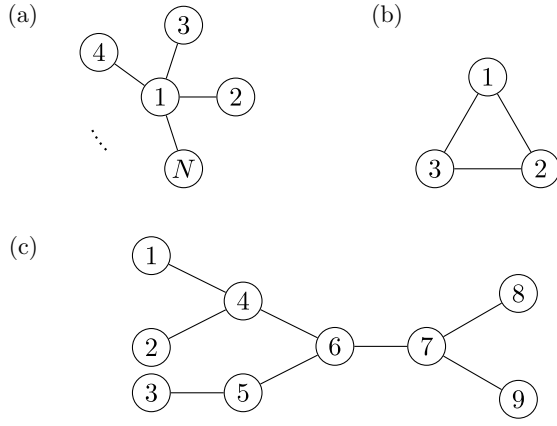
FIG. 1. Examples of QKD networks: a star network with N users (a), the triangle network (b), and a tree network (c). Vertices (nodes) of a graph represent users and edges represent (bipartite) QKD links between them.
