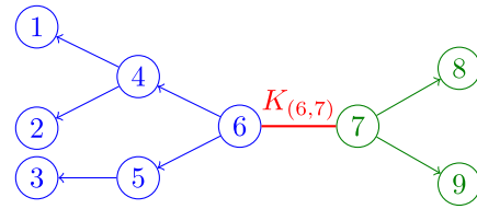
FIG. 3. Conference-key propagation for the tree graph from Fig. 1(c). The users agree whose bipartite key will be the conference-key. Here: K_{(6,7)} . Removal of the corresponding edge breaks the graph into two nonconnected subgraphs (subtrees, depicted by the blue and green colors) with vertices 6 and 7 as the roots. The propagation of the key K_{(6,7)} proceeds according to the arrows.
