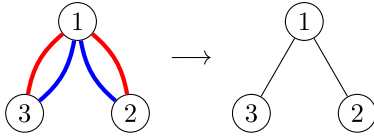
FIG. 9. If we ignore the edge multiplicities of a multigraph, several spanning trees of it (here: two spanning trees of the multigraph, which are depicted by red and blue) can map into the same spanning tree of the resulting graph.
