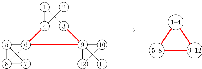
FIG. 6. A contraction of a graph indicating a more complex bottleneck structure, than a connection between two subgraphs (like in Fig. 5): a triangle bottleneck structure. If all bipartite QKD links have the rate r_e = 1 and, thus, the triangle network with bipartite key rates r_e = 1 has conference-key rate 3/2 (see Fig. 4), then, for the left graph, r_{\text{conf}} \leq 3/2 .
