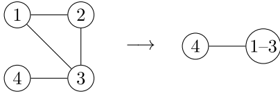
FIG. 5. A contraction of the graph from Fig. 4 (last row) indicating a bottleneck structure, which restricts the conference-key rate: connection of node 4 to the rest of the network. The conference-key rate in the original graph cannot be larger than the conference (bipartite) key rate in the contracted graph. If the link (3, 4) has the rate r_{(3,4)} = 1 , then, for the left graph, r_{\text{conf}} \leq 1 .
