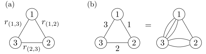
FIG. 2. Quantum QKD network as a weighted graph with bipartite secret key rates r_e as the weights (a). In the case of integer weights, it can be alternatively represented as the multigraph where edge multiplicities correspond to the weights (b).
