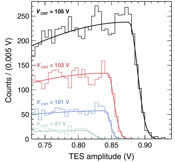
FIG. 6. Example fits, for four different values of V_{\text{CNT}} , of the high-amplitude peak with the asymmetric Gaussian function.
