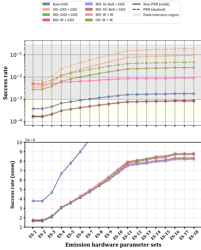
FIG. 9. GHZ success rates ( P_{\text{succ}} ) for varying hardware parameters from ES-1 to ES-18 for coherence times of T = 10^6 , physical error rates of p = 10^{-3} tuned at \alpha = 0.025 (except OD-GHZ that is biased for \alpha = 0.5 ).
