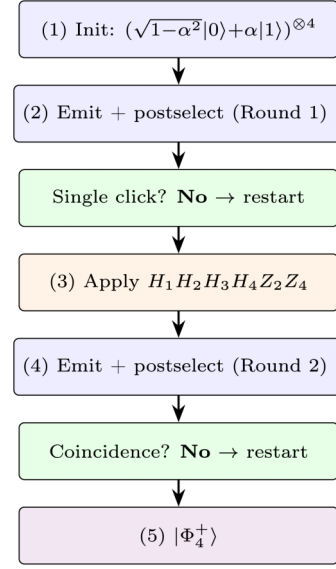
FIG. 5. OD-W protocol operational summary (RUS). (1) Initialize and emit photons into the beam-splitter network. (2) Single-detector click heralds the raw W state. (3) Local H_1 H_2 H_3 H_4 Z_2 Z_4 rotations expose the GHZ component. (4) Second emission round with two-detector coincidence postselection. (5) Output approximates |\Phi_4^+\rangle ; unlike OD-GHZ, a perfect GHZ state requires \alpha \rightarrow 0 as W -state noise terms cannot be fully suppressed. A failed postselection at either round triggers a full restart.
