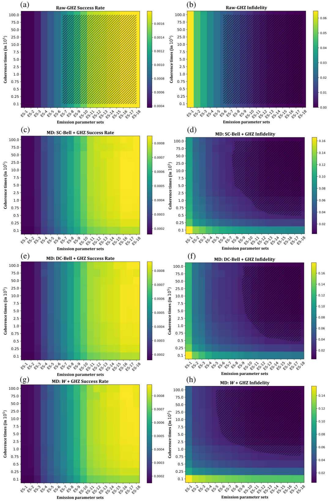
FIG. 14. (1 of 2) Heatmaps for varying coherence times and hardware parameters with PNR detectors, physical error rate of p = 10^{-3} , and \alpha = 0.025 . OD-GHZ is evaluated at \alpha = 0.5 . Fault-tolerance regions are shaded with black lines.
