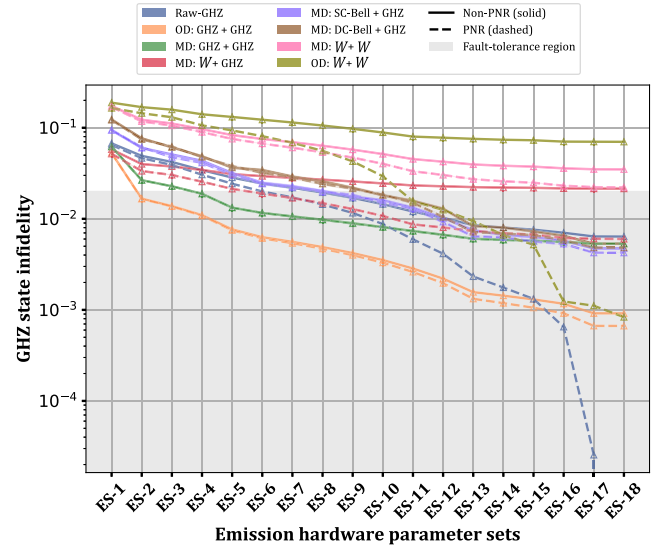
FIG. 10. GHZ state infidelity ( 1 - F_{\text{GHZ}} ) for varying hardware parameters from ES-1 to ES-18 for coherence times of T = 10^6 , physical error rates of p = 10^{-3} tuned at \alpha = 0.025 (except OD-GHZ that is biased for \alpha = 0.5 ).
