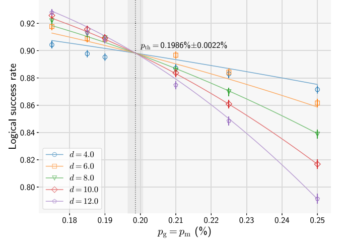
FIG. 12. Threshold plot for OD-GHZ protocol with non-PNR detectors for circuit-level noise. The threshold plot is evaluated for T = 10^6 , and hardware parameter set ES-5, leading to a toric surface code threshold of p_{th} = 0.1986\% \pm 0.0022\% .
