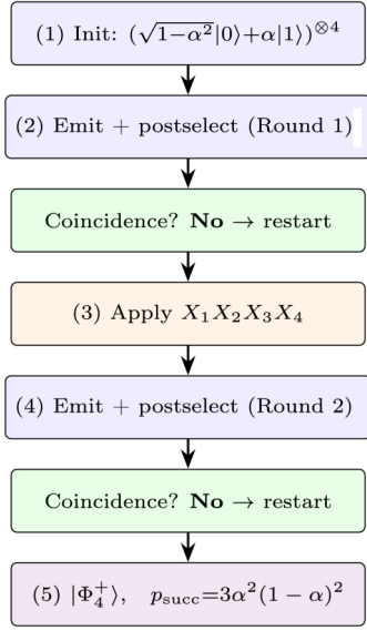
FIG. 4. OD-GHZ protocol operational summary (RUS). (1) All four communication qubits are initialized and excited to emit photons into the beam-splitter network. (2) A two-detector coincidence postselection heralds the raw-GHZ state [Eq. (17)]. (3) Local X_1 X_2 X_3 X_4 gates map the noise terms into the low-excitation subspace [Eq. (21)]. (4) A second emission round is executed on the same device without reconfiguration. (5) Postselection on the same coincidence pattern heralds the purified GHZ state |\Phi_4^+\rangle with p_{\text{succ}} = 3\alpha^2(1-\alpha)^2 . A failed coincidence at either round triggers a full restart.
