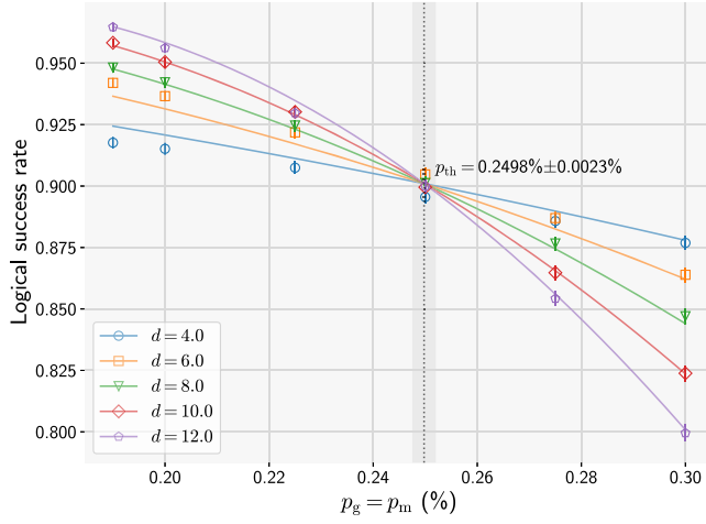
FIG. 11. Threshold plot for OD-GHZ protocol with PNR detectors for circuit-level noise. The threshold plot is evaluated for T = 10^6 , and hardware parameter set ES-2, leading to a toric surface code threshold of p_{th} = 0.2498\% \pm 0.0023\% .
