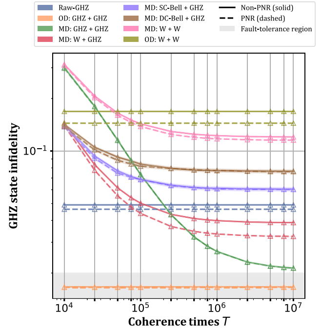
FIG. 8. GHZ state infidelity ( 1 - F_{\text{GHZ}} ) for varying coherence times ( T = T_{\text{link}}^{\text{dec}} = T_{\text{idle}}^{\text{dec}} ) for the ES-2 hardware parameter set, physical error rate of p = 10^{-3} , tuned at \alpha = 0.025 .
