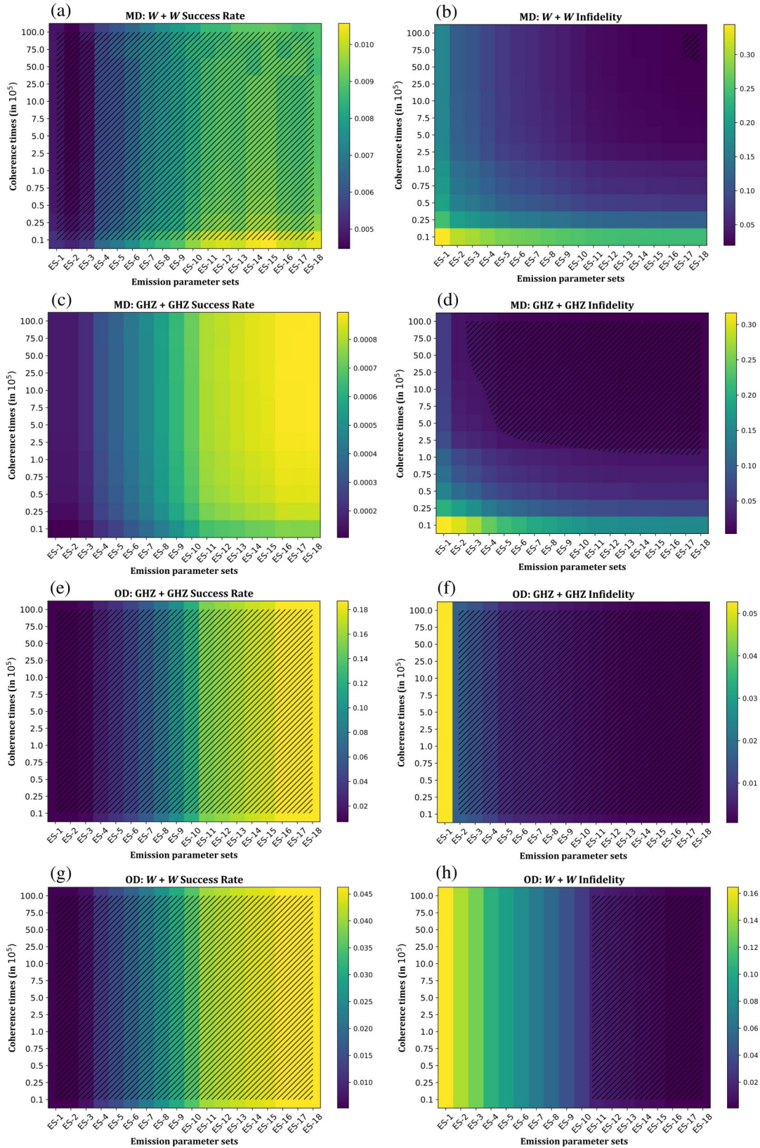
FIG. 15. (2 of 2) Heatmaps for varying coherence times and hardware parameters with PNR detectors, physical error rate of p = 10^{-3} , and \alpha = 0.025 . OD-GHZ is evaluated at \alpha = 0.5 . Fault-tolerance regions are shaded with black lines.
