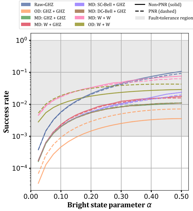
FIG. 7. Success rates for GHZ state ( P_{\text{succ}} ) for varying bright-state parameter ( \alpha ) for ES-2 hardware parameter set, coherence times T = 10^6 , and physical error rate of p = 10^{-3} .
