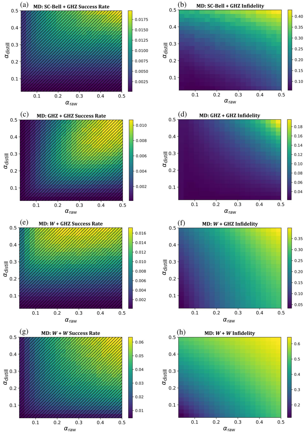
FIG. 13. Bright-state parameter trade-off for protocols with distinct \alpha for base state and distilling state, with PNR detectors. Evaluated with coherence times of T = 10^6 , hardware parameter set ES-2, and physical error rates of p = 10^{-3} . Fault-tolerance regions are shaded with black lines.
