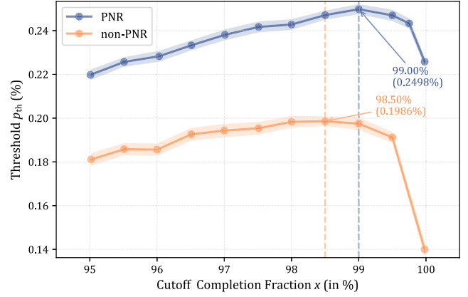
FIG. 16. Code threshold versus cutoff completion fraction for the OD-GHZ protocol under PNR (blue) and non-PNR (orange) detection. Optimal thresholds p_{\text{th}}^{\text{PNR}} = 0.2498\% and p_{\text{th}}^{\text{non-PNR}} = 0.1986\% are attained at x = 99.00\% and x = 98.50\% (marked by dashed lines), respectively. The decline beyond the optimal completion fraction reflects the dominance of decoherence accumulation on idle qubits over gains in syndrome information, establishing the necessity for precise cutoff optimization in distributed surface code.
