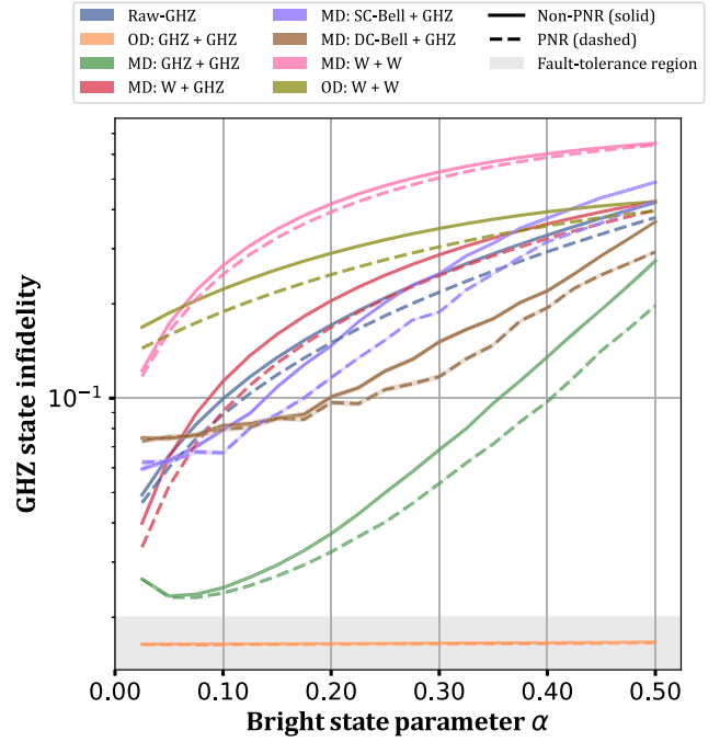
FIG. 6. GHZ state infidelity ( 1 - F_{\text{GHZ}} ) for varying bright-state parameter ( \alpha ) for ES-2 hardware parameter set, coherence times T = 10^6 , and physical error rate of p = 10^{-3} .
