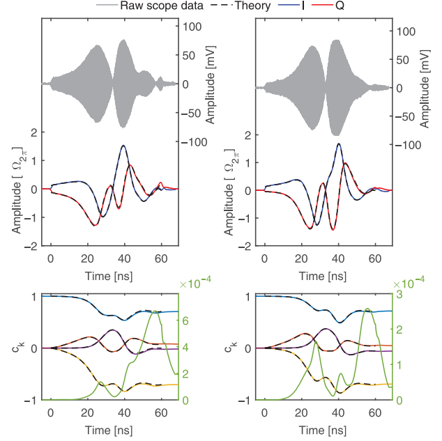
FIG. 8. Top: The real and imaginary part of the pulse \Omega(t)e^{iq(t)} (black dashed), along with the measured pulse (gray) and its demodulated real (blue) and imaginary (red) components. Bottom: The c_0 (blue), c_x (red), c_y (yellow), and c_z (purple) coefficients as a function of time for the scope data, along with the theory (black dashed). The right-hand scale, along with the solid green trace, shows the infidelity ( 1-F ) of the experimental trajectory with respect to the theoretical one. The left and right columns correspond to the qubit and qutrit optimized pulses, respectively.
