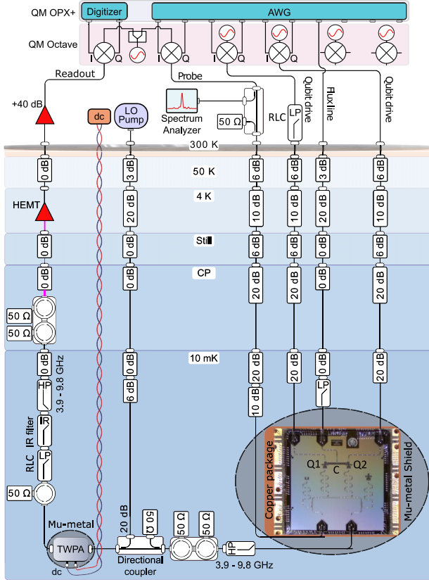
FIG. 7. A diagram of the experimental setup. Microscope image of the quantum processor with two transmon qubits. Only the left qubit ( Q_1 ) is used for the experiment. The sample is mounted inside a \mu -metal shield to protect it from stray magnetic fields.
