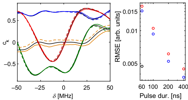
FIG. 2. Left: The experimentally obtained coefficients c_0 (blue), c_x (red), c_y (green), and c_z (yellow) for the pulse (solid) and its conjugate form (dashed) along with the theoretically expected value (solid black). Right: the RMSE between the theory and the experiment as a function of the pulse duration for the direct (red) and conjugated (blue) pulses, as well as the pulse optimized to suppress the interactions with the |2\rangle state (black).
