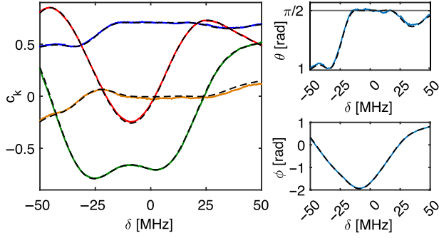
FIG. 3. Left: The experimentally obtained coefficients c_0 (blue), c_x (red), c_y (green), and c_z (yellow) for the pulse optimized to suppress the interactions with the |2\rangle state. Right: the azimuthal and polar rotation angles, \theta and \phi , top and bottom, respectively. The dashed black traces on all panels correspond to the theoretically expected behavior.
