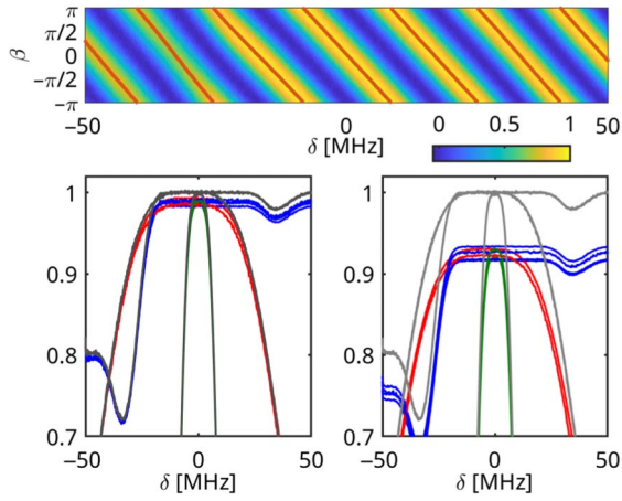
FIG. 13. Top: A 2D map of the excited state population as a function of the detuning \delta and relative pulse phase \beta . The red dots indicate the optimal \beta values for each \delta . Bottom: The measured excited state population as a function of \delta , using the optimal \beta values, for the robust (blue), DRAG (red), and rectangular (green) pulses before, and after correcting for the readout fidelity (gray). The left and right panels correspond to the averaged and single-shot readout schemes, respectively.
