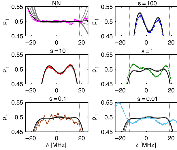
FIG. 14. The |0\rangle to |1\rangle transfer probability p_1 as a function of the detuning \delta for the NN and GRAPE pulses: Solid gray lines represent the full dataset. Colored dots indicate the experimental validation for a representative pulse, with the corresponding theoretical prediction denoted by the solid black trace.
