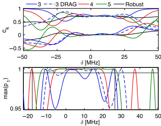
FIG. 16. Top: The c_0 and c_z traces for various composite pulse sequence lengths. The solid-colored lines correspond to the rectangular pulses, the black ones to the robust pulse, and the dashed-blue to a 3-pulse long sequence implemented with DRAG pulses. Bottom: The corresponding transition probabilities in a Ramsey-like experiment; the solid gray lines indicate the region in which the robust pulse has an efficiency greater than 0.995.
