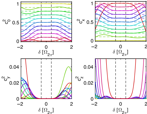
FIG. 5. The squared coefficients c_0^2 , c_x^2 , c_y^2 , and c_z^2 as a function of \delta for a detuning robust gateset. The rotation angles \theta satisfy \sin(\theta_k/2)^2 = k/10 from k = 0 (yellow) to k = 10 (red), with their target c_0^2 and c_x^2 indicated by the dashed horizontal lines. The dashed vertical lines indicate the training region.
