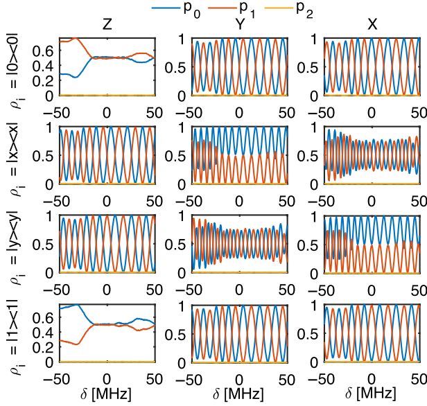
FIG. 9. The raw results of the frequency-dependent process tomography of the robust ( \frac{\pi}{2} ) pulse. Different rows correspond to different initial states, while the columns correspond to reading out the x , y , and z components of the density matrix. See the text for more details.
