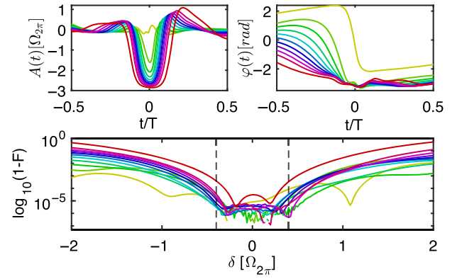
FIG. 6. The time-dependent amplitude A(t) (top left) and phase \varphi(t) (top right) required to realize the unitary operations presented in Fig. 5. The bottom panel shows the fidelity F of the operation as a function of detuning \delta (the dashed vertical lines indicate the training region). All traces are color-matched to the ones in Fig. 5.
