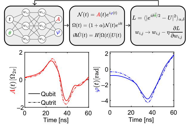
FIG. 1. Top: A schematic representation of the neural network approach: given some target rotation angle \theta and time t , the output of the network \mathcal{N} is perturbed by \alpha (amplitude) and \delta (detuning) to construct the complex drive field \Omega(t) , and the equation of motion is integrated to obtain the propagator U . Based on this, a loss L can be computed, which quantifies the discrepancy between the implemented and the target operation. Lastly, the weights of the neural network w_{i,j} are updated based on the gradients of L w.r.t w_{i,j} and a learning rate \eta . The cycle is repeated N times or until convergence. Bottom: The resulting pulse amplitude A(t) (left), shown in units of \Omega_{2\pi} = 2\pi/T_p where T_p is the pulse duration, and phase \varphi(t) (right) as a function of time, optimized for a true qubit (solid) and a qutrit (dashed-dotted).
