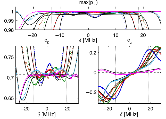
FIG. 15. Top: The QPT predicted \max(p_1) vs \delta for the NN pulse (magenta) and the GRAPE ones for s \in \{0.01, 0.1, 1, 10, 100\} (teal, brown, green, red, and blue, respectively). Bottom: the QPT extracted c_0 (left) and c_z (right) coefficients of the same set of pulses. The solid black traces correspond to the theoretically expected values, while the vertical dashed lines indicate the training region, and the horizontal ones show the target c_{0/z} values.
