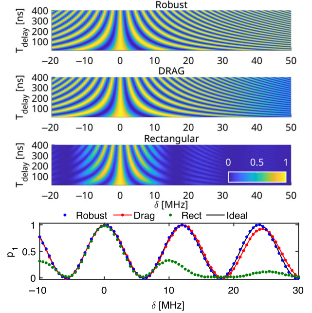
FIG. 12. Top: The Ramsey interference pattern measured for the robust, DRAG and rectangular pulses. Bottom: slices of the former as a function of detuning \delta for a fixed T_{\text{delay}} (colored symbols), along with the ideal response (solid black).
