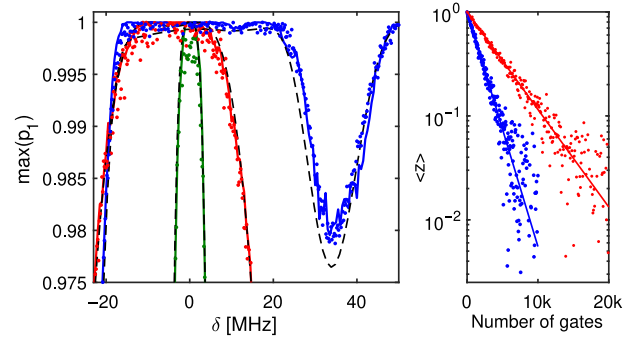
FIG. 4. Left: The maximum |0\rangle \rightarrow |1\rangle transfer efficiency as a function of detuning \delta for the robust (blue), DRAG (red) and rectangular (green) pulses. The dots correspond to directly measured values, the solid lines to the QPT inferred ones and the dashed black to the theoretical expectation. Right: The z component of the density as a function of the number of applied robust (blue) and DRAG (red) pulses.
