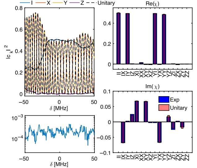
FIG. 10. Left: The diagonal elements of the experimental process matrix (solid, colored), along with that of the unitary fit (black, dashed), as a function of detuning \delta , along with their Frobenius distance (bottom). Right: The real (top) and imaginary (bottom) parts of the experimental and unitary process matrices at \delta = 0 .
