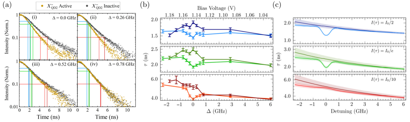
FIG. 2. Enhancement of emitter decay rate. (a) Comparison of the decay curves of the system with the QDs detuned by (i) \Delta = 0 , (ii) \Delta = 0.26 GHz, (iii) \Delta = 0.52 GHz, and (iv) \Delta = 0.78 GHz. Measurements are performed with (yellow) and without (black) optical gating of QD2. Colored lines indicate where the intensity drops below the thresholds used in (b),(c). (b) Detuning dependence of the decay rate with (lighter lines) and without (darker lines) gating of QD2. The results are plotted as the time taken for the emission intensity to drop below three threshold values: I_0/2 (blue), I_0/e (green), and I_0/10 (red). (c) Theoretical prediction of the results in (b). The shaded regions signify uncertainties in the model due to errors in the X_{\text{QD1}}^- lifetime estimation.
