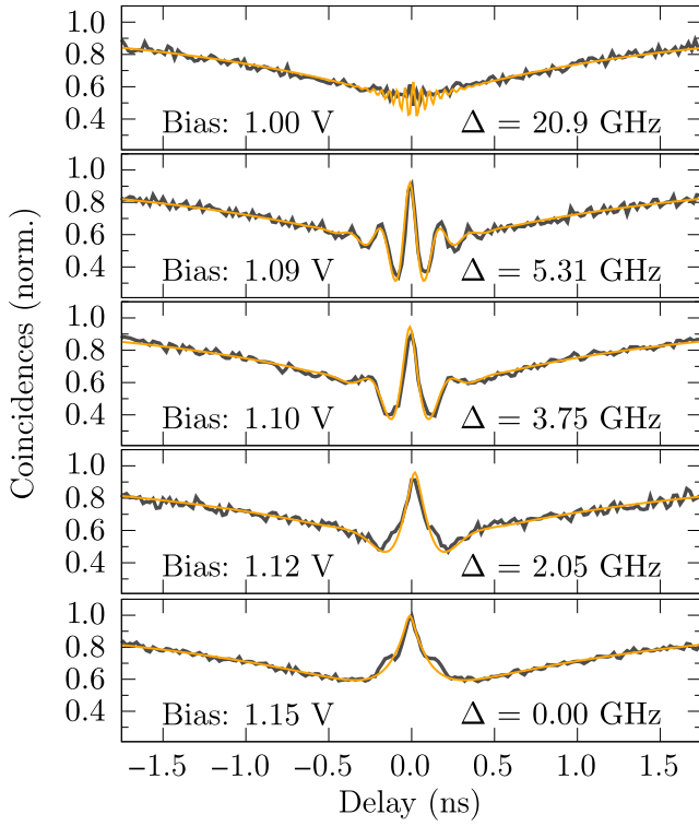
FIG. 3. Photon correlations. Autocorrelation function of emission collected from the end of the waveguide as a function of emitter-emitter detuning. The yellow lines are theoretical predictions of the measurements.
