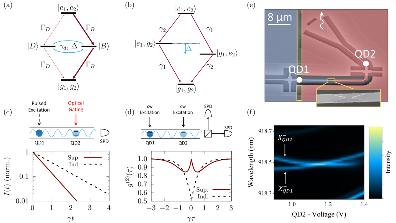
FIG. 1. Independent tuning of QDs and properties of superradiant emission. (a) Energy-level diagram of two resonant waveguide-coupled QDs. The states |e_1, e_2\rangle and |g_1, g_2\rangle describe both QDs in their excited and ground states, respectively. The spectral detuning and dephasing rate are labeled \Delta and \gamma_d . (b) Energy-level diagram of two independent quantum emitters. The state |e_1, g_2\rangle ( |g_1, e_2\rangle ) signifies that X_{QD1}^- ( X_{QD2}^- ) is excited, while the other QD is in the ground state. (c) Expected intensity decay for an ideal system of two superradiant (solid red line) or two independent (dashed black line) emitters given the depicted excitation scheme. (d) Expected autocorrelation function g^{(2)}(\tau) for a pair of superradiant (solid red line) or independent (dashed black line) emitters given the depicted excitation scheme. (e) SEM image of the waveguide device. The positions of the two QDs are marked by white spots. The red and blue coloring marks the area of the two diodes that control the two QDs. Yellow indicates the areas that are etched for electrical isolation. Inset: SEM of the isolation etch in the waveguide. (f) Emission spectrum of the X^- transitions of the two QDs, measured from the outcoupler of the device, as a function of the voltage applied to QD2 [red area in (e)].
