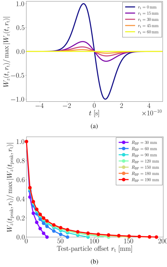
FIG. 5. Longitudinal BP space-charge wake potential: (a) normalized wake for a BP of radius 60 mm at various test-particle transverse offsets and (b) normalized transverse dependence of the wake potential for several BP radii R_{BP} .
