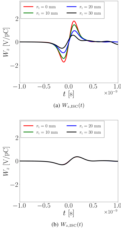
FIG. 9. Indirect space-charge longitudinal wake potential as a function of the test-particle transverse offset r_t for the stage-B5 multicell cavity (a) with Be windows and (b) without Be windows.
