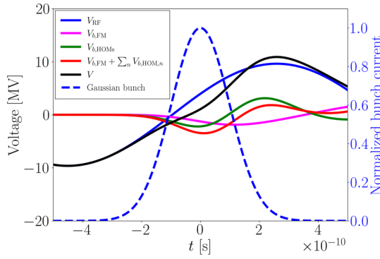
FIG. 13. Resonant beam-induced voltage decomposition and input rf voltage for the stage-B5 multicell cavity with Be windows. The normalized bunch current distribution is shown on the secondary axis.
