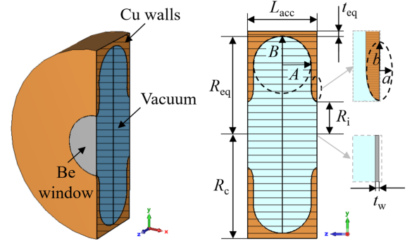
FIG. 2. Single-cell rf cavity design for muon cooling. The geometry is defined by the cavity accelerating length L_{acc} , equatorial radius R_{eq} , window radius R_i , window thickness t_w , and elliptical profile semiaxes A, B and a, b . The thin Be windows seal both irises of the cell. Reproduced from Ref. [25].
