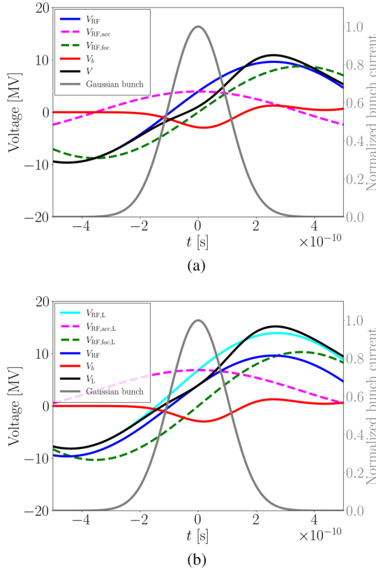
FIG. 14. Beam loading and local compensation in the stage-B5 multicell cavity. The total voltage experienced by the beam and the rf voltage components are shown (a) before and (b) after beam-loading compensation, alongside the beam-induced voltage from the FM and HOMs. The normalized bunch current distribution is illustrated on the secondary axis.
