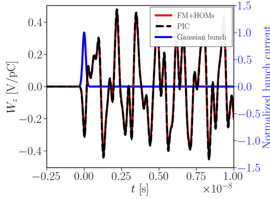
FIG. 12. Comparison of the on-axis longitudinal wake potential excited by a bunch with finite transverse size using the analytical eigenmode method and the PIC solver for the stage-B5 single-cell cavity with Be windows. The normalized bunch distribution is shown on the secondary axis.
