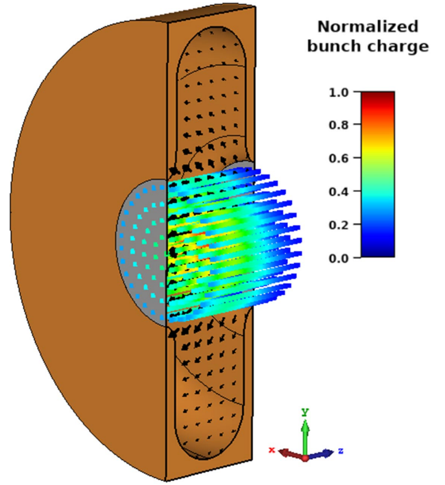
FIG. 11. Example setup for a PIC solver simulation. The particle source is released from the exterior wall of the Be window and traverses the cavity along its axis. The particle bunch excites electromagnetic fields within the cavity, with the black arrows representing the electric field vector.
