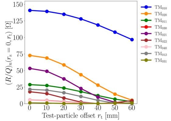
FIG. 7. Variation of the generalized (R/Q)_n of stage-B5 single-cell cavity as a function of test-particle transverse offset r_t for the relevant monopole modes.
