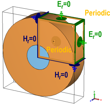
FIG. 4. Single-cell simulation setup with periodic boundary conditions and symmetry planes, used to model the field distribution of a multicell cavity without Be windows. The cavity utilizes the same elliptical profile as stage B5 in Fig. 2, with its equatorial radius R_{eq} retuned to maintain a resonant frequency of 704 MHz. Reproduced from Ref. [34].
