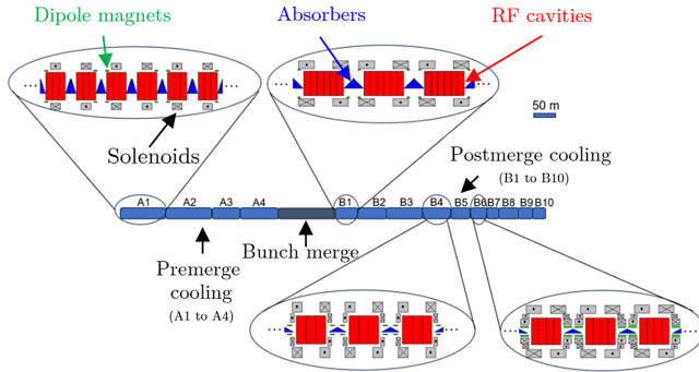
FIG. 1. Schematic of the rectilinear muon cooling channel. The channel is divided into a premerge section (stages A1–A4), a bunch merging system, and a postmerge section (stages B1–B10). Enlargement views illustrate the periodic lattice cell configurations, depicting the integration of radio-frequency (rf) cavities (red), absorbers (blue triangles), dipole magnets (green blocks), and focusing solenoids (gray blocks). Adapted from Ref. [7].
