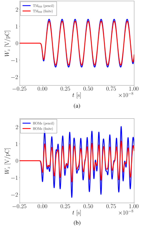
FIG. 10. (a) Longitudinal wake potentials of the FM and (b) the HOMs listed in Table V excited by a pencil beam (blue) and a finite beam with a transverse size of \sigma_t = 20 mm (red) in the stage-B5 multicell cavity with Be windows.
