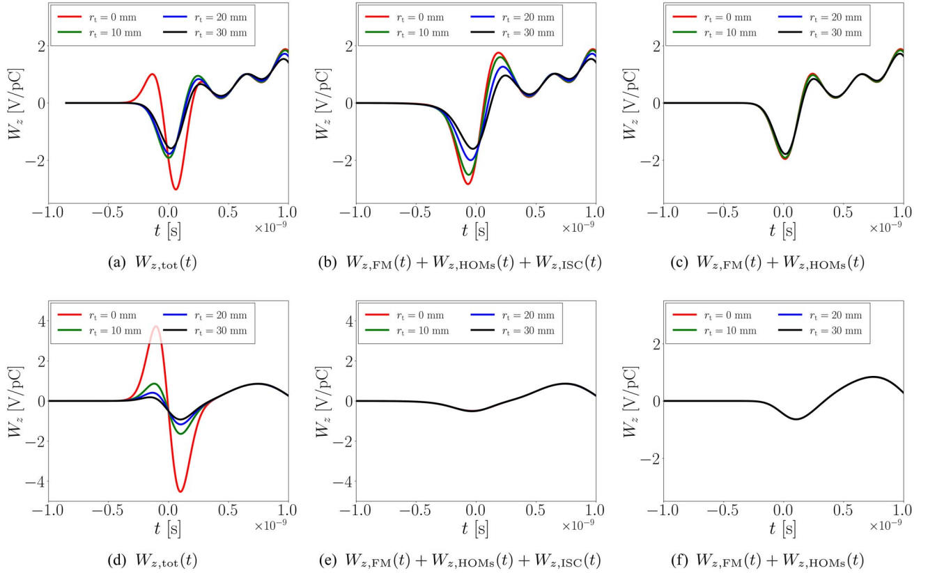
FIG. 8. Decomposition of the longitudinal wake potential as a function of the test-particle transverse offset r_t for the stage-B5 multicell cavity with Be windows (top) and without Be windows (bottom).
