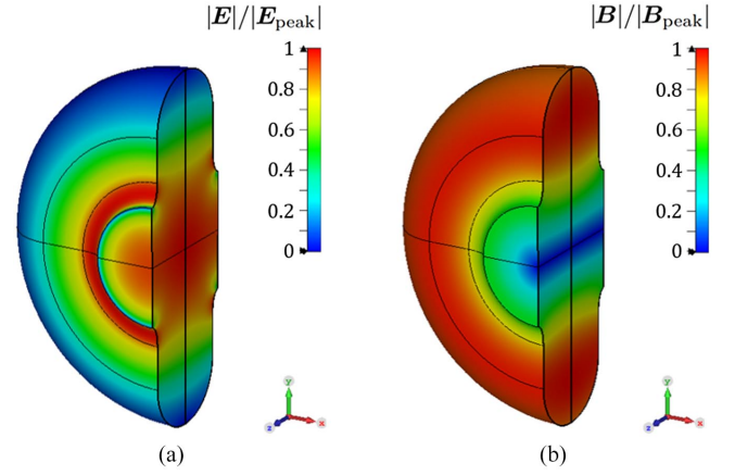
FIG. 3. (a) Normalized electric and (b) magnetic field distributions for the FM of the single-cell rf cavity with Be windows for muon cooling [25].
