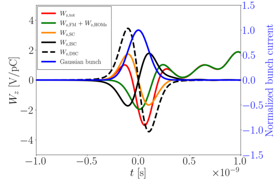
FIG. 6. Longitudinal wake potential decomposition for the stage-B5 multicell cavity with Be windows. The reconstructed eigenmode wake potential includes the first nine monopole modes up to 4 GHz. The normalized Gaussian bunch longitudinal profile is shown on the secondary axis.
