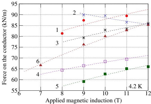
FIG. 13. Electromagnetic \vec{I} \times \vec{B} force sustained by individual layer witness samples at 4.2 K as a function of applied magnetic induction. Dashed lines indicate the calculation based on the fitting parameters from Table IV.
