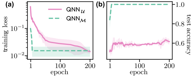
FIG. 3. Comparison of the training performance (a) and generalization (b) between the two GQML architectures, \text{QNN}_U and \text{QNN}_M . Both models were trained and tested on pairs of barcodes with 16 pixels each, corresponding to an 8-qubit quantum state for each input datum. Solid/dashed lines indicate the mean values across the ten trials, while the shaded region indicates the standard deviation.
