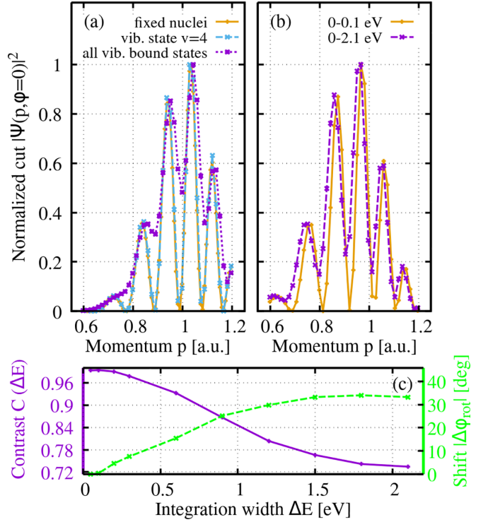
FIG. 4. Analysis of the contrast in PMDs, shown by cuts of PMDs along the positive p_x axis. (a) Comparison of the vibrational state v = 4 , fixed-nuclei results, and the integrated PMD of all vibrational bound states of \text{H}_2^+ . (b) Comparison of small and large integration regions of energies for the dissociation channel. (c) Contrast (purple line, left y axis) and relative shift of the rotation angle with respect to a small integration region (green dashed line, right y axis) as a function of the right boundary of the integration range for dissociation. Results are obtained for \tau_1 \approx 1.6 fs.
