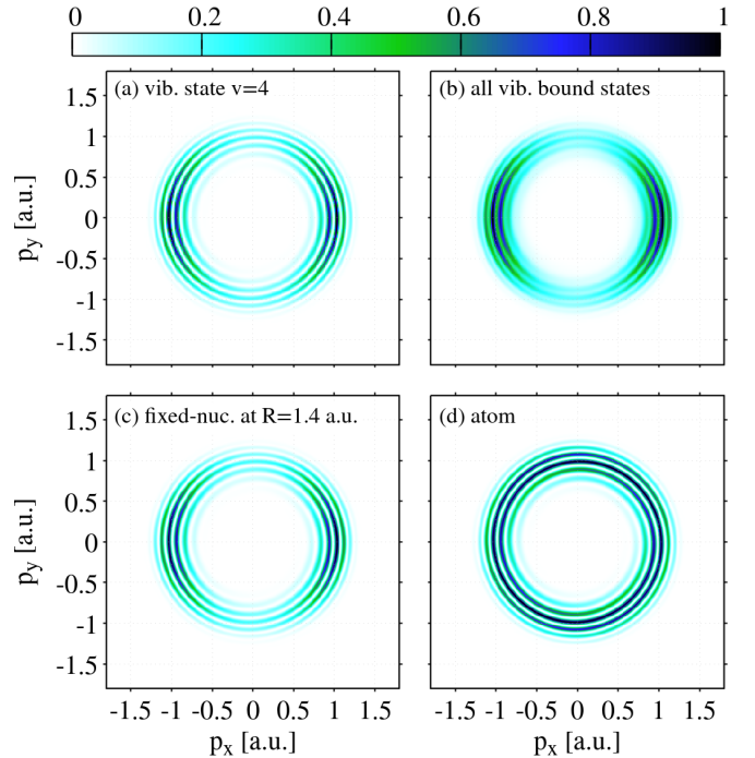
FIG. 3. Normalized photoelectron momentum distribution correlated with (a) the vibrational bound state v = 4 of \text{H}_2^+ , (b) the summed PMD of all vibrational bound states, (c) the result of a 2D fixed-nuclei TDSE simulation at an internuclear distance of R = 1.4 a.u., and (d) the 2D TDSE result for a model atom. All PMDs are obtained with an LRCP pulse and a time delay of 12 cycles ( \tau_1 \approx 1.6 fs).
