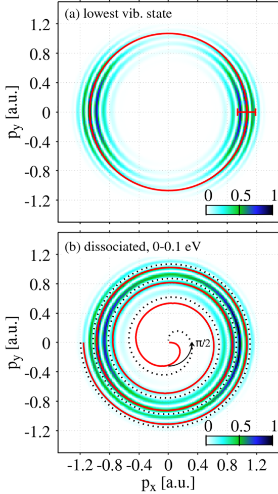
FIG. 1. Photoelectron momentum distributions normalized to a maximum value of 1 for two different energy regions of the nuclei after ionization by an LRCP pulse with a time delay of 12 cycles ( \tau_1 \approx 1.6 fs). (a) Lowest vibrational bound state of \text{H}_2^+ in 1s\sigma_g with energy E_{0,v=0} \approx -0.5975 a.u. The red circle shows the electron momentum p_{\text{el}} \approx 1.07 a.u. according to energy conservation and the red horizontal line is the estimated width \Delta p_{\text{width}} = 0.25 a.u. based on the frequency spectrum of a single pulse. (b) Integrated PMD for an energy region of 0–0.1 eV for dissociated nuclei. The red line represents a spiral arm from the kinematical model (1). The black dotted line is the spiral arm rotated by \pi/2 .
