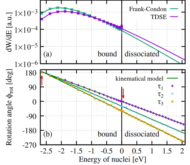
FIG. 2. (a) Vibrational-energy distribution of the molecular ion at the end of the simulations in the \sigma_g state compared to the distribution expected from Franck-Condon factors (arbitrarily scaled for better comparison). (b) Rotation angle of FEVs extracted from the TDSE as a function of vibrational energy in comparison to a kinematical model based on instantaneous energy sharing [Eq. (19)]. At zero energy we find a rotation angle of approximately -0.08^\circ , -30^\circ , and -60^\circ for \tau_1 \approx 1.6 fs, \tau_2 \approx 1.9 fs, and \tau_3 \approx 2.1 fs. Red arrows highlight the positions of the rotation angles of the spirals shown in Fig. 1.
