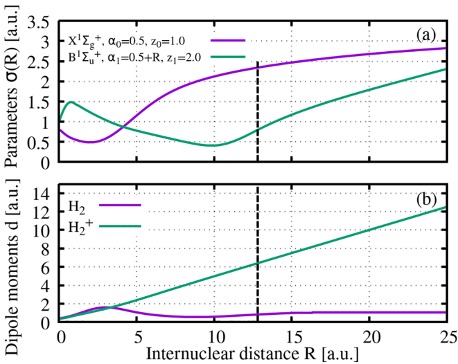
FIG. 7. (a) Optimized parameters \sigma_j(R) for both states of H_2 . (b) Transition dipole moments between the two lowest dipole-allowed electronic states of H_2 and H_2^+ as a function of the internuclear distance, obtained from the literature [68–71].
