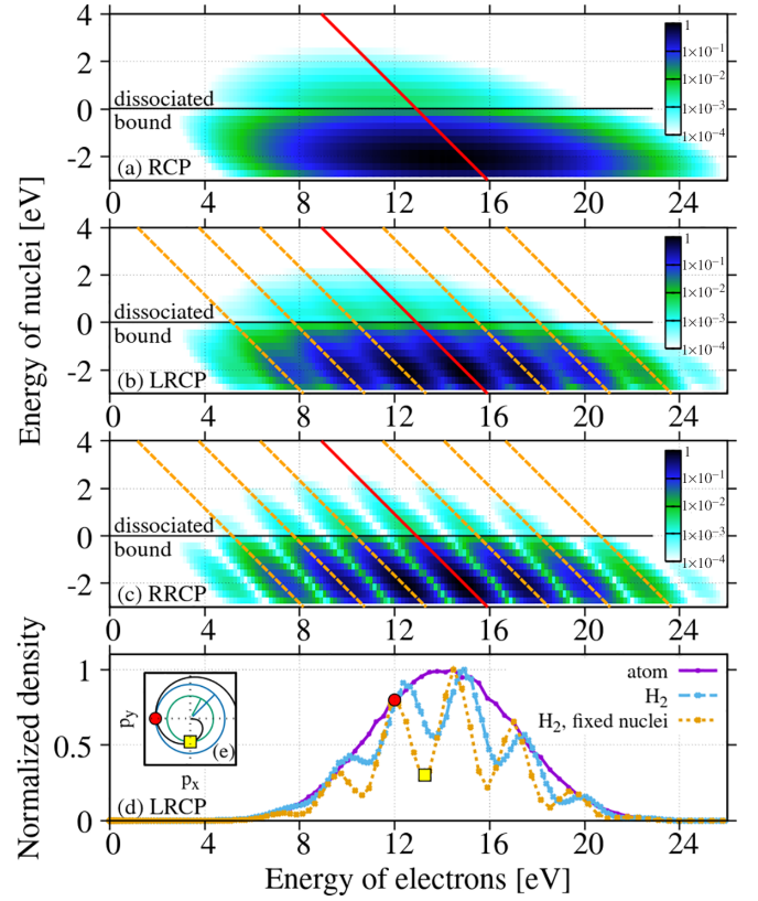
FIG. 5. Normalized joint-energy spectrum of nuclei and photoelectrons for (a) a single RCP pulse, (b) an LRCP, and (c) an RRCP pulse sequence, showing correlation lines (red and orange lines) spaced by \Delta E_{\text{cor}} = \frac{2\pi}{\tau_1} = 2.58 \text{ eV} , which is much smaller than the photon energy ( \hbar\omega \approx 31 \text{ eV} ). (d) Normalized electron-energy spectrum for an LRCP pulse. The magenta solid and orange dotted lines show the spectrum for the atom and the fixed-nuclei molecule with R = 1.4 \text{ a.u.} , respectively. The blue dashed line shows the JES from (b) integrated over the nuclear energy. (e) Illustration of intersections of a spiral with circles of different radii. Yellow and red points mark intersections corresponding to minima and maxima in the electron energy spectrum (see the text for details). All distributions are normalized to the maximal value 1.
