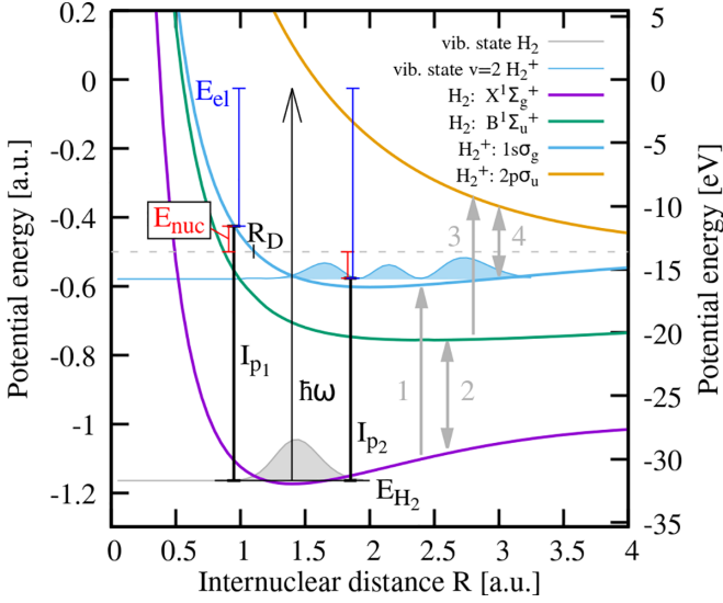
FIG. 6. Energy potential curves of H_2 and H_2^+ used in the model. The large arrow labeled \hbar\omega shows the photon energy. Numbered arrows (1–4) illustrate different mechanisms how population can be transferred between the states: 1 and 3 by removing the active electron |\vec{r}| \rightarrow \infty , and 2 and 4 by population transfer in the two-level system driven by the interaction potential W = -\vec{d}(\vec{r}, R) \cdot \vec{\mathcal{E}}(t) . Vertical lines labeled E_{\text{nuc}} , E_{\text{el}} , I_{p1} = I_p^{\text{vert}}(R = 0.95 \text{ a.u.}) , and I_{p2} = I_p^{\text{adi}}(v = 3) illustrate two examples of the described energy sharing (4) with neglected ponderomotive potential U_p .
