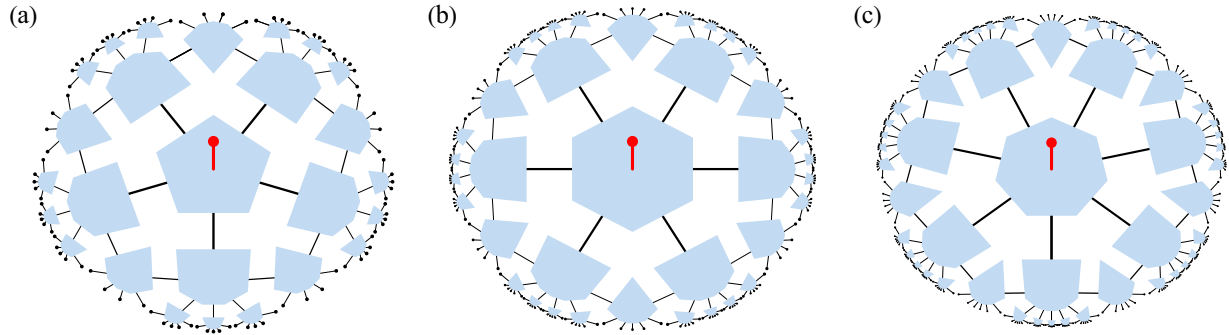
FIG. 1. The holographic tensor-network codes considered in this work: (a) The Harlow-Preskill-Pastawski-Yoshida (HaPPY) code [5] whose pentagon-hexagon geometry also underlies the holographic surface-code fragment (SCF) model [24], (b) the holographic [[6, 1, 3]] code [7], and (c) the holographic Steane code [23]. All are defined as tensor-network contractions of copies of a fixed q -leg tensor on a hyperbolic tiling, with the central tensor used as a seed tensor for the encoding isometry of a [[q - 1, 1, d]] code with some distance d . The remaining tensors have all q legs contracted in the plane, leading to a larger encoding map between one logical qubit (central red leg) and the boundary physical qubits (open black legs). Here we depict the codes with R = 2 layers of edge inflation. In the R \rightarrow \infty limit, the rate of each code goes to zero.
