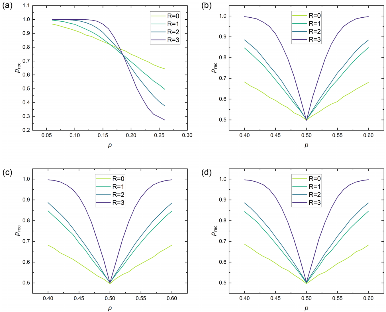
FIG. 4. Threshold curves for depolarizing, pure- X , -Y , and -Z noise, as studied using the tensor-network decoder, for the zero-rate HaPPY code at up to R = 3 layers of edge inflation. Here, p_{\text{rec}} represents the probability for logical qubit recovery, following from [7,9,23].
