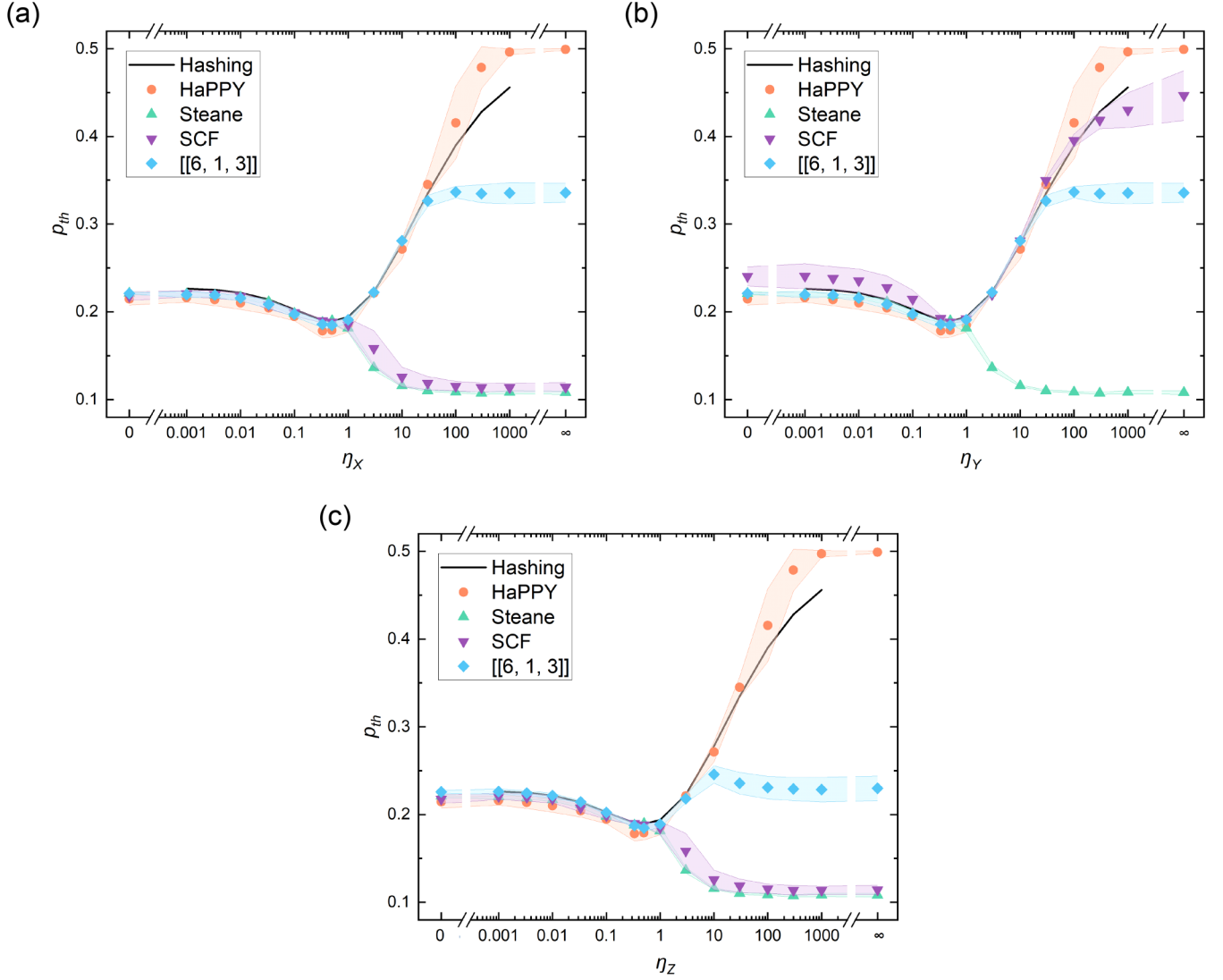
FIG. 5. Hashing bound plots for all of the codes tested in this work; we denote the hashing bound values as a black solid line, while holographic codes are shown in varying colors and markers, together with calculated uncertainties. For all of the plots, the biases range is \eta = \{0, +\infty\} . We list particular points of interest in Table II.
