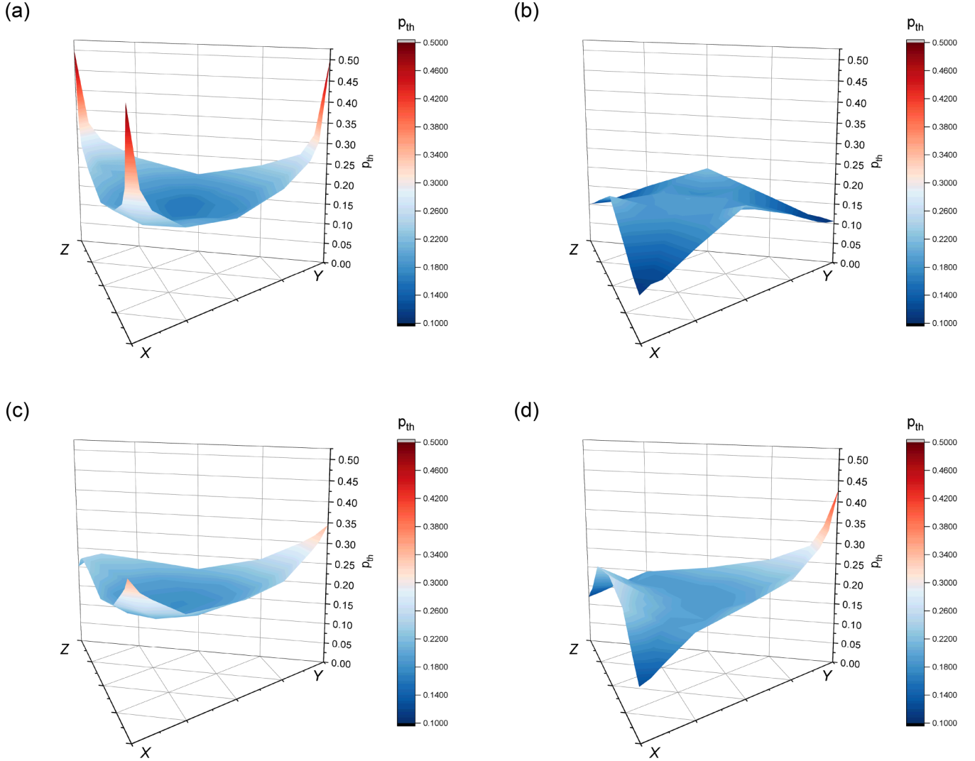
FIG. 3. Ternary plots for all holographic codes investigated in this study under biased noise, in the code-capacity setting. (a)–(d) The zero-rate HaPPY, Steane, [[6, 1, 3]] , and SCF codes; thresholds are color coded from dark blue ( p_{\text{th}} = 10\% ) to dark red ( p_{\text{th}} = 50\% ). Additionally, we tested the tailored [[7, 1, 3]] code from [14,22], which achieved an identical threshold profile to that of the HaPPY code.
