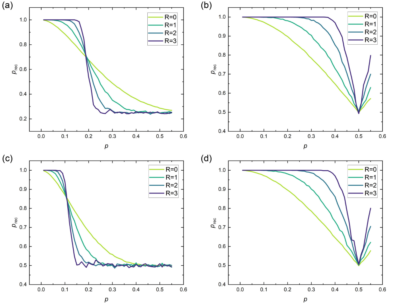
FIG. 6. Threshold curves for the Clifford-deformed Steane code that we mention in Sec. IV. Here, we have applied hadamard gates to physical qubits 2, 3, 5, and 6. In (a), we document a slight threshold increase to 19.0 \pm 0.33\% . (b),(d) The thresholds under pure- X and -Z noise, respectively, under which an increase to approximately 50% can be observed. (c) The results for pure- Y noise, with an apparent slight decrease to 10.58 \pm 0.12\% . As in Fig. 4, p_{\text{rec}} represents the probability for logical qubit recovery, hailing from [7,9,23].
