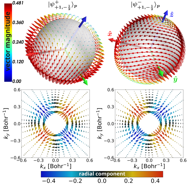
FIG. 2. The momentum-resolved propensity field \vec{B}_k [Eq. (34)] in k space for the chiral state |\psi_{1,-\frac{1}{2}}^\pm\rangle_p . The spheres correspond to \vec{B}_k with |\vec{k}| = 0.525 bohr ^{-1} where the vectors are colored as |\vec{B}_k| . The two-dimensional vector fields represent an equatorial cut in the k_x - k_y plane and colored according to its radial component ( \hat{k} \cdot \vec{B}_k ). It can be seen that the propensity field for opposite enantiomers R and S are related via inversion \vec{B}_k^{(R)} = \vec{B}_{-\vec{k}}^{(S)} .
