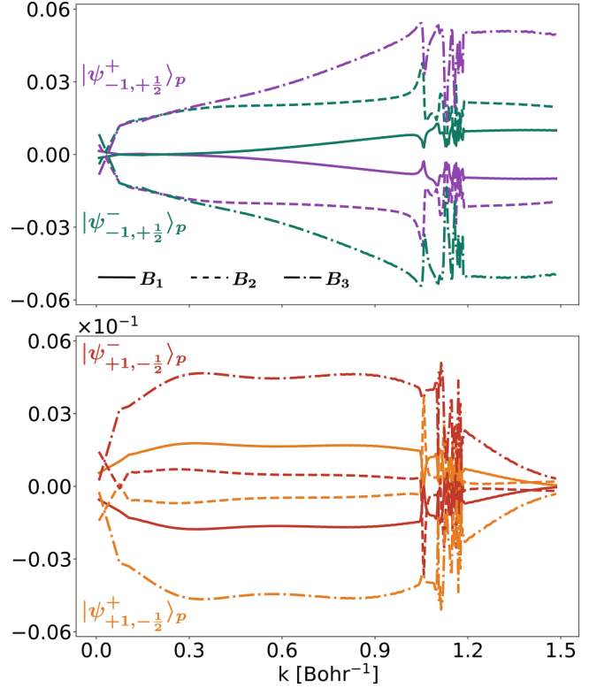
FIG. 8. The coefficient B_1 (solid line), B_2 (dashed line), and B_3 (dotted-dashed line) for the chiral states |\psi_{\pm 1, \pm \frac{1}{2}}^{\pm}\rangle_p and |\psi_{\pm 1, \mp \frac{1}{2}}^{\pm}\rangle_p .
