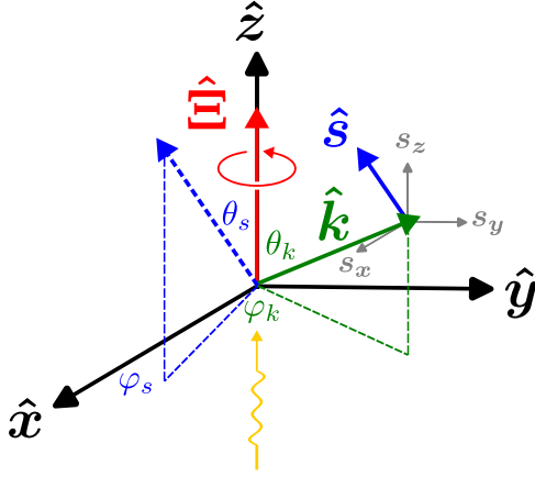
FIG. 1. Specification of coordinates in the laboratory frame. The light field propagates along \hat{z} . The unit vector \hat{\mathbf{E}} = \xi \hat{z} (solid red) is the direction of photon spin, where \xi = \pm 1 is a dichroic parameter characterizing the direction of rotation of the light polarization vector. Upon ionization, the photoelectron is ejected in the direction of \hat{\mathbf{k}} (solid green) with its spin measured parallel to \hat{\mathbf{s}} (solid blue). The expansion W^L(\hat{\mathbf{k}}^L, \hat{\mathbf{s}}^L) [Eq. (11a)] is represented by the solid green and dashed blue vectors.
