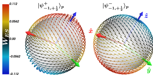
FIG. 10. Spin texture that maximizes the enantio-sensitive part of the yield W(\hat{\mathbf{k}}^L, \hat{\mathbf{s}}^L) for the chiral states |\psi_{-1,\frac{1}{2}}^{\pm}\rangle_p at k = 1.055 \text{ bohr}^{-1} . The arrows are colored according to the enantio-sensitive component of the yield W_{\text{ES}} .
