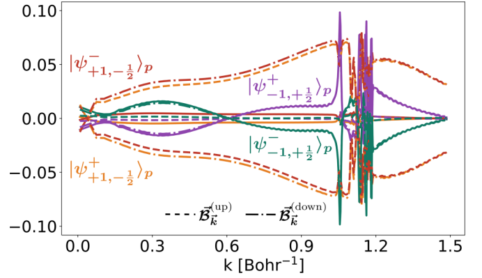
FIG. 3. The coefficient D (solid line) as well as the contributions of the spin up (dashed line) and spin down (dotted-dashed line) [Eq. (34)] for the chiral states |\psi_{1,-\frac{1}{2}}^\pm\rangle_p . The rapidly oscillating behavior of D at higher values of k is due to the Fano resonances, leading up to the ionization threshold for the 3s electrons [44,45].
