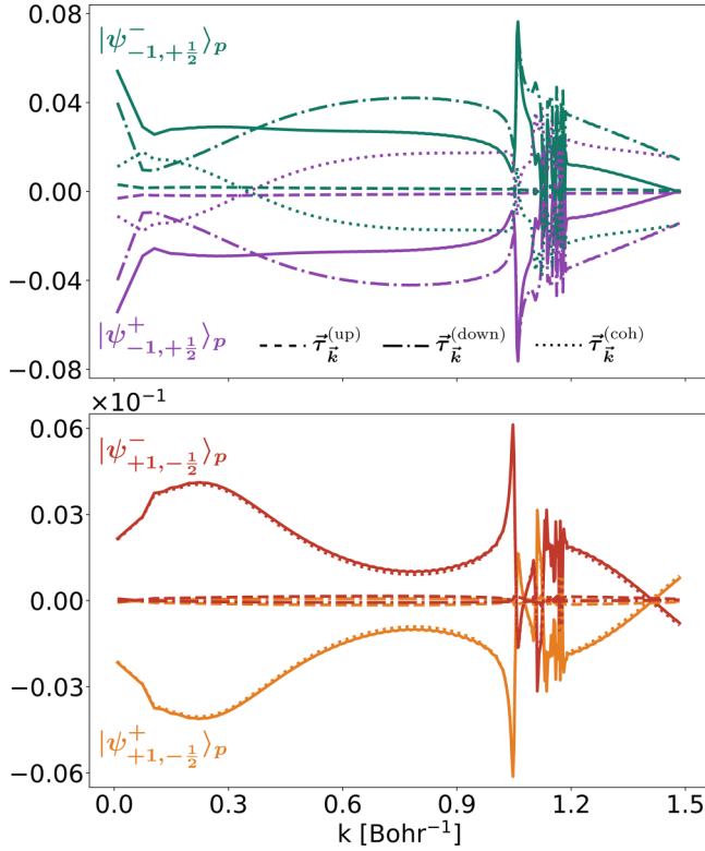
FIG. 5. The coefficient C (solid line) as well as the contributions of the spin up (dashed line) and spin down (dotted-dashed line) [Eq. (34)] for the chiral states |\psi_{1,-\frac{1}{2}}^{\pm}\rangle_p and |\psi_{-1,\frac{1}{2}}^{\pm}\rangle_p .
