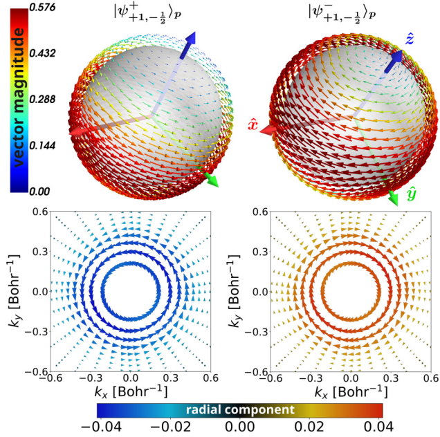
FIG. 7. The momentum-resolved Bloch pseudovector \vec{S}_{\vec{k}} in k space for the chiral state |\psi_{\pm 1, -\frac{1}{2}}^{\pm}\rangle_p . The spheres correspond to \vec{S}_{\vec{k}} with |\vec{k}| = 0.525 bohr ^{-1} where the vectors are colored as |\vec{S}_{\vec{k}}| . The two-dimensional vector fields represent an equatorial cut in the k_x - k_y plane and colored according to their radial component ( \hat{k} \cdot \vec{S}_{\vec{k}} ). It can be seen that the Bloch pseudovector field for opposite enantiomers R and S is related via inversion \vec{S}_{\vec{k}}^{(R)} = \vec{S}_{-\vec{k}}^{(S)} .
