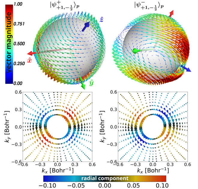
FIG. 4. The momentum-resolved spin torque field \vec{\tau}_k [Eq. (35)] in k space for the chiral state |\psi_{1,-\frac{1}{2}}^\pm\rangle_p . The spheres correspond to \vec{\tau}_k with |\vec{k}| = 0.525 bohr ^{-1} where the vectors are colored as |\vec{\tau}_k| . The two-dimensional vector fields represent an equatorial cut in the k_x - k_y plane and colored according to its radial component ( \hat{k} \cdot \vec{\tau}_k ). It can be seen that the spin torque field for opposite enantiomers R and S is related via inversion \vec{\tau}_k^{(R)} = \vec{\tau}_{-\vec{k}}^{(S)} .
