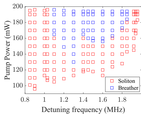
FIG. 4. Experimental measurements. Stable region in the pump power–detuning parameter space for single solitons and breather solitons in detuning and power space.
