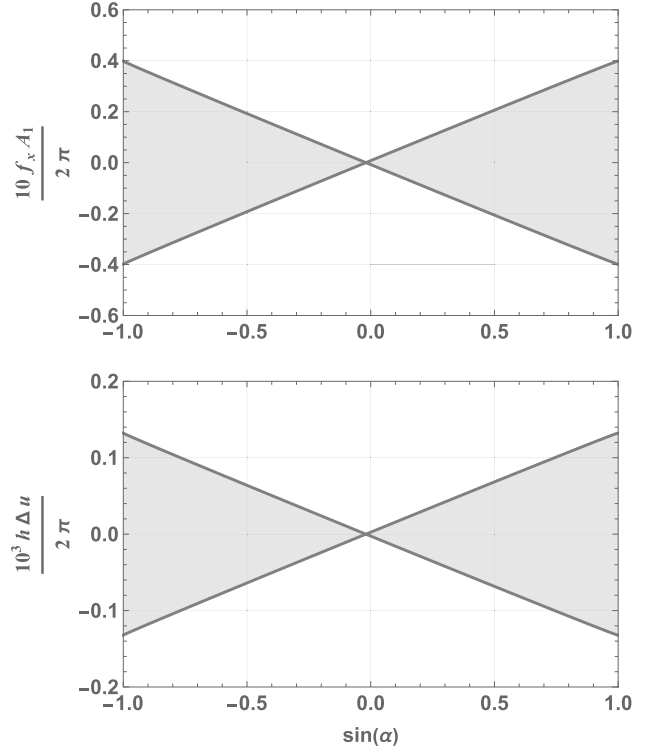
FIG. 2. Distribution (gray area) of the \mathcal{A}_1 f_x (top) and h\Delta u (bottom) phase excesses (defects). They form a bundle of nearly straight lines. The interferometer parameters and 2- \mu\text{m} geometry tolerances are from [6] (see Table I). The detector distance from the interferometer is 0.5 m. The defocus is uniformly distributed in the [-6, +6] \mu\text{m} interval.
