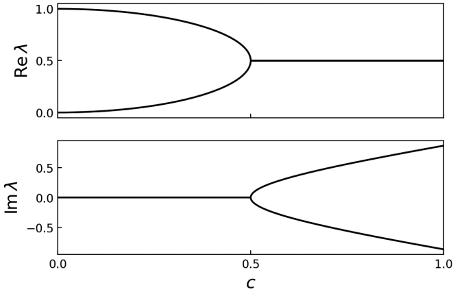
FIG. 1. Eigenvalues of Eq. (1), where a = 0 , b = ic , and d = 1 , varied against parameter c , taking a value of c = \frac{1}{2} at an EP.
