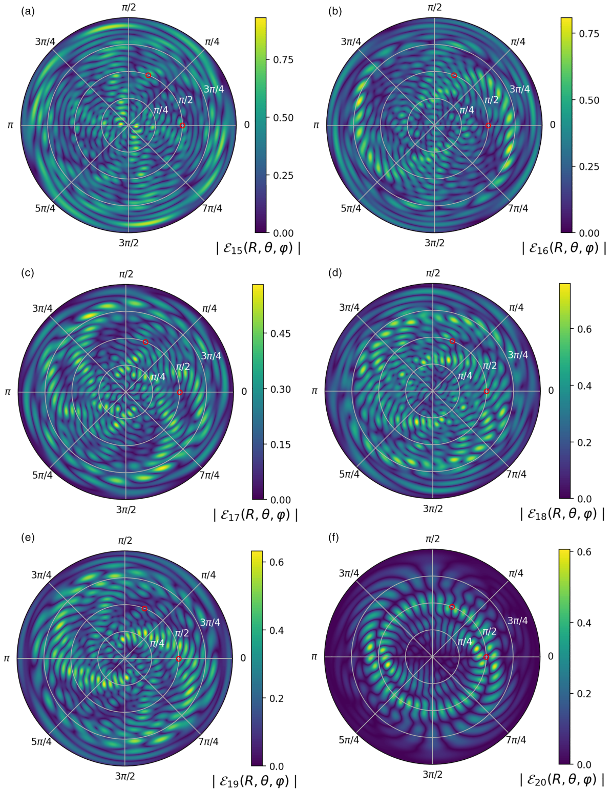
FIG. 13. As Fig. 9(a) but with (a), (b), (c), (d), (e), and (f) showing the wave functions of states v = 15, 16, 17, 18, 19, and 20 , respectively.
