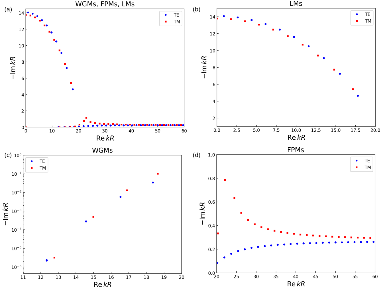
FIG. 3. Wave numbers of the TE (blue circles) and TM (red squares) 2l + 1 degenerate modes of a homogeneous dielectric sphere with refractive index n_r = 2 , surrounded by vacuum, for angular momentum number l = 20 . (a) All types of optical modes, (b) LMs, (c) WGMs (using a \log_{10} scale for the imaginary part), and (d) FPMs. Reproduction of Fig. 1 in [49].
