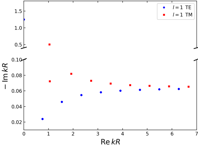
FIG. 2. Wave numbers of the TE (blue circles) and TM (red squares) 2l + 1 degenerate modes of a homogeneous dielectric sphere with refractive index n_r = 4 , surrounded by vacuum, for angular momentum number l = 1 .
