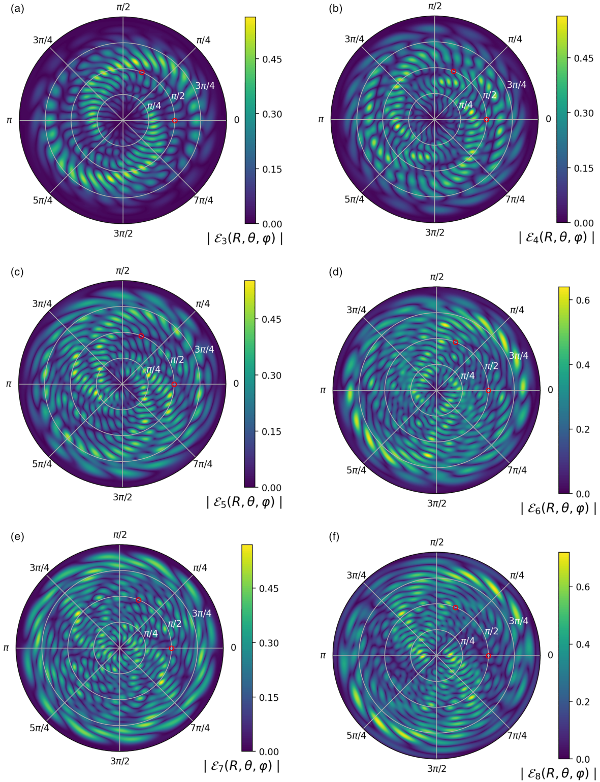
FIG. 11. As Fig. 9(a) but with (a), (b), (c), (d), (e), and (f) showing the wave functions of states \nu = 3, 4, 5, 6, 7 , and 8 , respectively.
