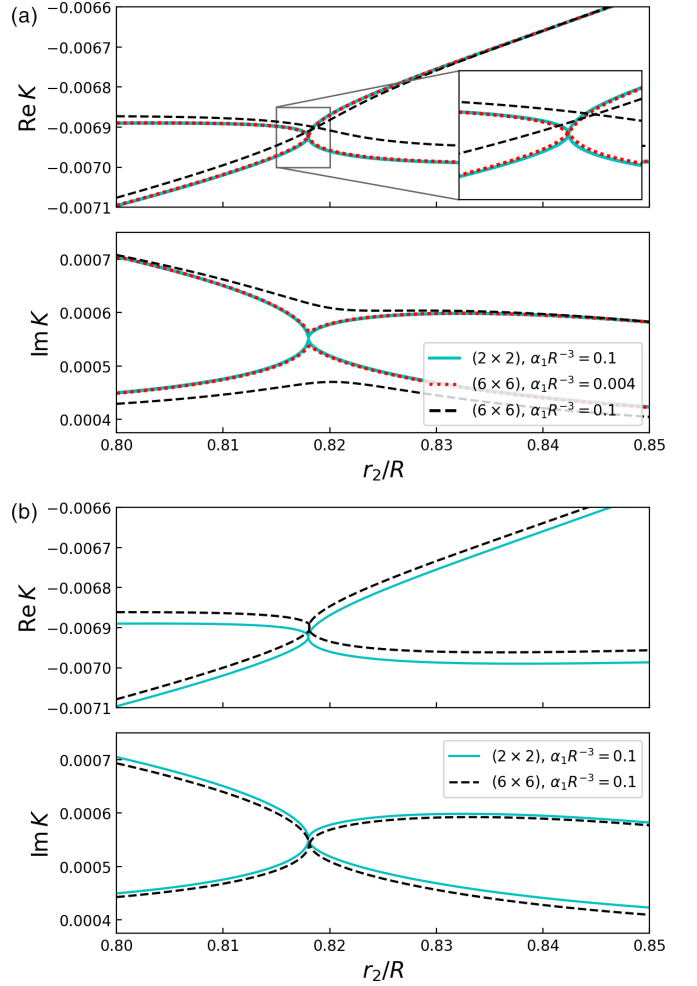
FIG. 5. Dimensionless wave numbers K of perturbed RSs calculated from H_{nn'} , with l = 1 , against r_2/R , for a microsphere with n_r = 4 and two perturbors. (a) For the cyan solid lines, H_{nn'} has the mode basis of a triply degenerate TE WGM only accounting for m = \pm 1 . For the red dotted and black dashed lines, H_{nn'} has the mode basis of a triply degenerate TE WGM and its closest triply degenerate TM FPM, both triplets with m = 0, \pm 1 . Red dotted (black dashed) lines have perturber strengths \alpha_1 R^{-3} = 0.004 and \alpha_2 R^{-3} = 0.003107 ( \alpha_1 R^{-3} = 0.1 and \alpha_2 R^{-3} = 0.0777 ). Cyan solid lines are the K values of the 2 \times 2 matrix which are equal for either factor of perturber strength, to first order. Other perturbation parameters are fixed at r_1/R = 0.95 and \Delta\varphi = 1.547 . (b) As the cyan solid lines and black dashed lines in (a) but with the 6 \times 6 matrix including the l = 1 TM mode (black dashed lines) fine tuned to restore the EP by changing the angle between perturbors to \Delta\varphi = 1.5494 .
