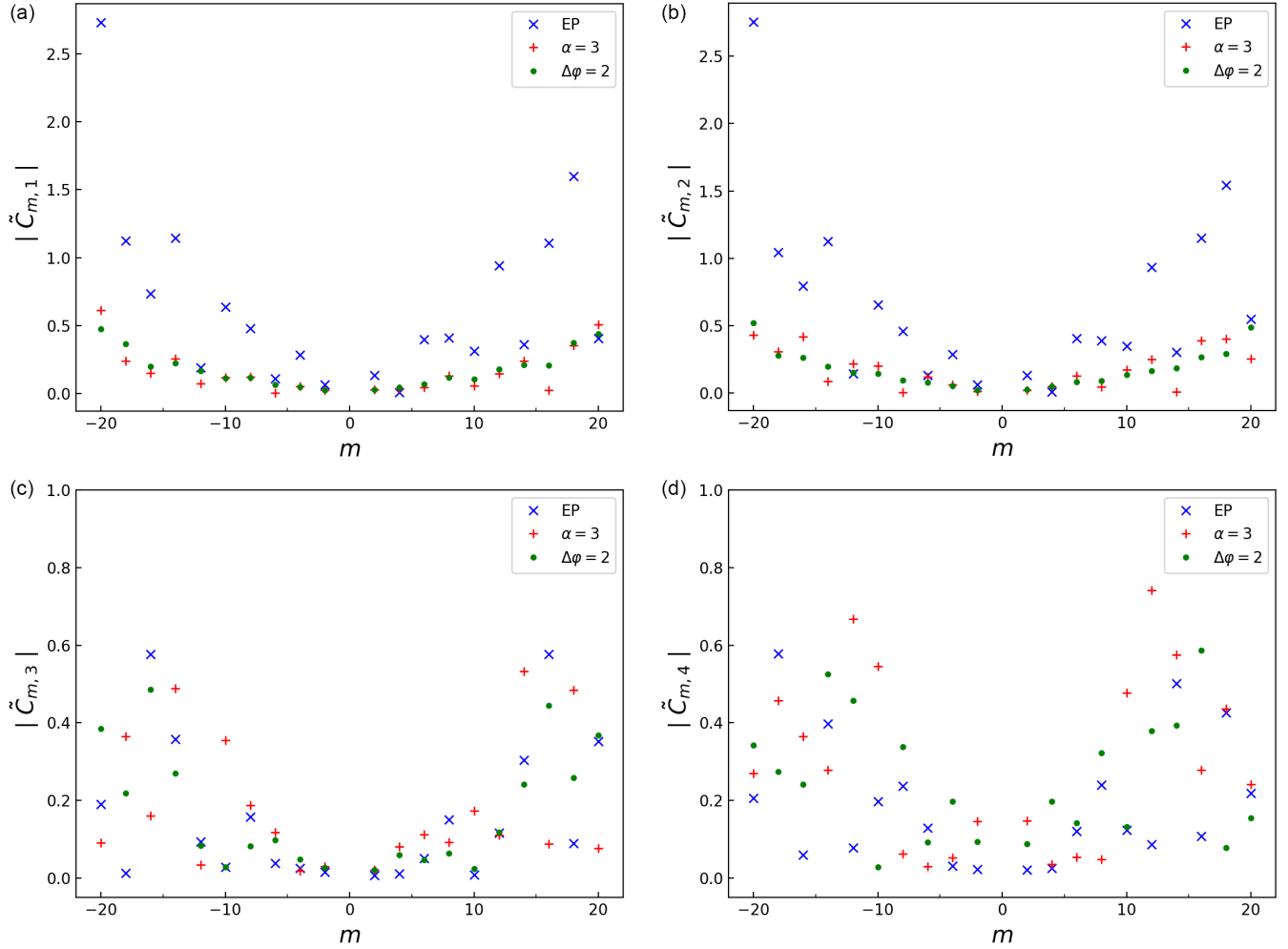
FIG. 10. Modulus of RSE expansion coefficients \tilde{C}_{mv} , for l = 20 , n_r = 2 , and two perturbors, against m . Blue crosses show eigenstates at the given parameters of the EP, which are \alpha = 1.6 , \Delta\varphi = 1.199\,605 , r_1/R = 1.5 , and r_2/R = 1.554\,20 , red pluses show eigenstates with the perturber strength ratio changed to \alpha = 3 , and green dots show eigenstates with the angle between the perturbors changed to \Delta\varphi = 2 . (a)–(d) Show the expansion coefficients for states v = 1, 2, 3 , and 4 , respectively.
