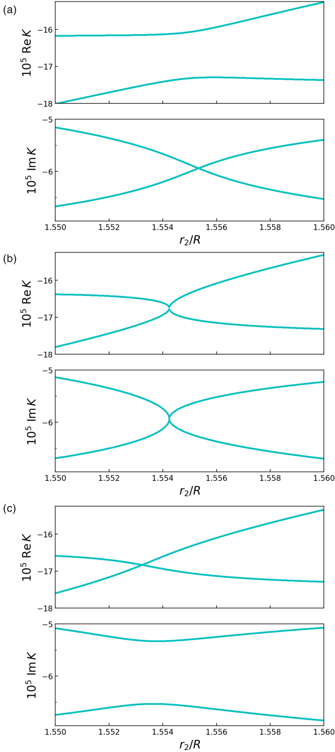
FIG. 8. As Fig. 7 but for a 20 \times 20 matrix only, varying r_2 , and fixing \alpha = 1.6 , r_1/R = 1.5 , and \Delta\varphi , with (a) \Delta\varphi = 1.200\,605 (strong coupling), (b) \Delta\varphi = 1.199\,605 (EP), and (c) \Delta\varphi = 1.198\,605 (weak coupling). The actual values of K are obtained by multiplying the shown numbers by 10^{-5} as indicated.
