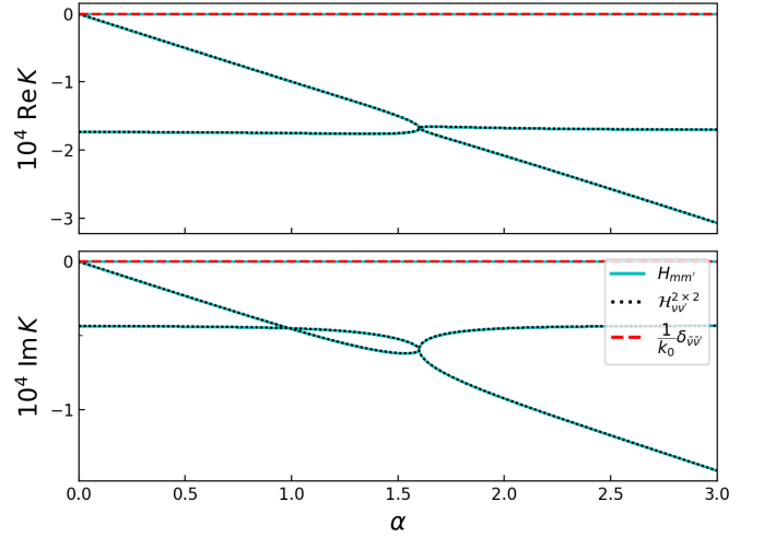
FIG. 7. Scaled dimensionless wave numbers K around an EP for a microsphere with refractive index n_r = 2 , angular momentum l = 20 , and two perturbors, calculated using a 20 \times 20 matrix H_{mm'} (cyan solid lines), 2 \times 2 matrix H_{vv'}^{2 \times 2} (black dotted lines), and the diagonal 18 \times 18 matrix k_0^{-1} \delta_{vv'} (red dashed lines) against the perturber strength ratio \alpha , with \sigma' = \alpha' = 10 used for the orthogonal transformation. The other parameters are fixed at r_1/R = 1.5 , r_2/R = 1.5542 , and \Delta\varphi = 1.199\,605 . The actual values of K are obtained by multiplying the shown numbers by 10^{-4} as indicated.
