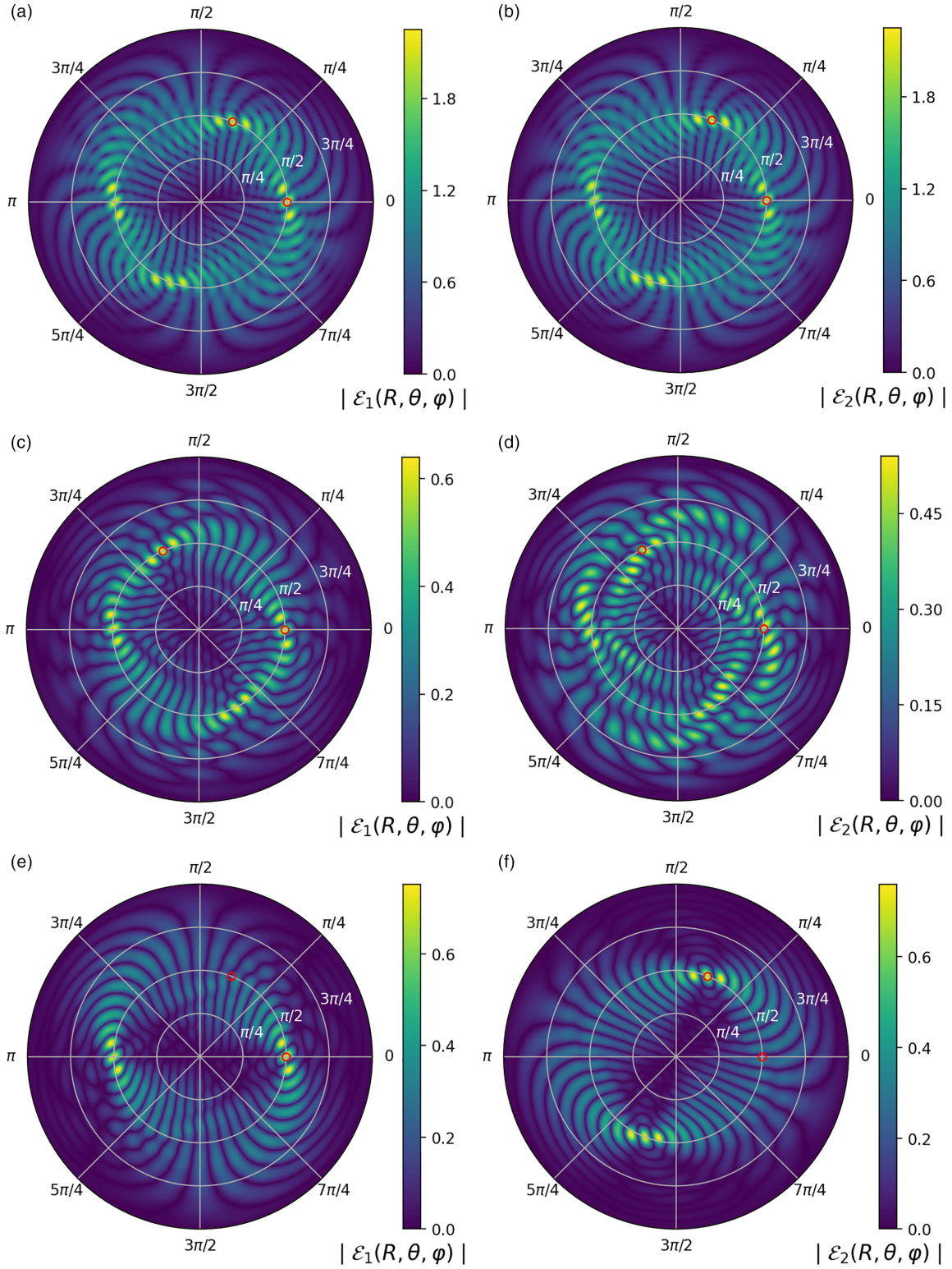
FIG. 9. Modulus of perturbed l = 20 electric fields at the sphere surface as a function of azimuthal and polar angles for \nu = 1 (left panels) and \nu = 2 (right panels). \theta is shown by the radial axis and \varphi by the polar angle. Brighter colors represent a stronger field. Red hollow circles show the angular position of the perturbers. (a), (b) show the wave functions at the EP with \Delta\varphi = 1.199\,605 and \alpha = 1.6 . (c), (d) show the wave functions away from the EP for \Delta\varphi = 2 and \alpha = 1.6 . (e), (f) show the wave functions away from the EP for \Delta\varphi = 1.199\,605 and \alpha = 3 . The perturber radii are r_1/R = 1.5 and r_2/R = 1.554\,20 for all panels.
