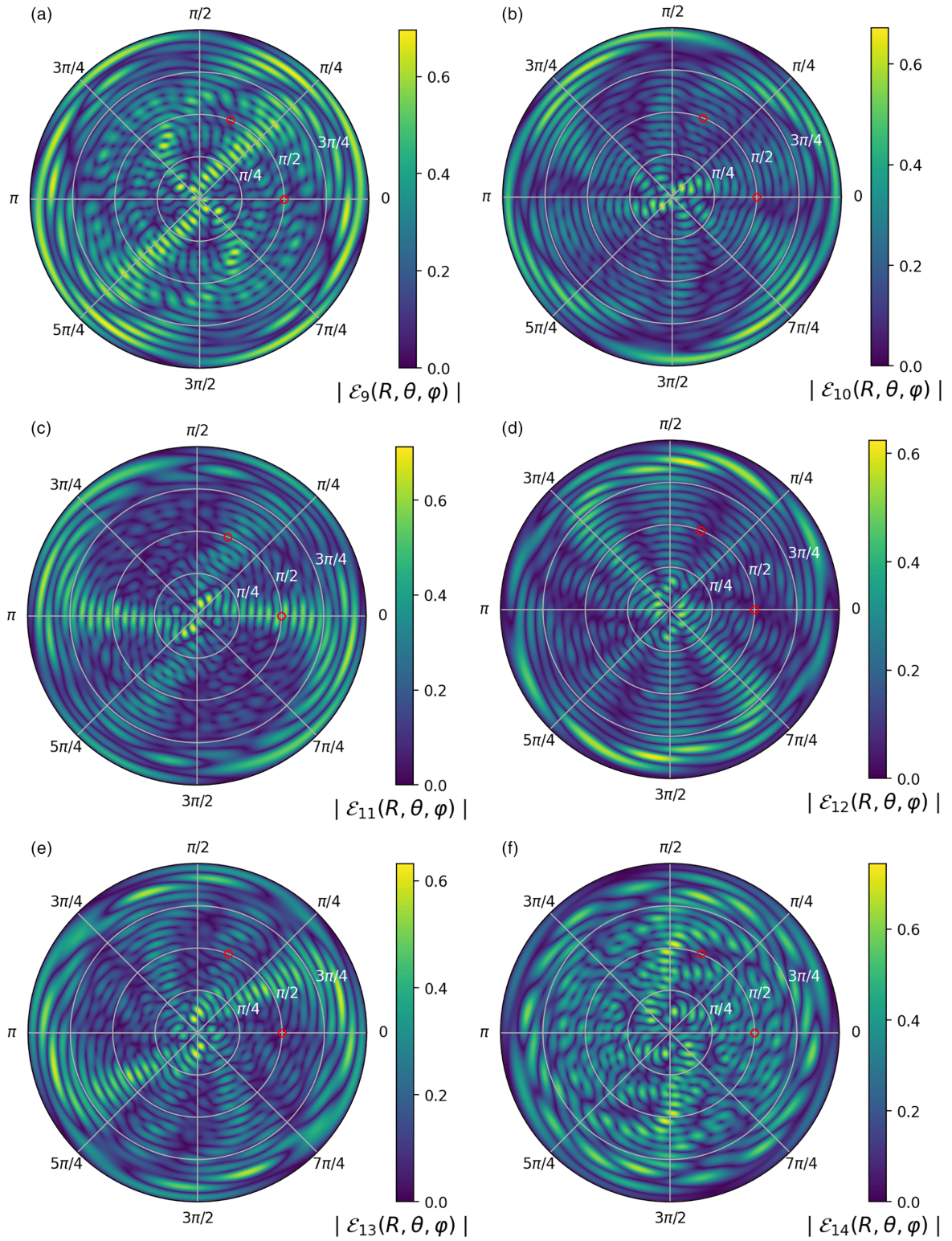
FIG. 12. As Fig. 9(a) but with (a), (b), (c), (d), (e), and (f) showing the wave functions of states \nu = 9, 10, 11, 12, 13 , and 14 , respectively.
