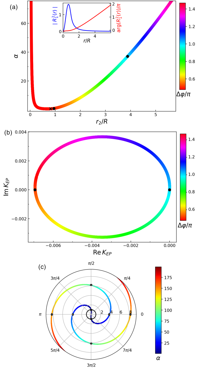
FIG. 4. Solutions of Eq. (22), the condition where the eigenvalues of H_{mn'} (with an m = \pm 1 two-mode TE basis of the fundamental WGM in Fig. 2) are degenerate, in the parameter space of the system (dielectric microsphere with n_r = 4 , surrounded by vacuum, with two perturbers). Black dots denote the parameters of DPs. The radial position of the first perturber is fixed at r_1/R = 0.95 . (a) Parameters satisfying Eq. (22): \alpha , r_2/R , and \Delta\varphi/\pi with the latter represented by color shown in the range \Delta\varphi/\pi = 0.477 to \Delta\varphi/\pi = 1.477 . Inset plots the modulus of the squared radial function |\mathcal{R}_1^2(r)| in the left axis and its phase \arg \mathcal{R}_1^2(r)/\pi in the right axis against radial position. Black cross denotes the parameters of the EP shown in Fig. 5. (b) K_{EP} for the same degeneracies as (a) with color representing the same range of \Delta\varphi/\pi . (c) Positions of the second perturber r_2/R and \varphi_2 = \Delta\varphi that lead to EPs in polar coordinates (with \varphi_1 = 0 and \theta_1 = \theta_2 = \pi/2 ) with the corresponding \alpha shown by color. Black thick hollow circle shows the surface at r = R of the microsphere.
